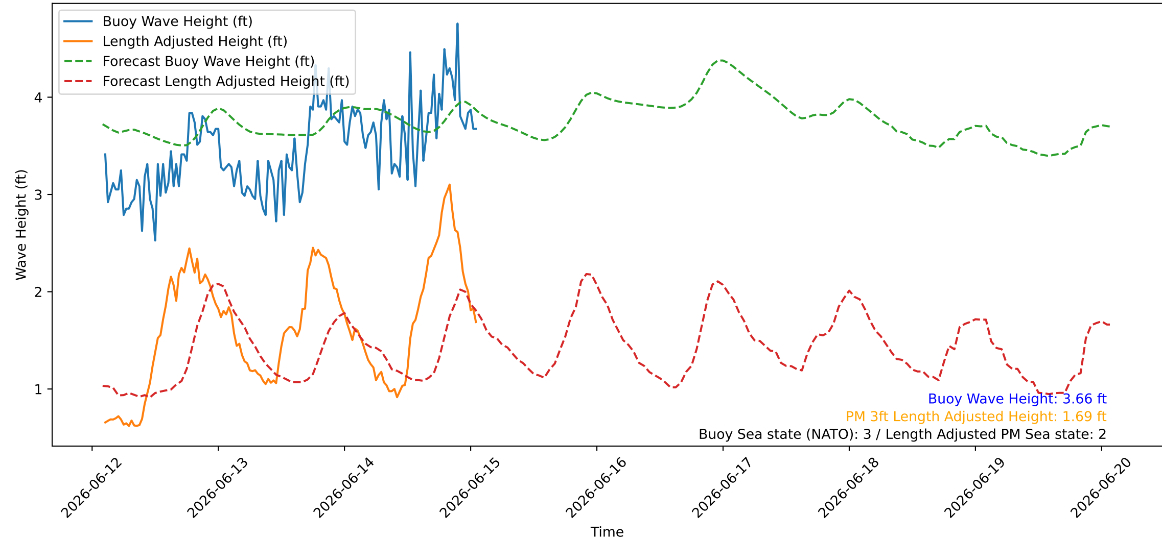
Wave Heights over Time for Red Beach at 2026-06-15 02:00:45
