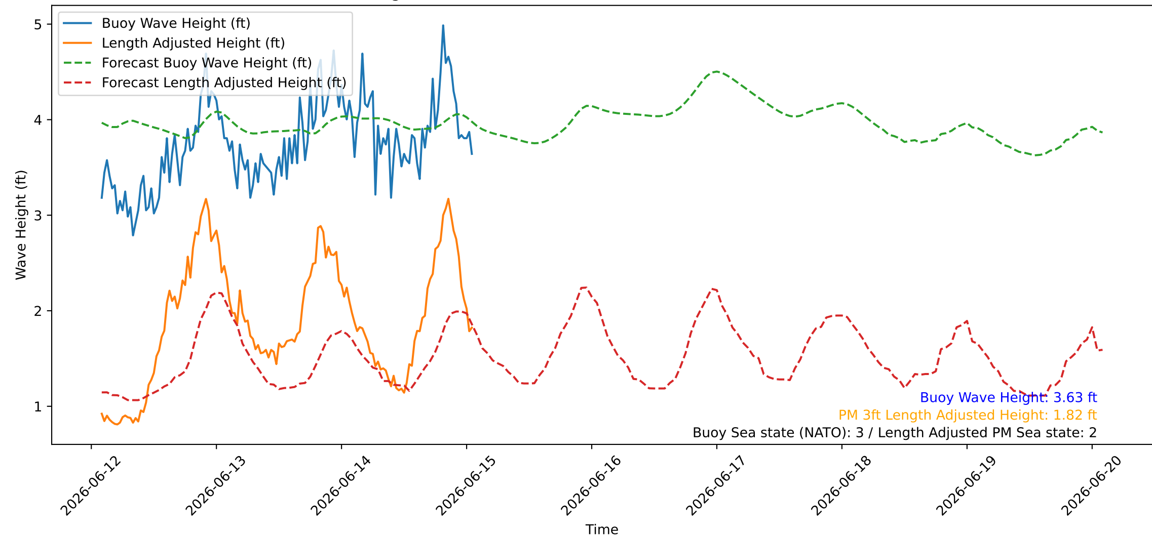
Wave Heights over Time for Oceanside Harbor at 2026-06-15 02:00:26
