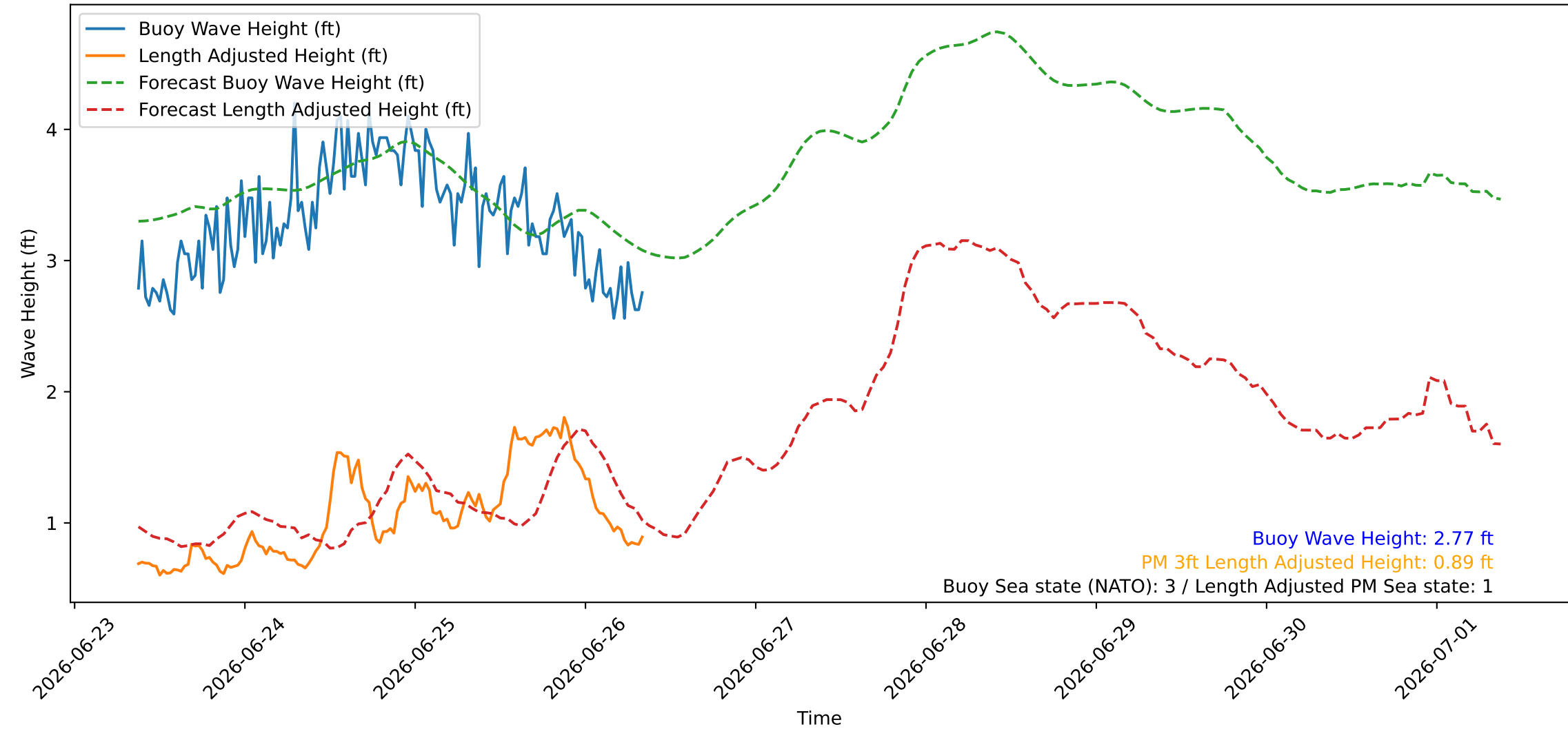
Wave Heights over Time for Green Beach at 2026-06-26 09:01:08
