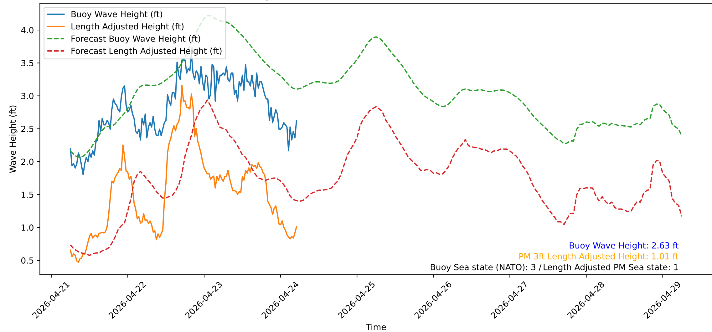
Wave Heights over Time for Red Beach at 2026-04-24 05:40:50
