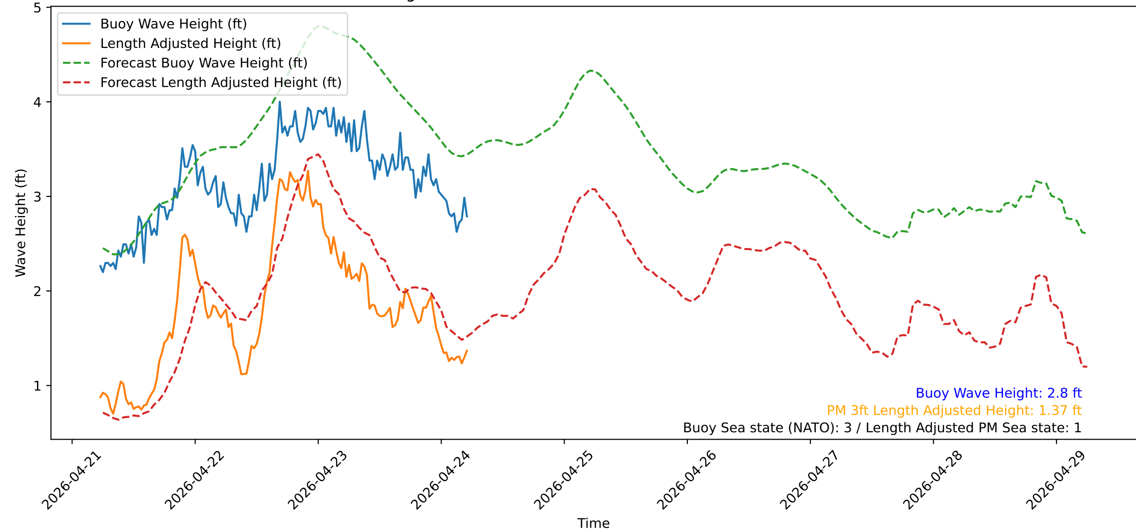
Wave Heights over Time for Green Beach at 2026-04-24 05:41:12
