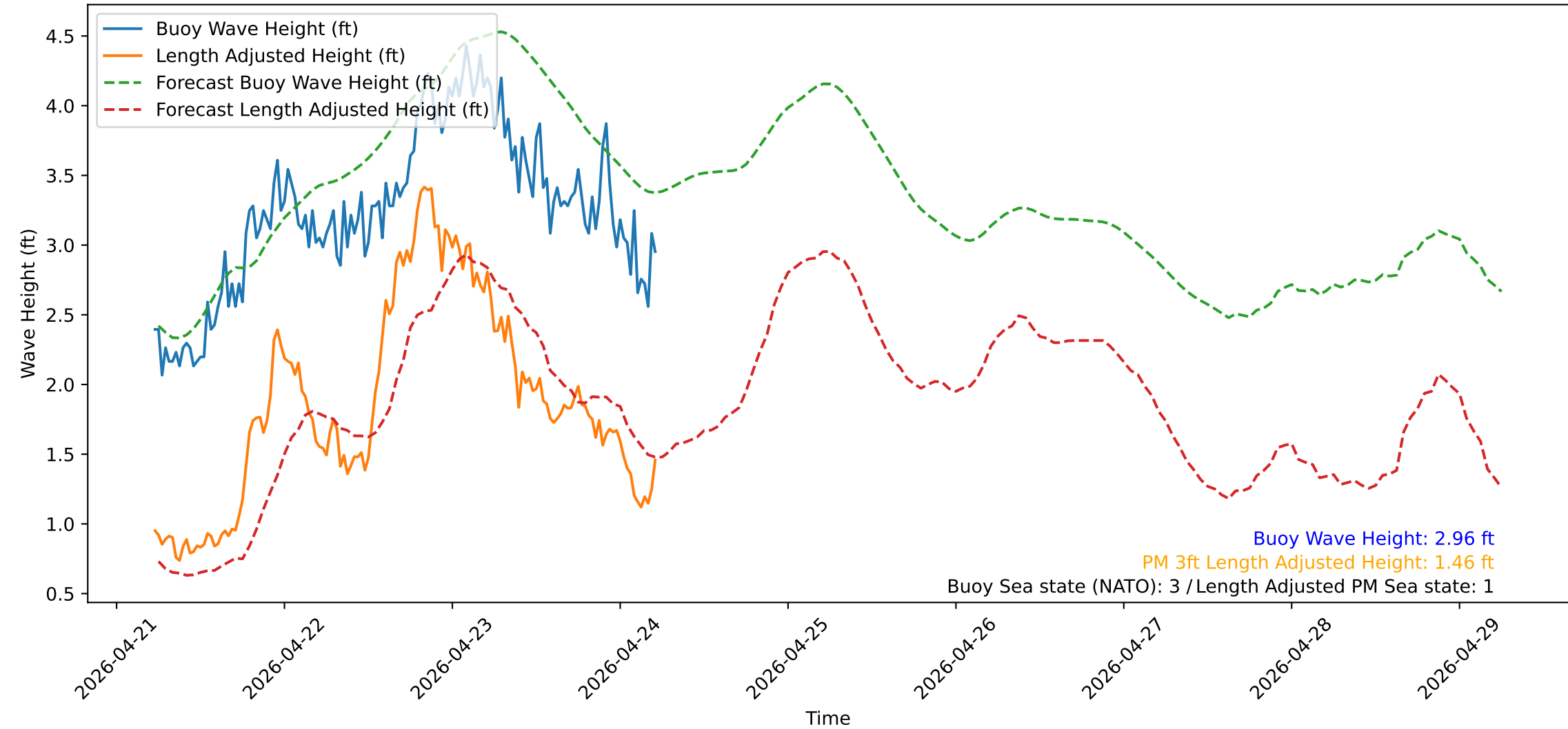
Wave Heights over Time for Oceanside Harbor at 2026-04-24 05:40:30
