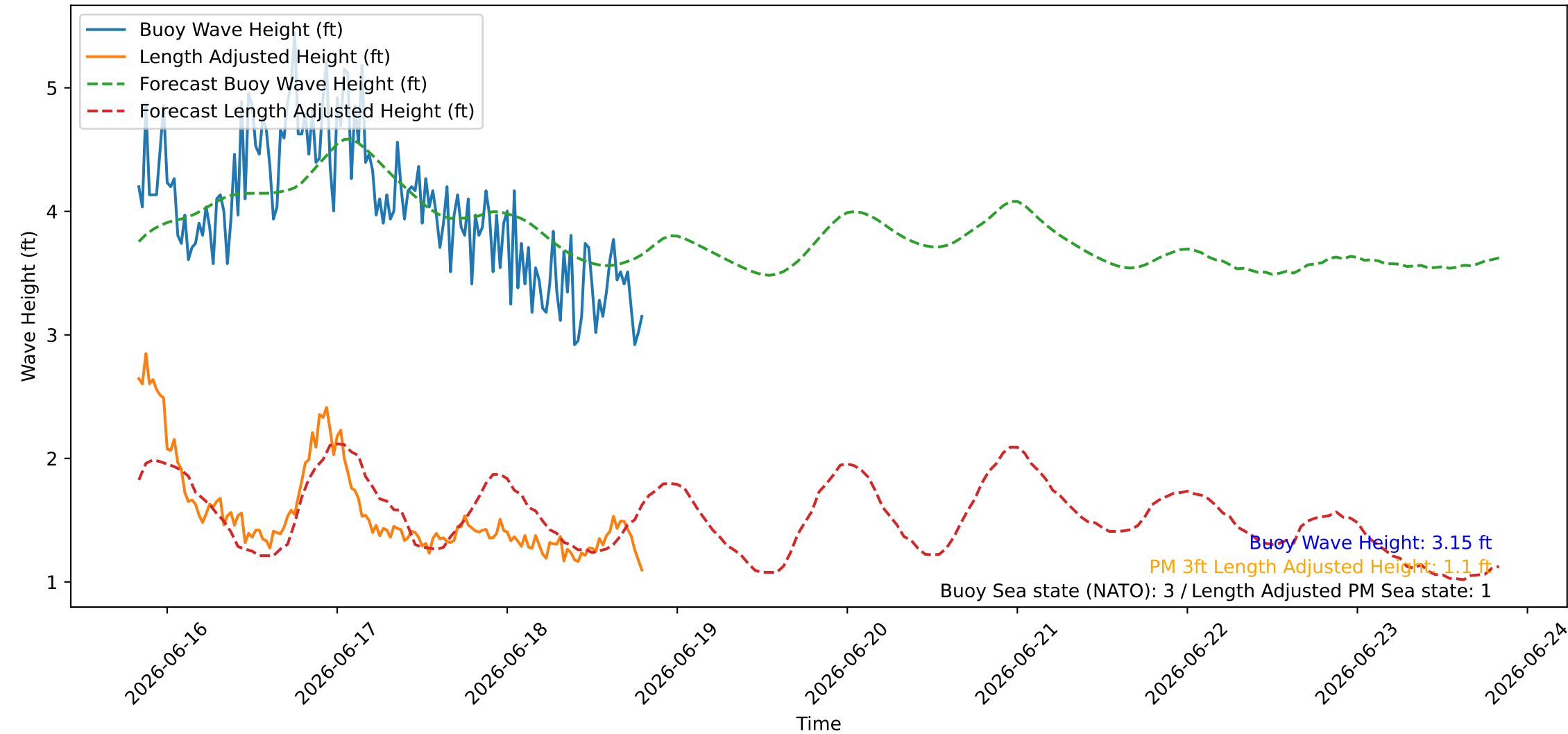
Wave Heights over Time for Oceanside Harbor at 2026-06-18 19:50:26
