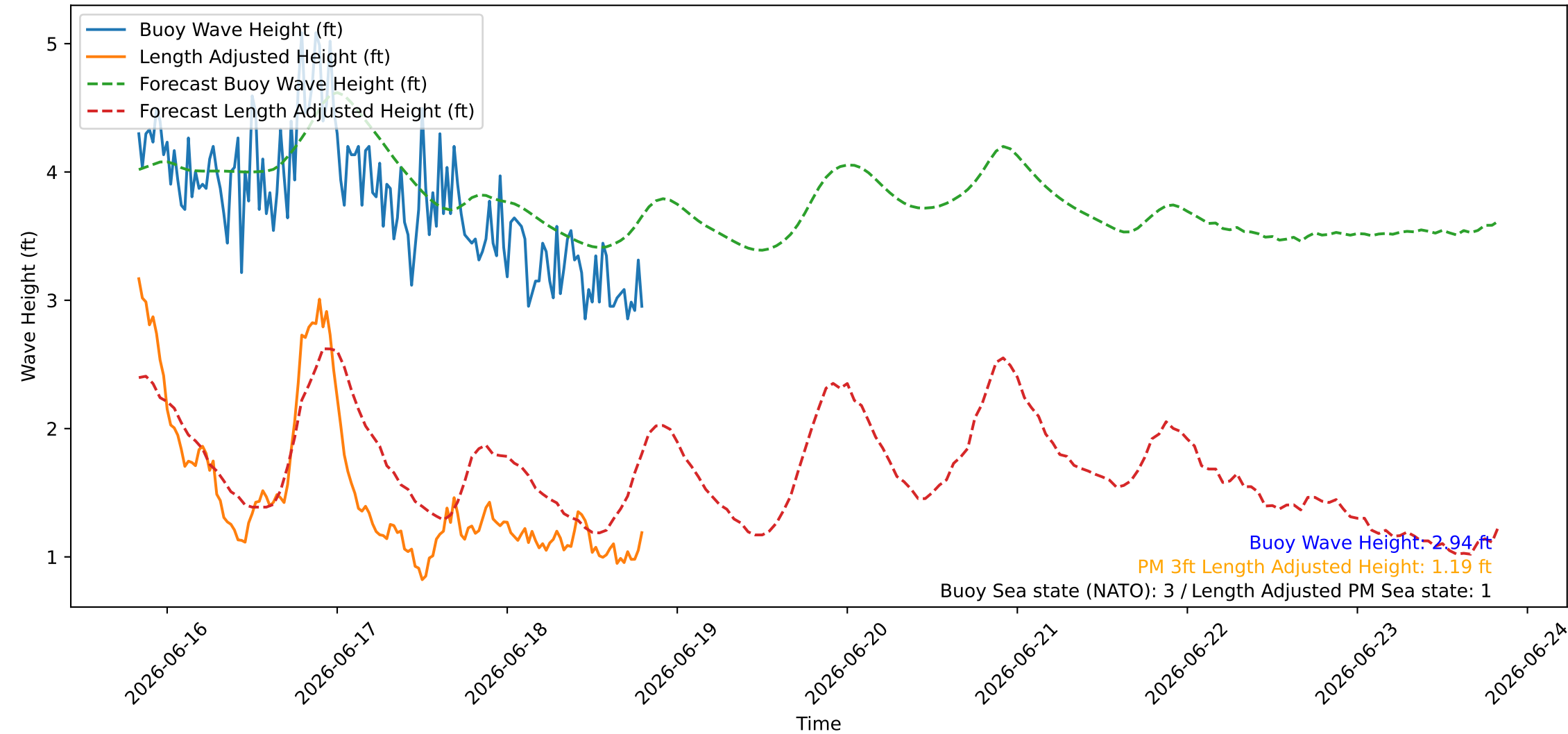
Wave Heights over Time for Green Beach at 2026-06-18 19:51:08
