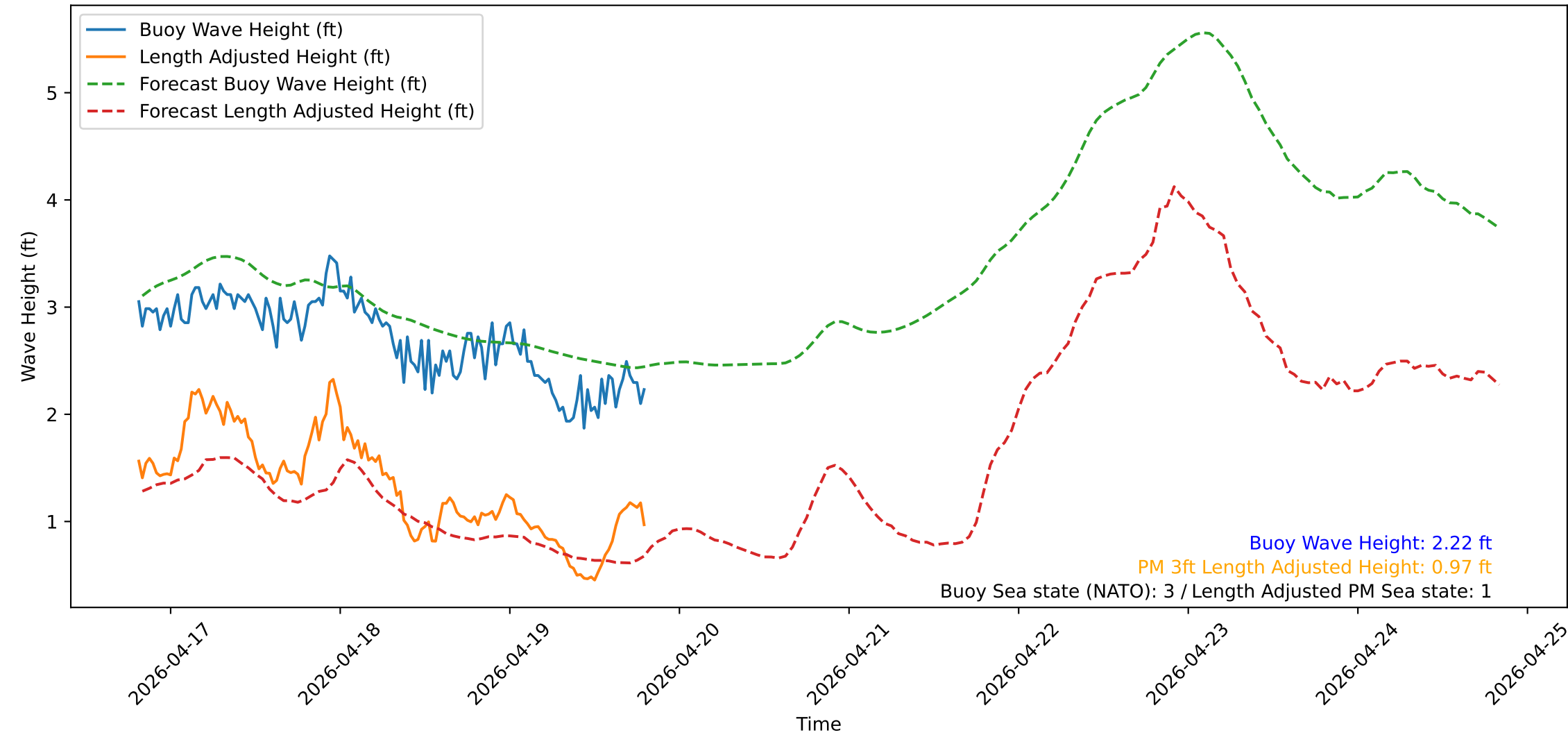
Wave Heights over Time for Green Beach at 2026-04-19 19:41:12
