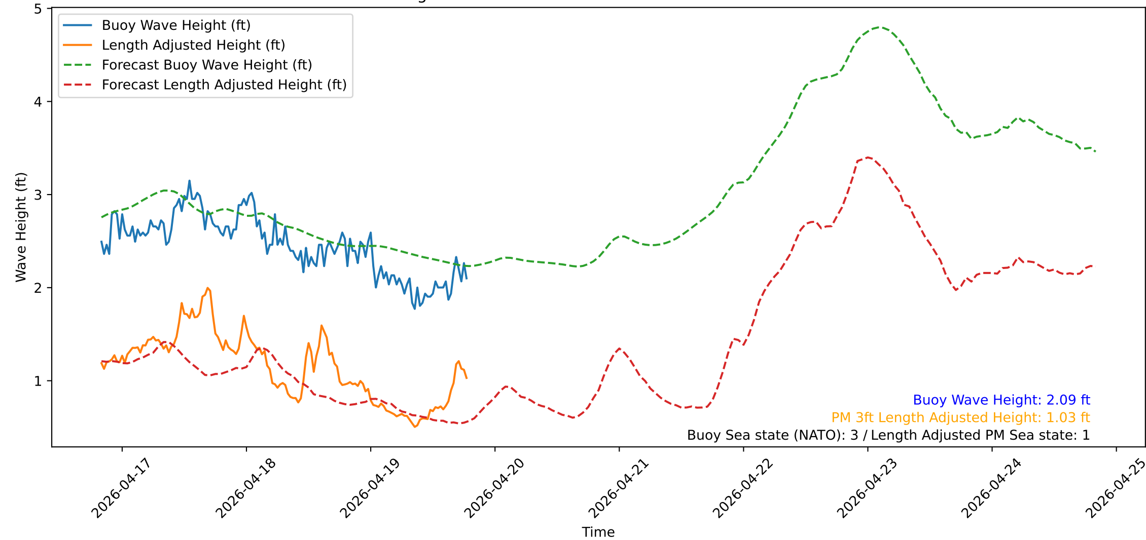
Wave Heights over Time for Red Beach at 2026-04-19 19:40:50
