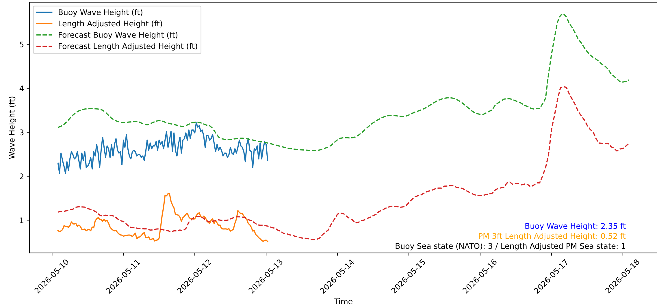
Wave Heights over Time for Red Beach at 2026-05-13 01:30:51
