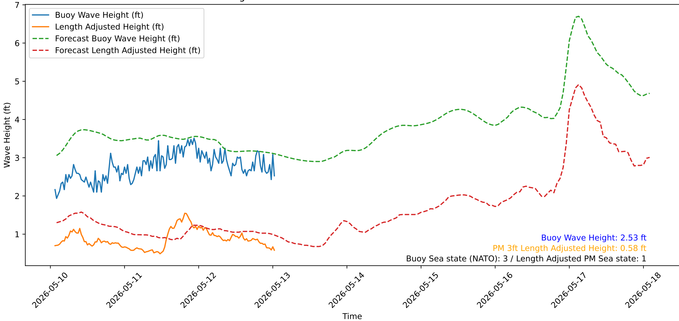
Wave Heights over Time for Green Beach at 2026-05-13 01:31:13
