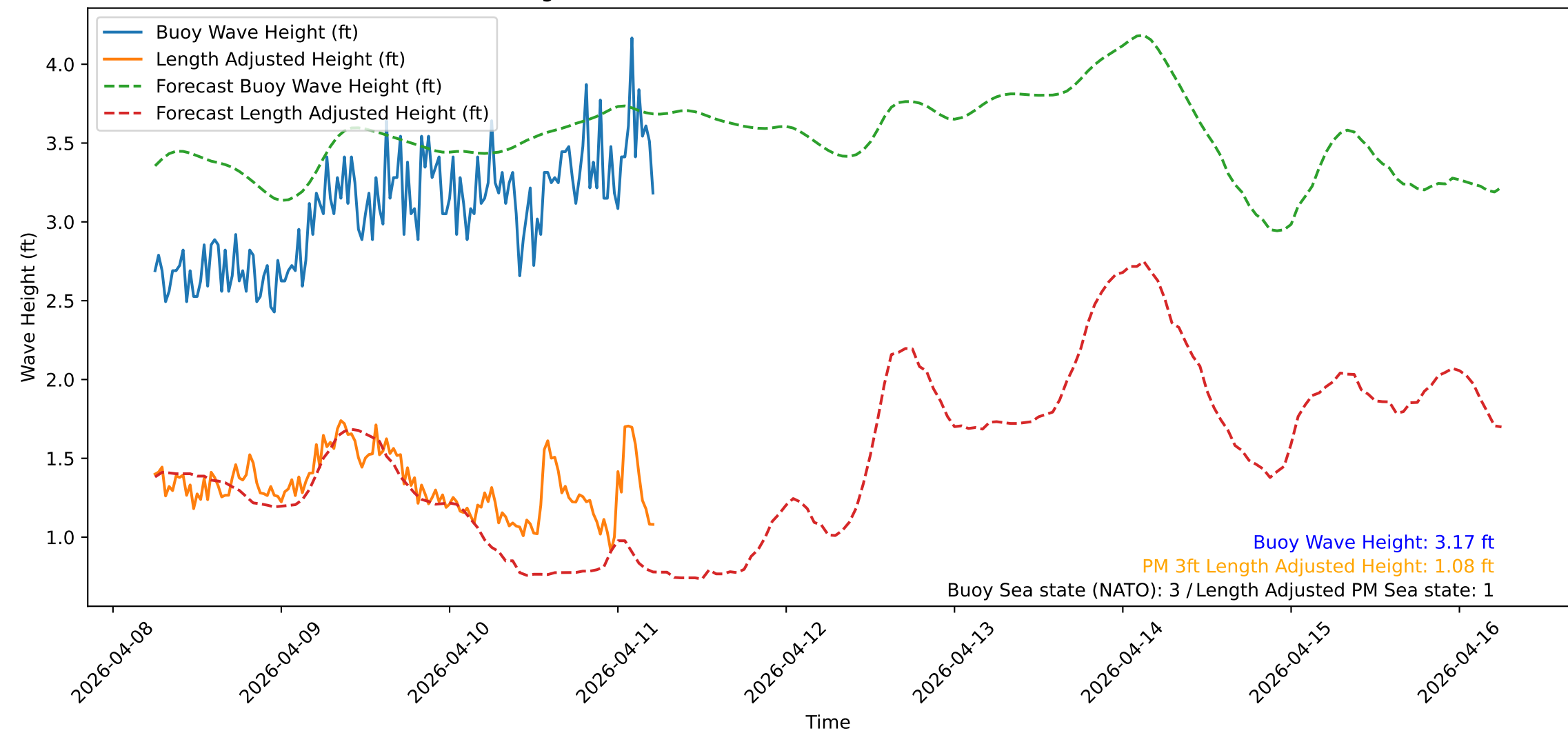
Wave Heights over Time for Oceanside Harbor at 2026-04-11 05:50:31
