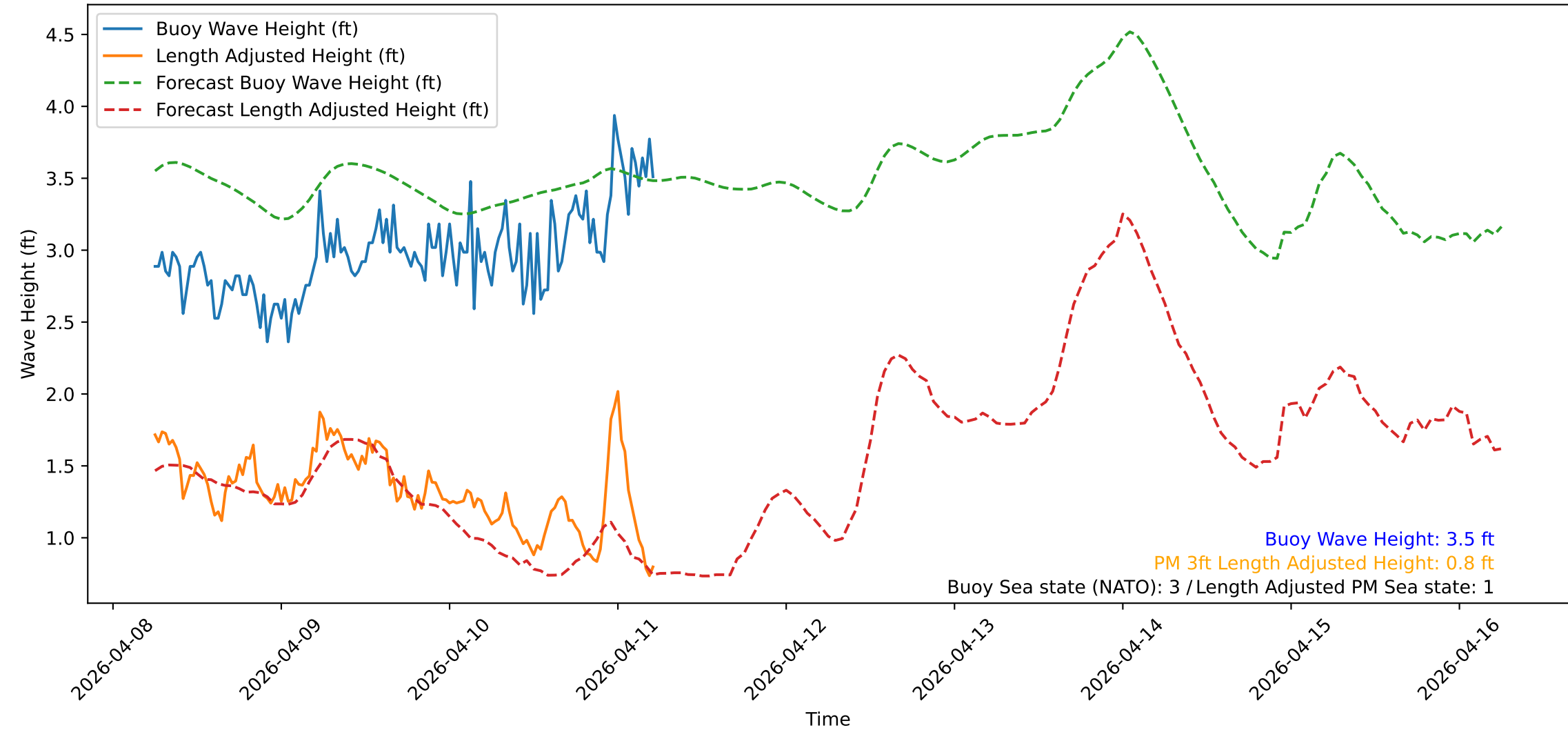
Wave Heights over Time for Green Beach at 2026-04-11 05:51:14
