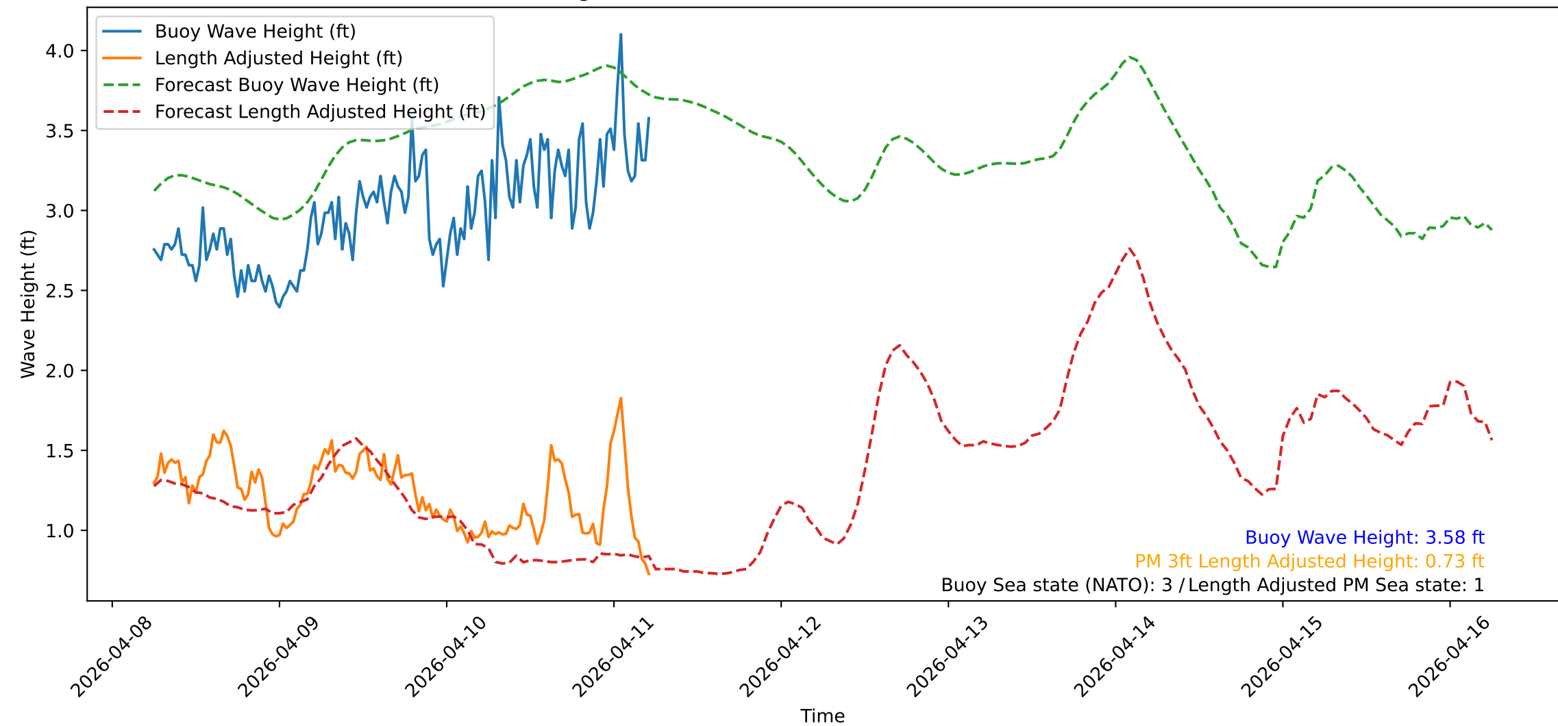
Wave Heights over Time for Red Beach at 2026-04-11 05:50:52
