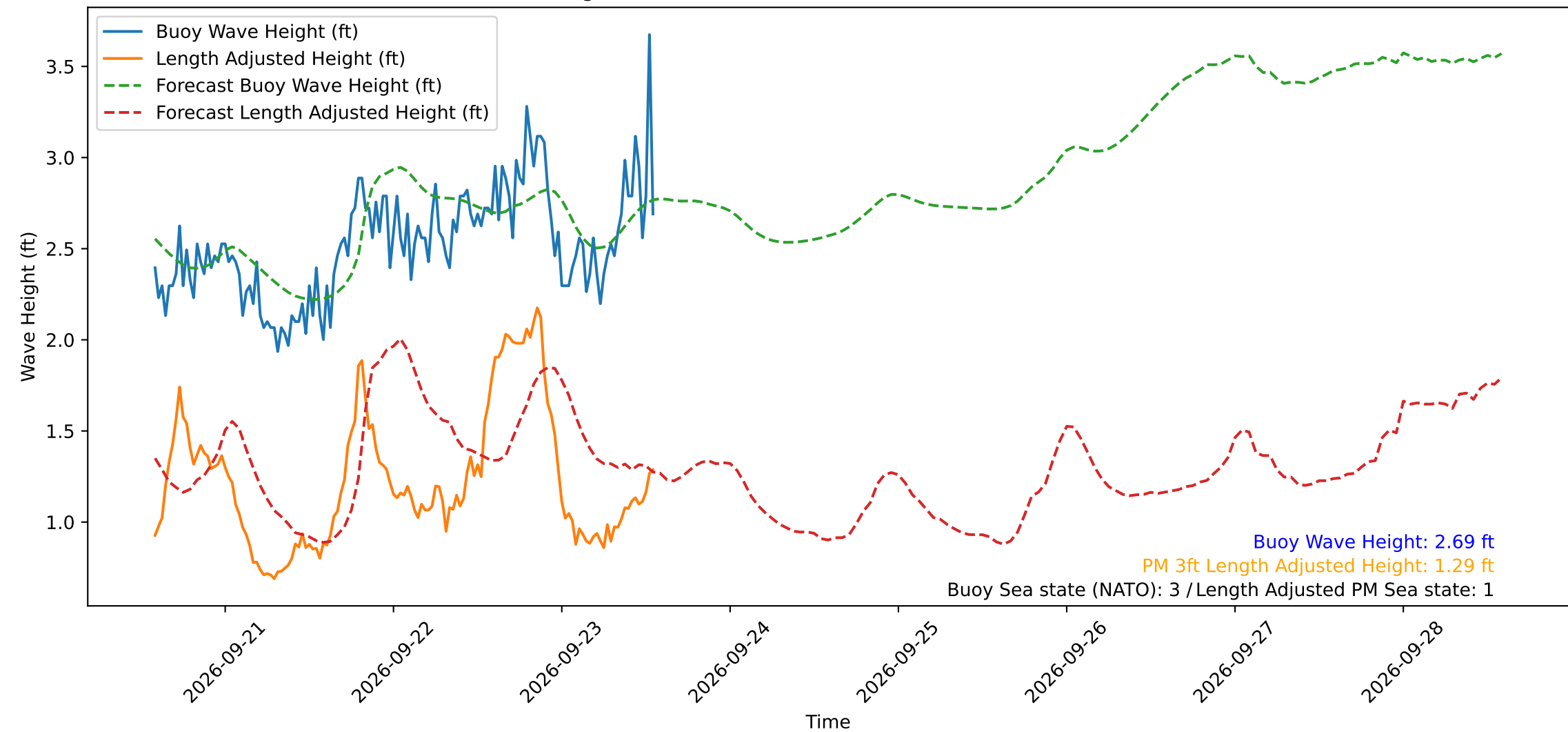
Wave Heights over Time for Red Beach at 2026-09-23 13:40:50
