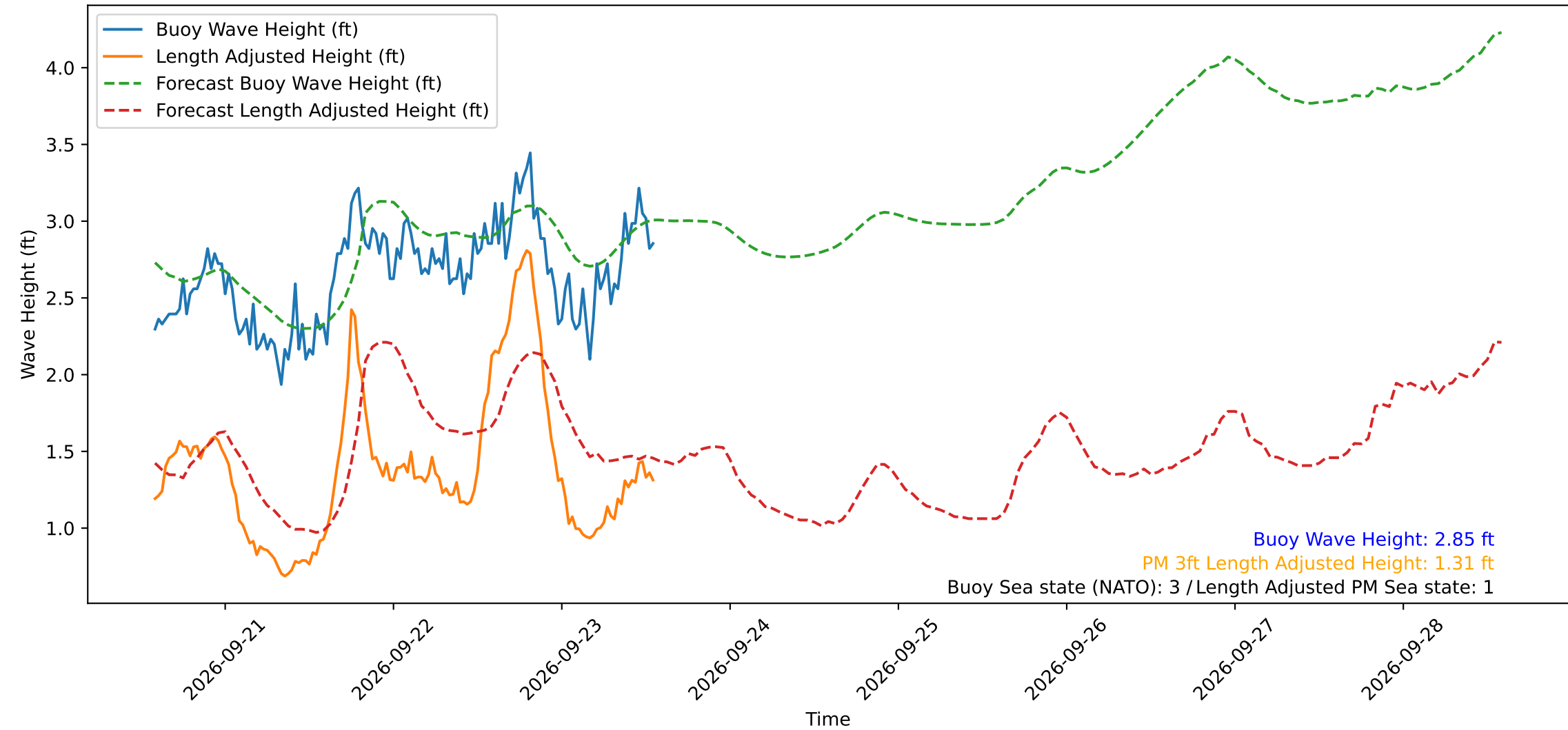
Wave Heights over Time for Green Beach at 2026-09-23 13:41:12
