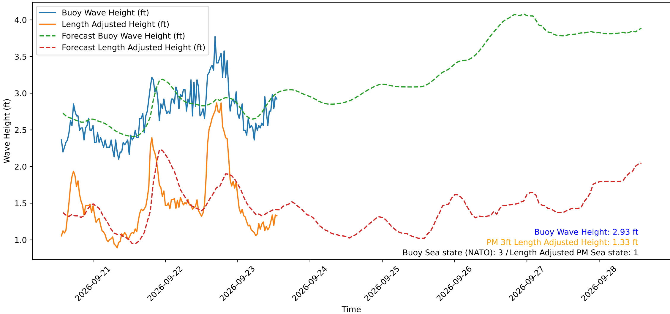
Wave Heights over Time for Oceanside Harbor at 2026-09-23 13:40:30
