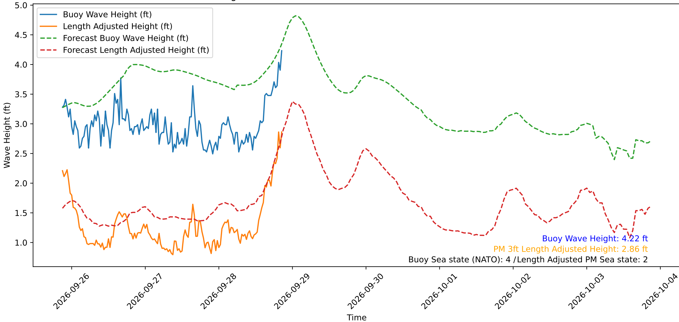
Wave Heights over Time for Oceanside Harbor at 2026-09-28 21:10:29
