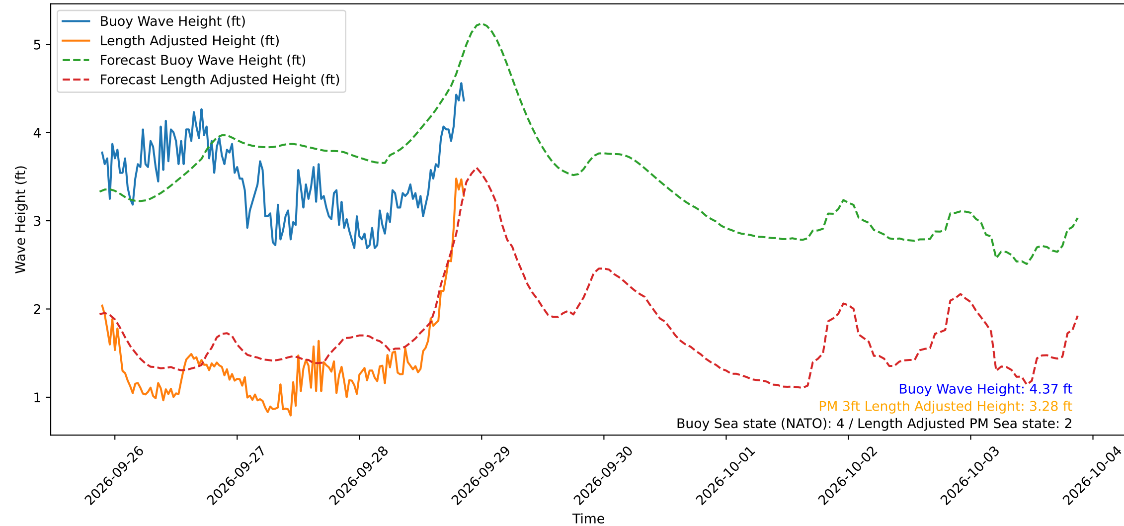
Wave Heights over Time for Green Beach at 2026-09-28 21:11:14
