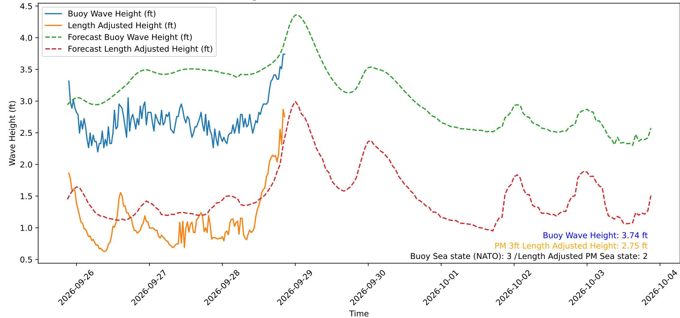
Wave Heights over Time for Red Beach at 2026-09-28 21:10:50
