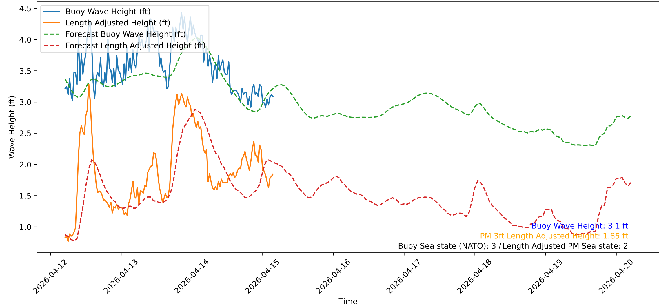
Wave Heights over Time for Red Beach at 2026-04-15 04:30:50
