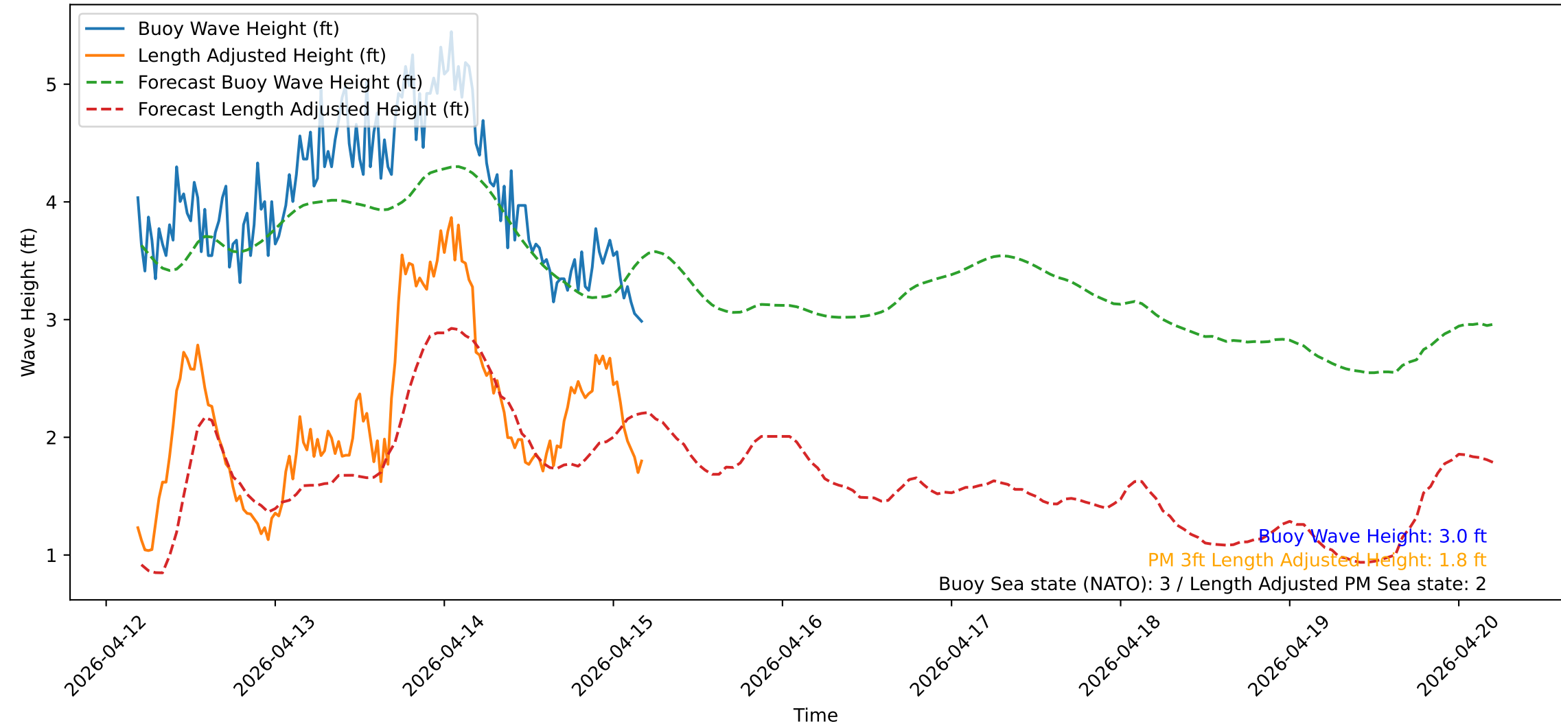
Wave Heights over Time for Oceanside Harbor at 2026-04-15 04:30:32
