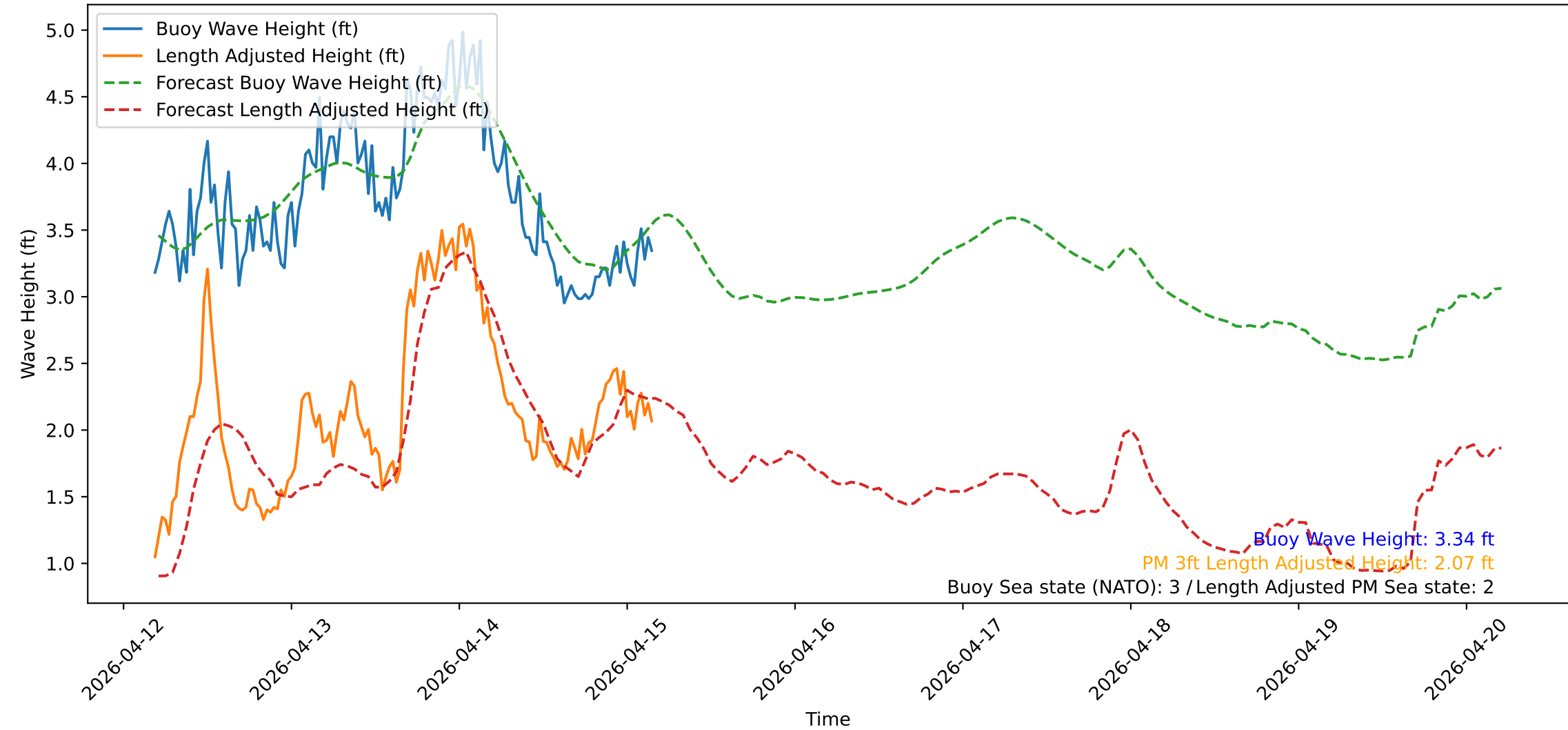
Wave Heights over Time for Green Beach at 2026-04-15 04:31:13
