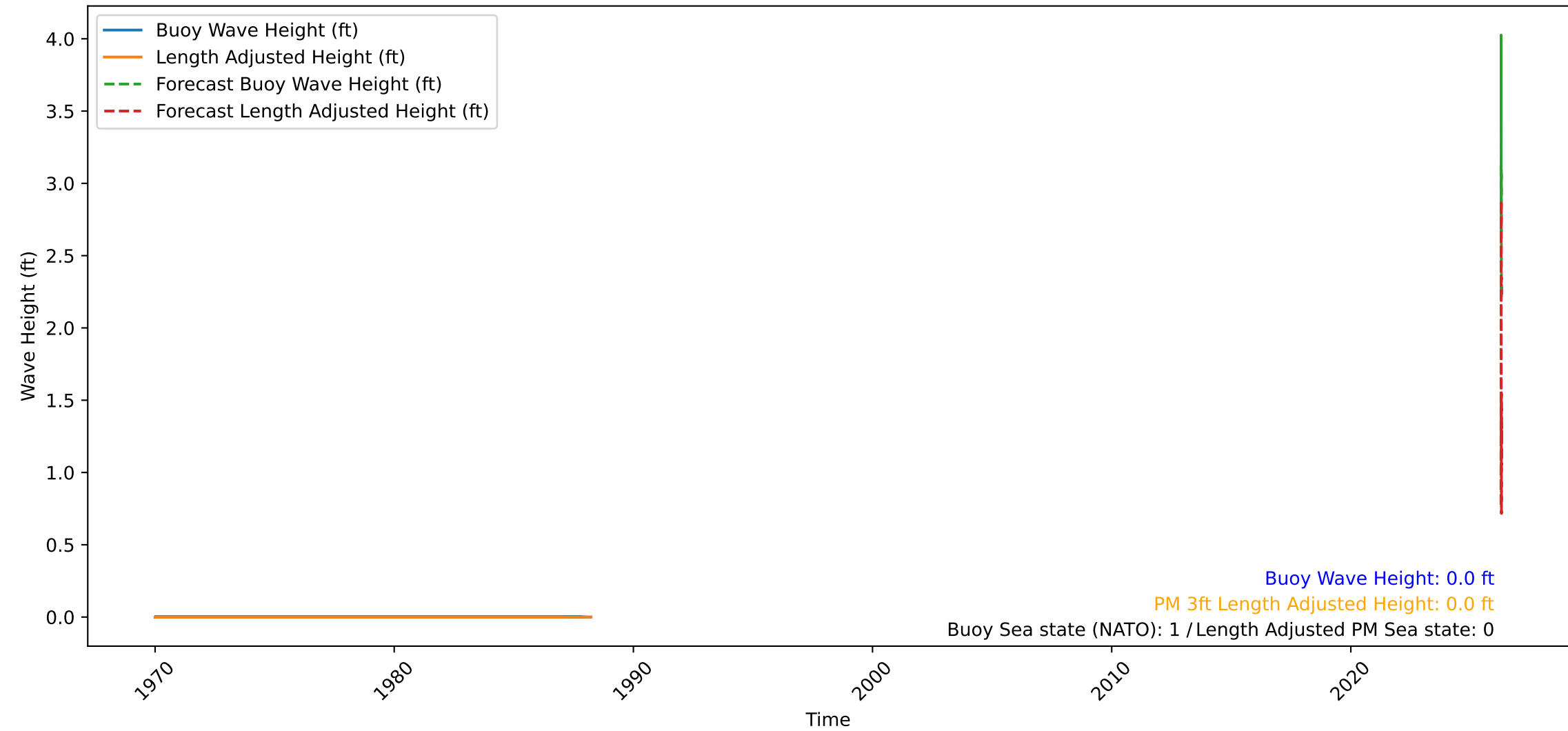
Wave Heights over Time for Red Beach at 2026-04-15 08:10:51
