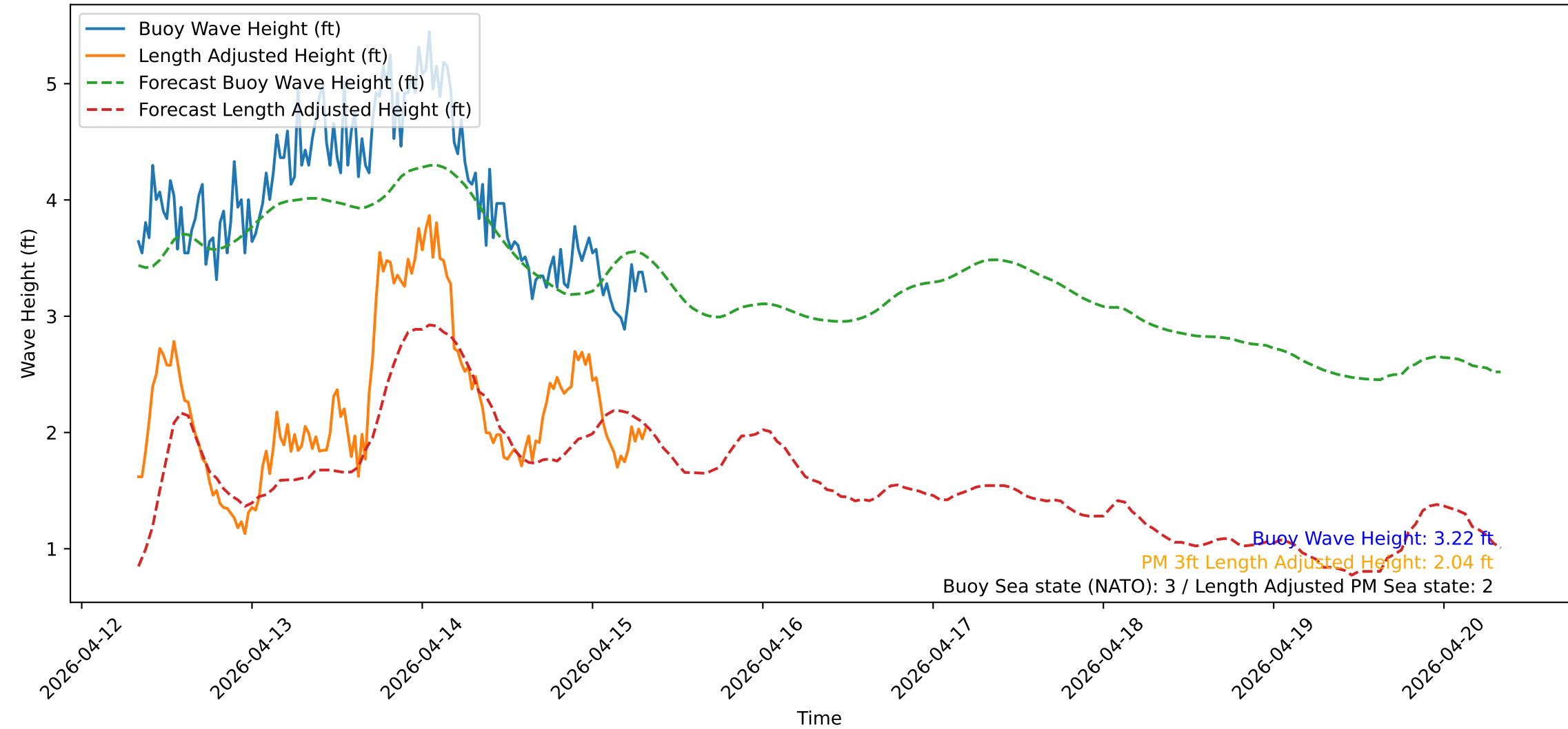
Wave Heights over Time for Oceanside Harbor at 2026-04-15 08:10:31
