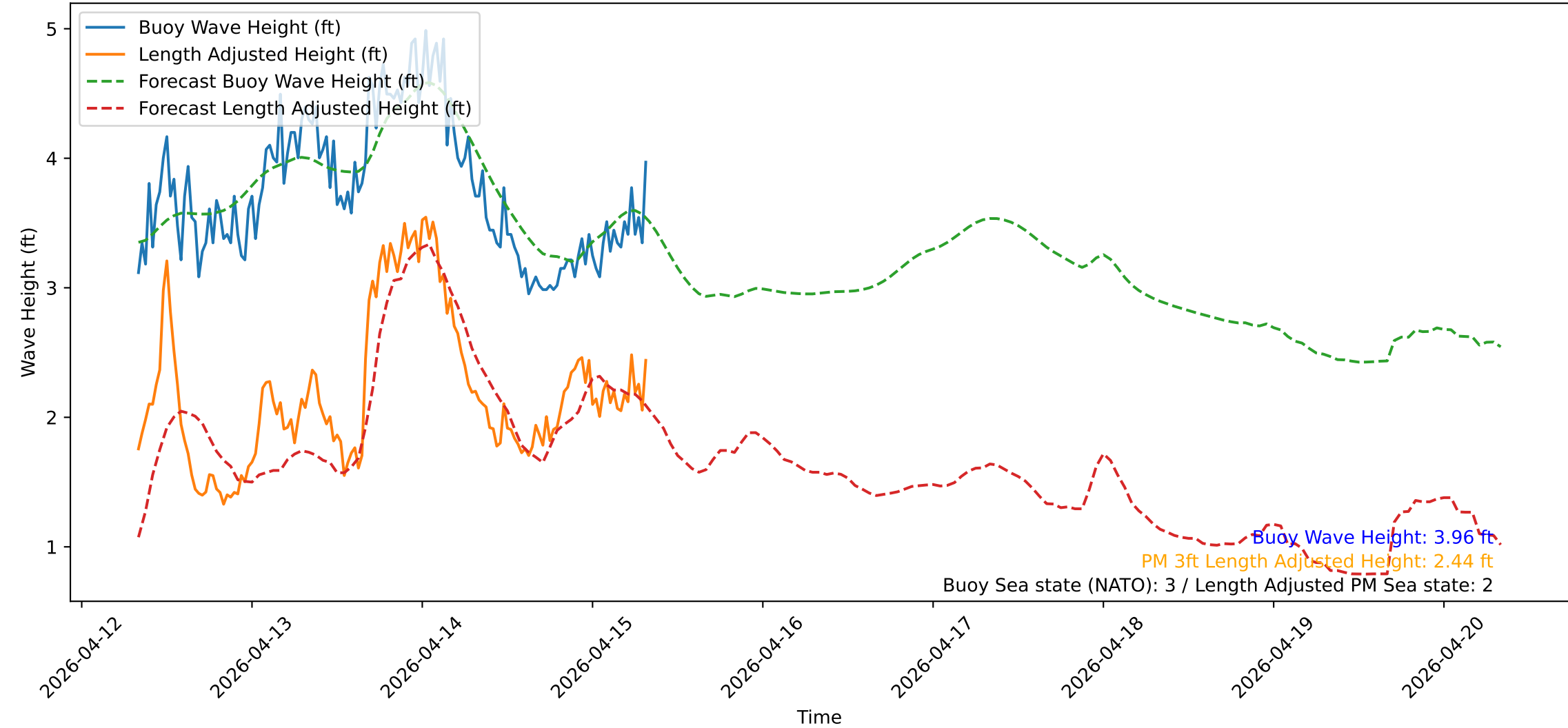
Wave Heights over Time for Green Beach at 2026-04-15 08:11:13
