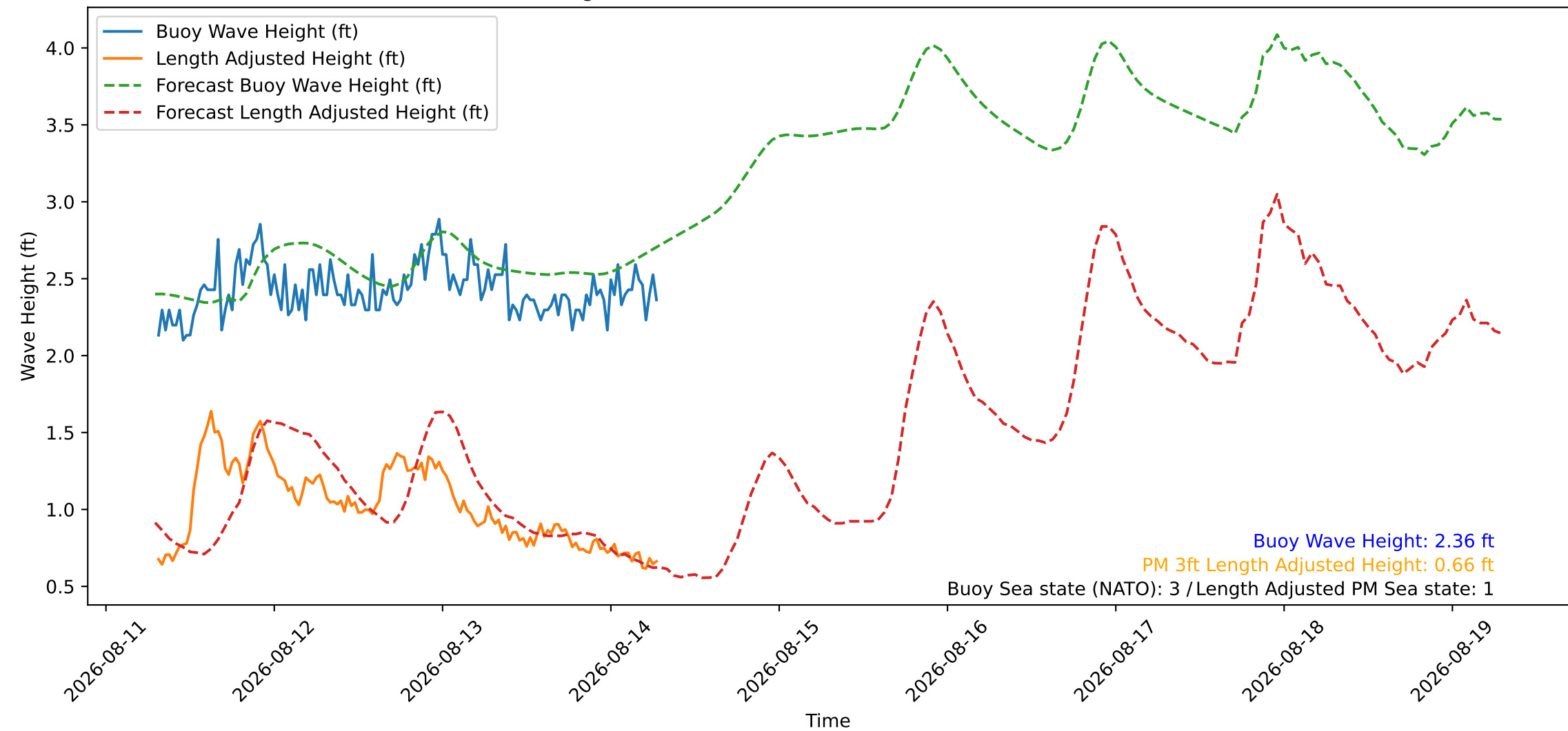
Wave Heights over Time for Red Beach at 2026-08-14 07:10:46
