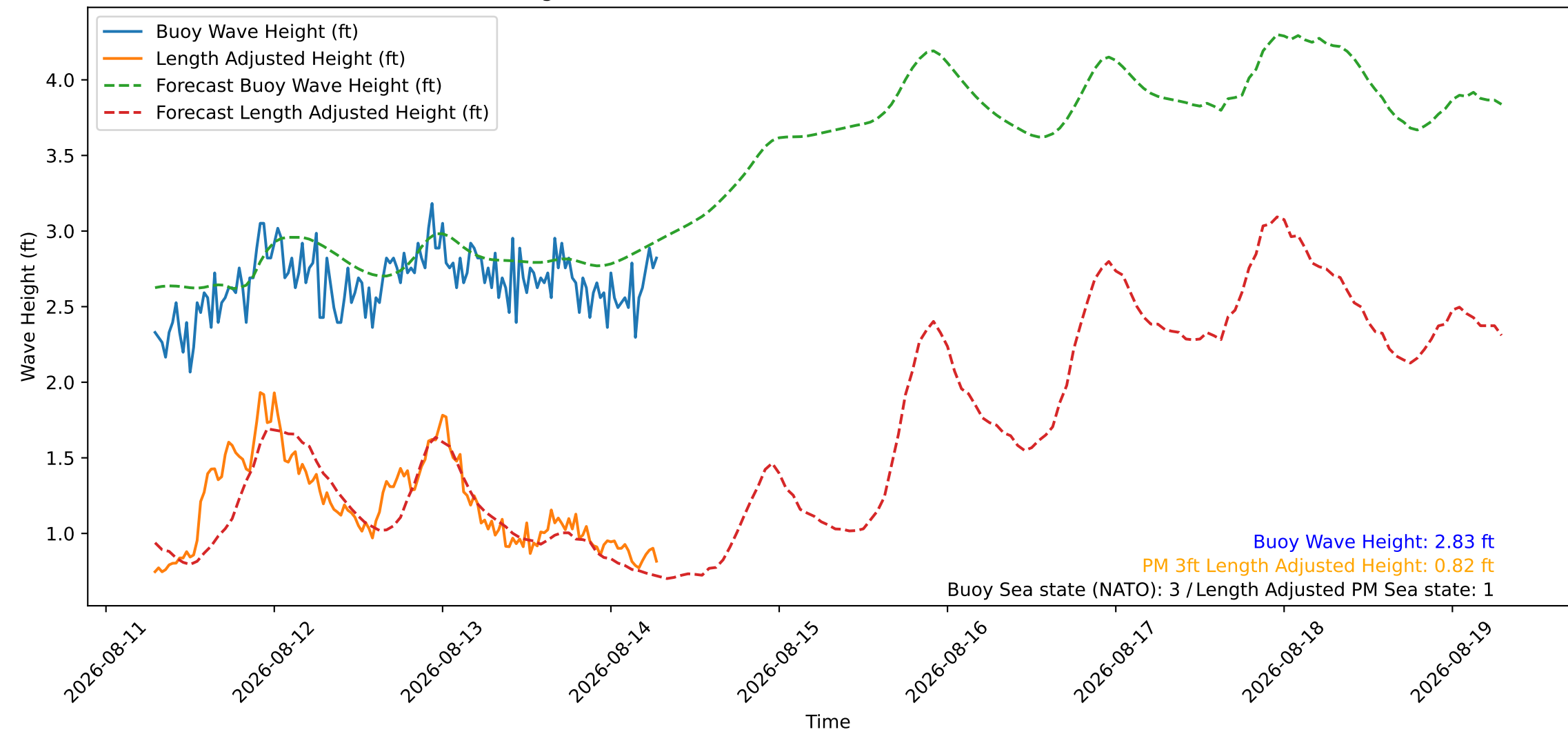
Wave Heights over Time for Oceanside Harbor at 2026-08-14 07:10:27
