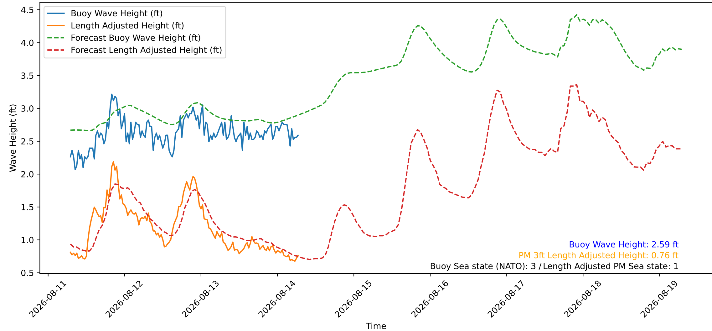
Wave Heights over Time for Green Beach at 2026-08-14 07:11:08
