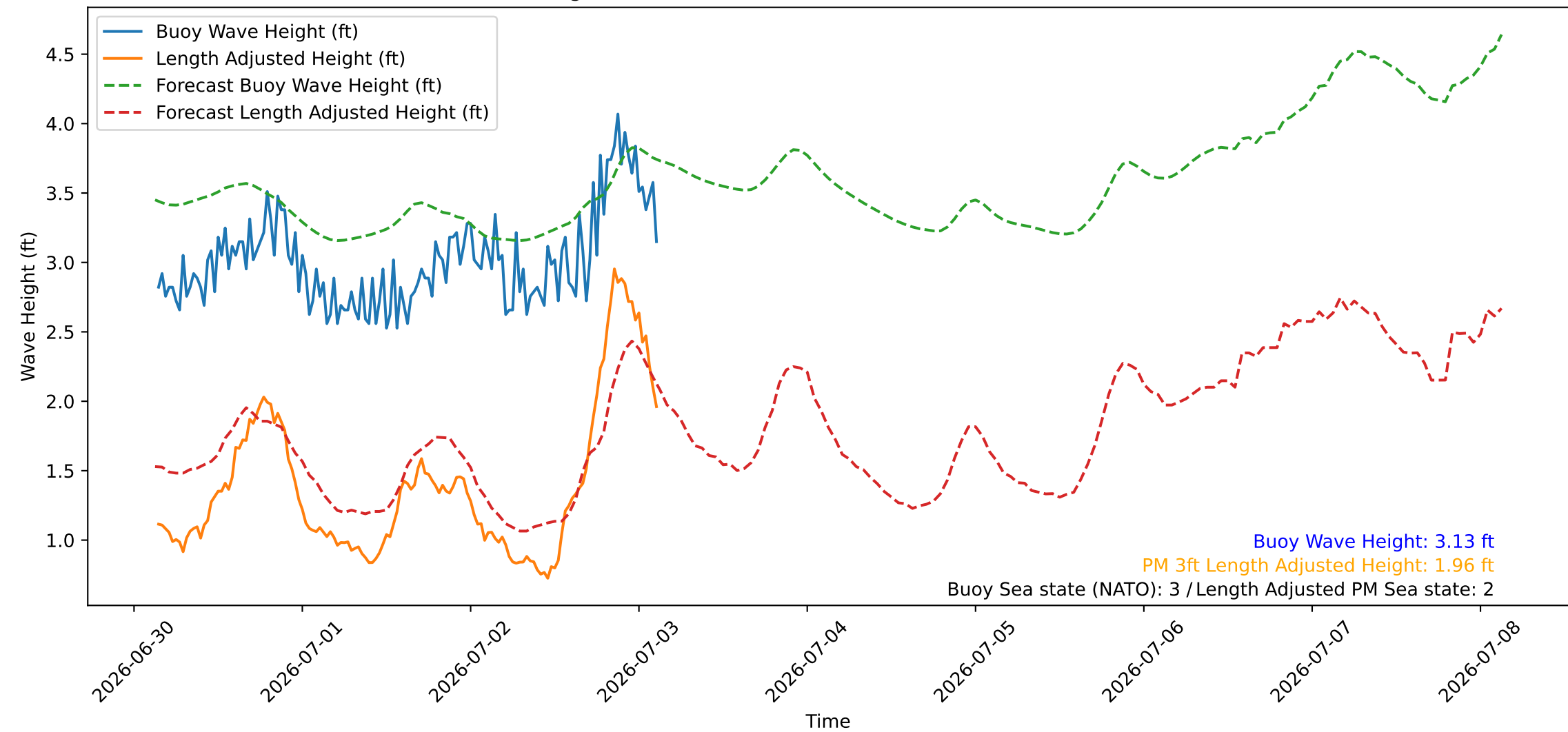
Wave Heights over Time for Green Beach at 2026-07-03 03:21:09
