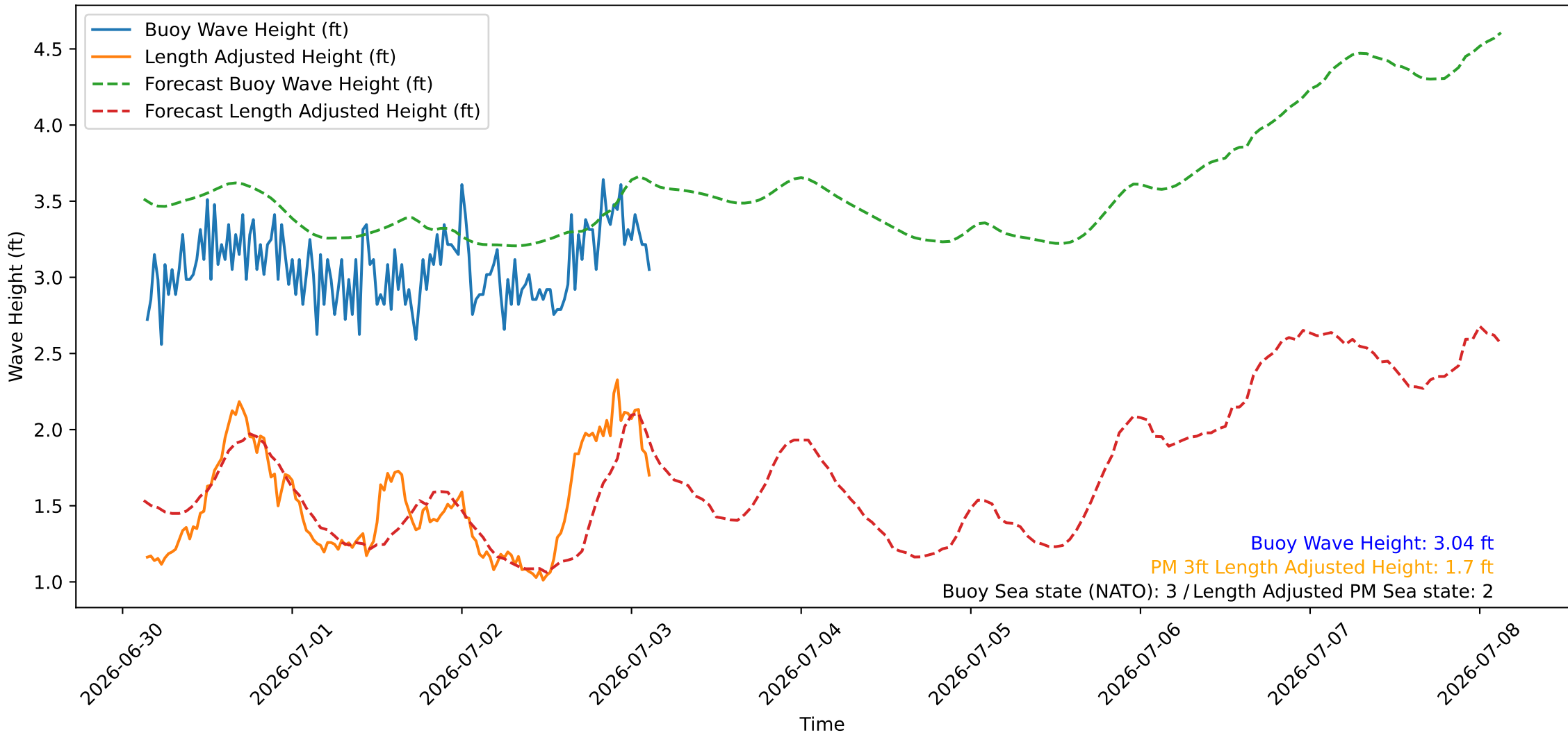
Wave Heights over Time for Oceanside Harbor at 2026-07-03 03:20:26
