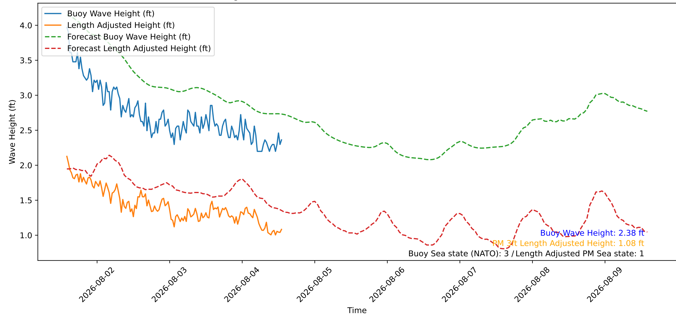
Wave Heights over Time for Oceanside Harbor at 2026-08-04 13:50:26
