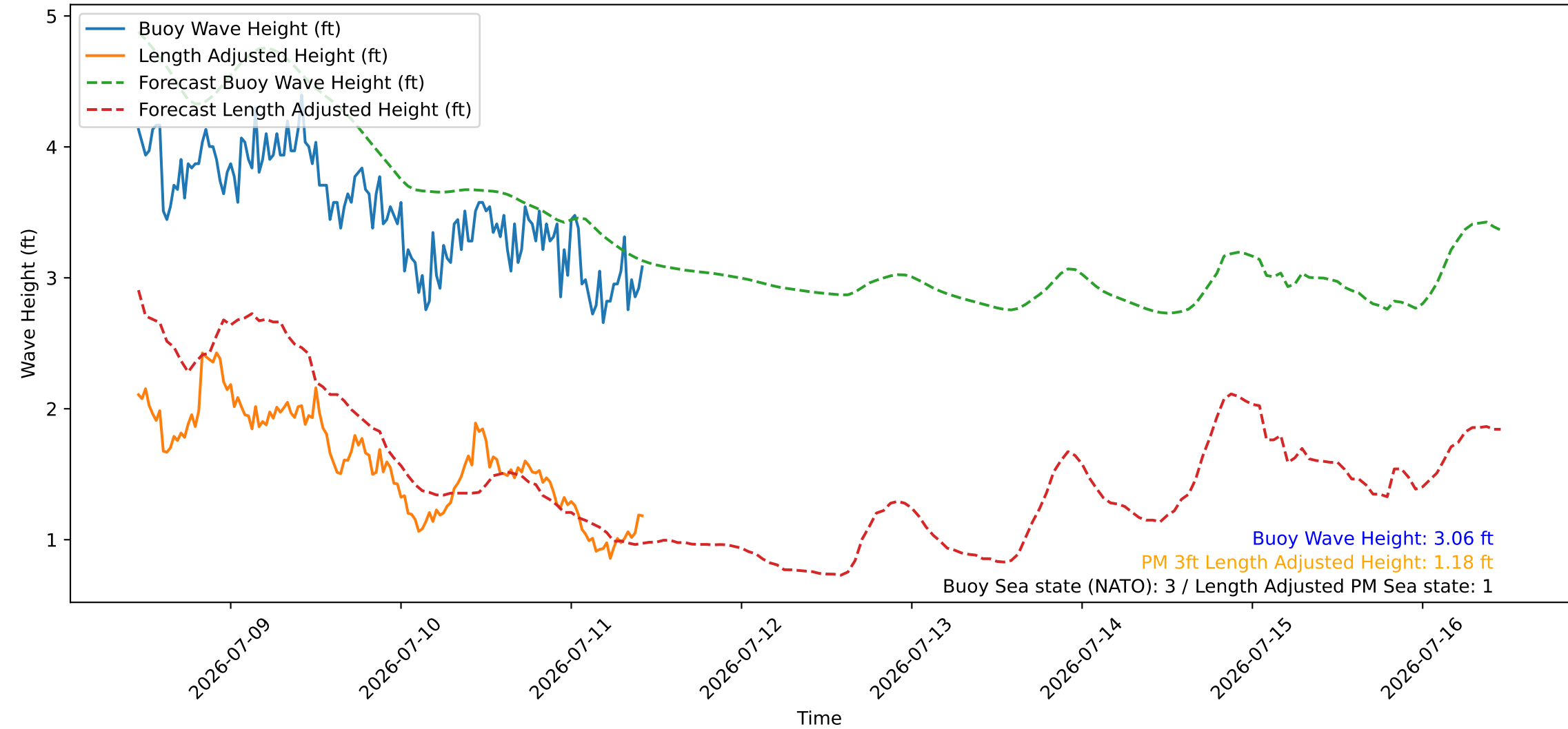
Wave Heights over Time for Green Beach at 2026-07-11 11:01:09
