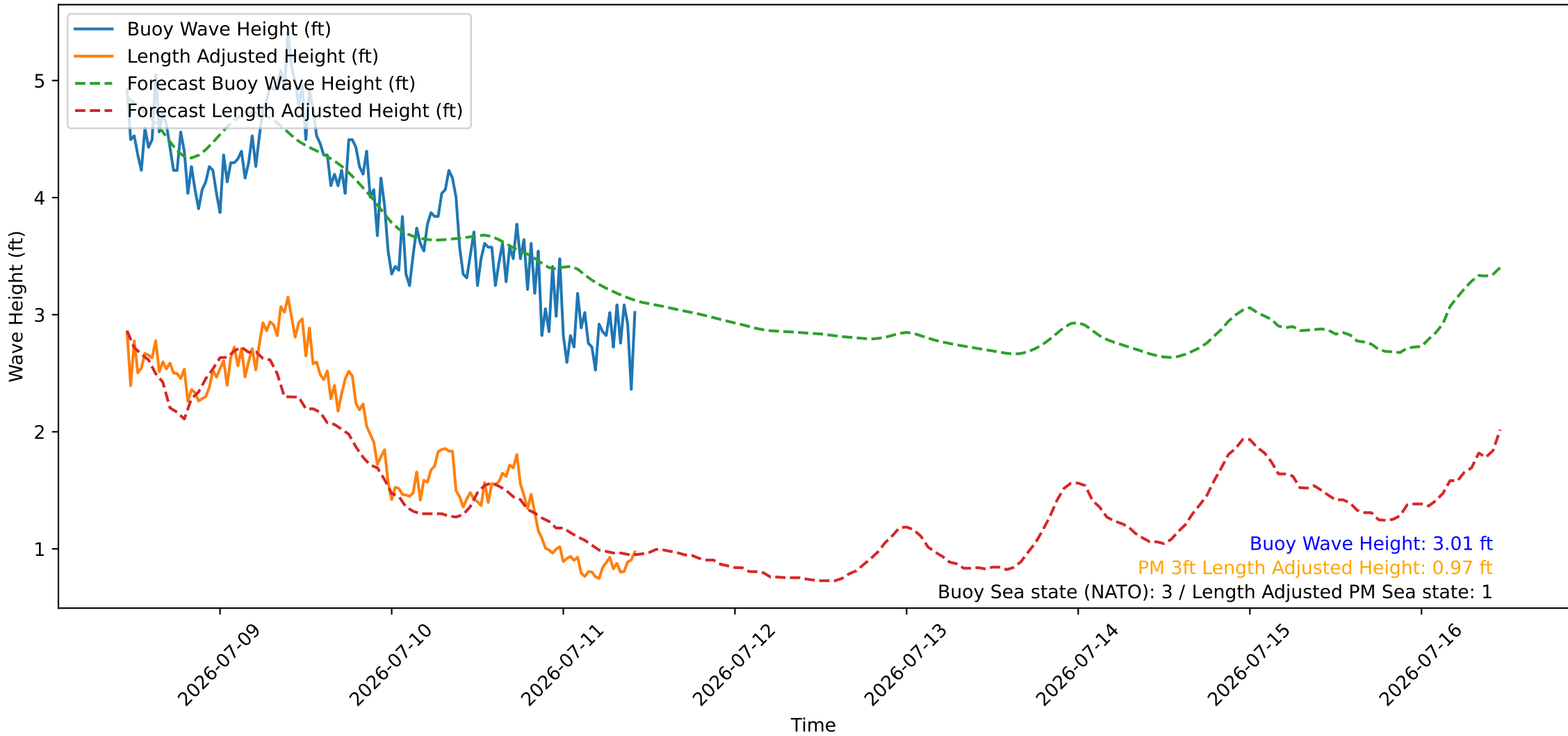
Wave Heights over Time for Oceanside Harbor at 2026-07-11 11:00:26
