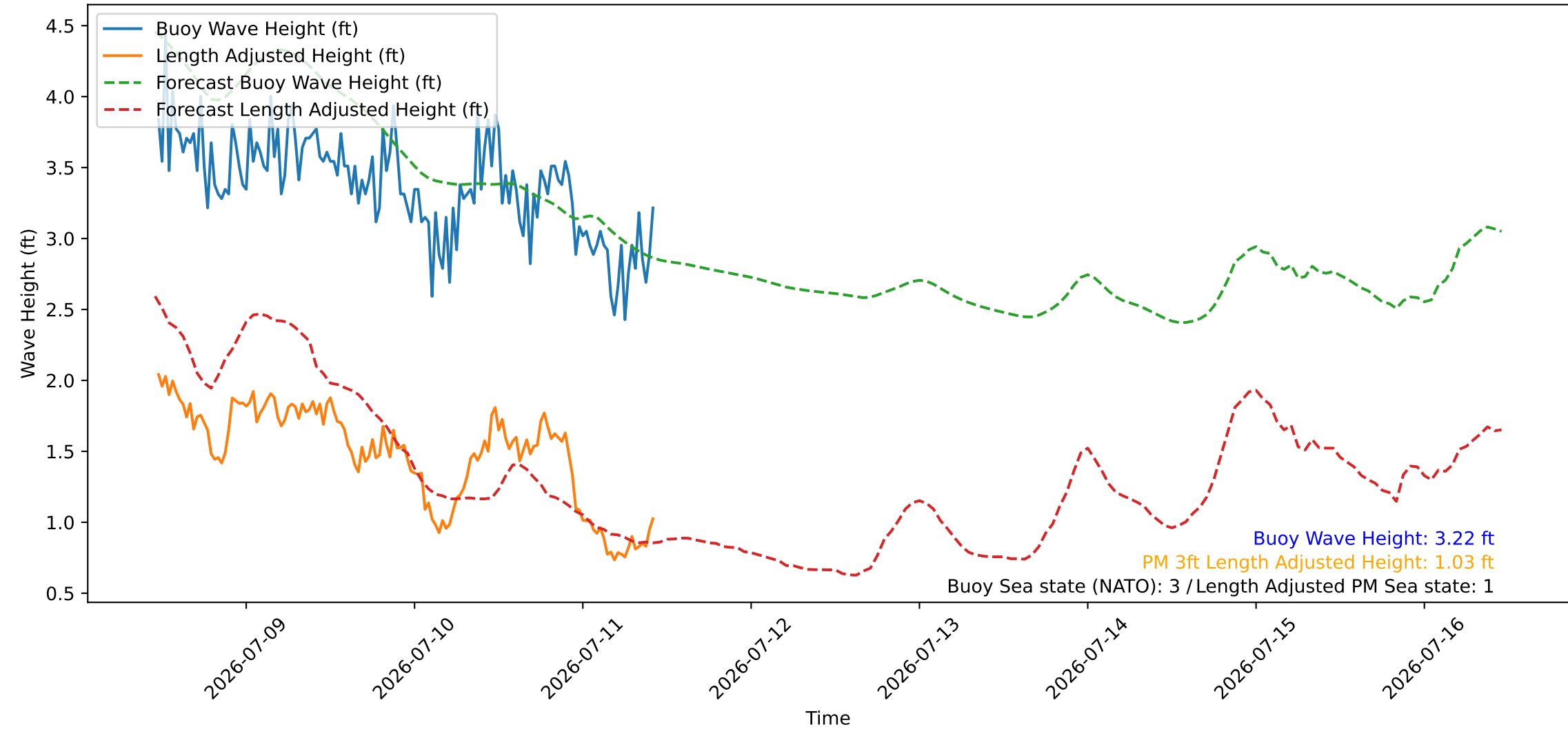
Wave Heights over Time for Red Beach at 2026-07-11 11:00:46
