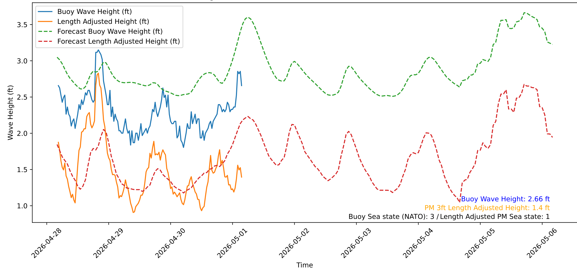
Wave Heights over Time for Green Beach at 2026-05-01 04:21:14
