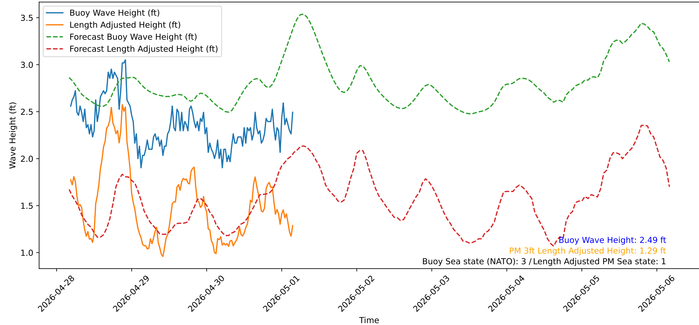
Wave Heights over Time for Oceanside Harbor at 2026-05-01 04:20:31
