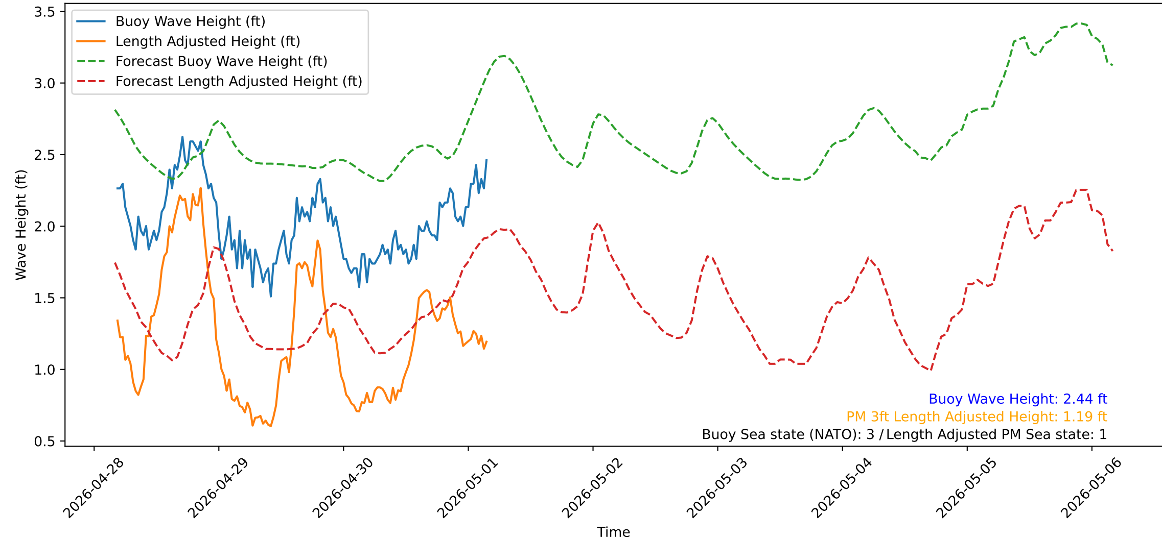
Wave Heights over Time for Red Beach at 2026-05-01 04:20:52
