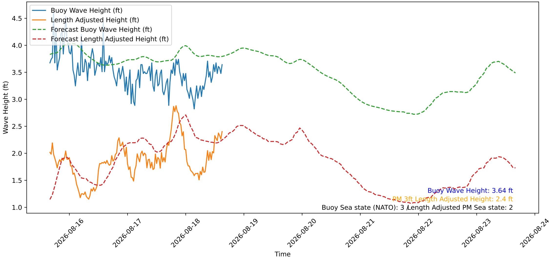
Wave Heights over Time for Oceanside Harbor at 2026-08-18 15:50:26
