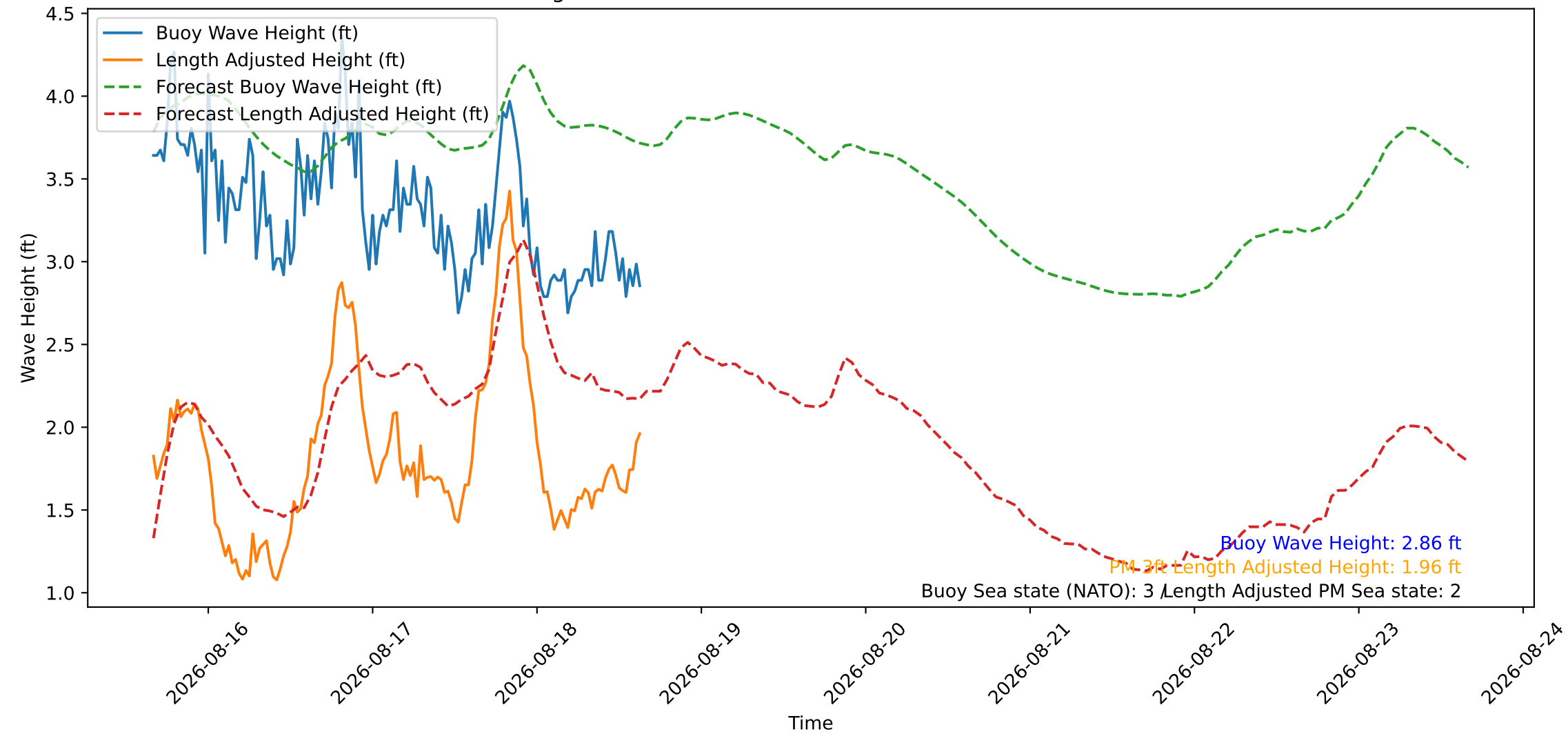
Wave Heights over Time for Green Beach at 2026-08-18 15:51:10
