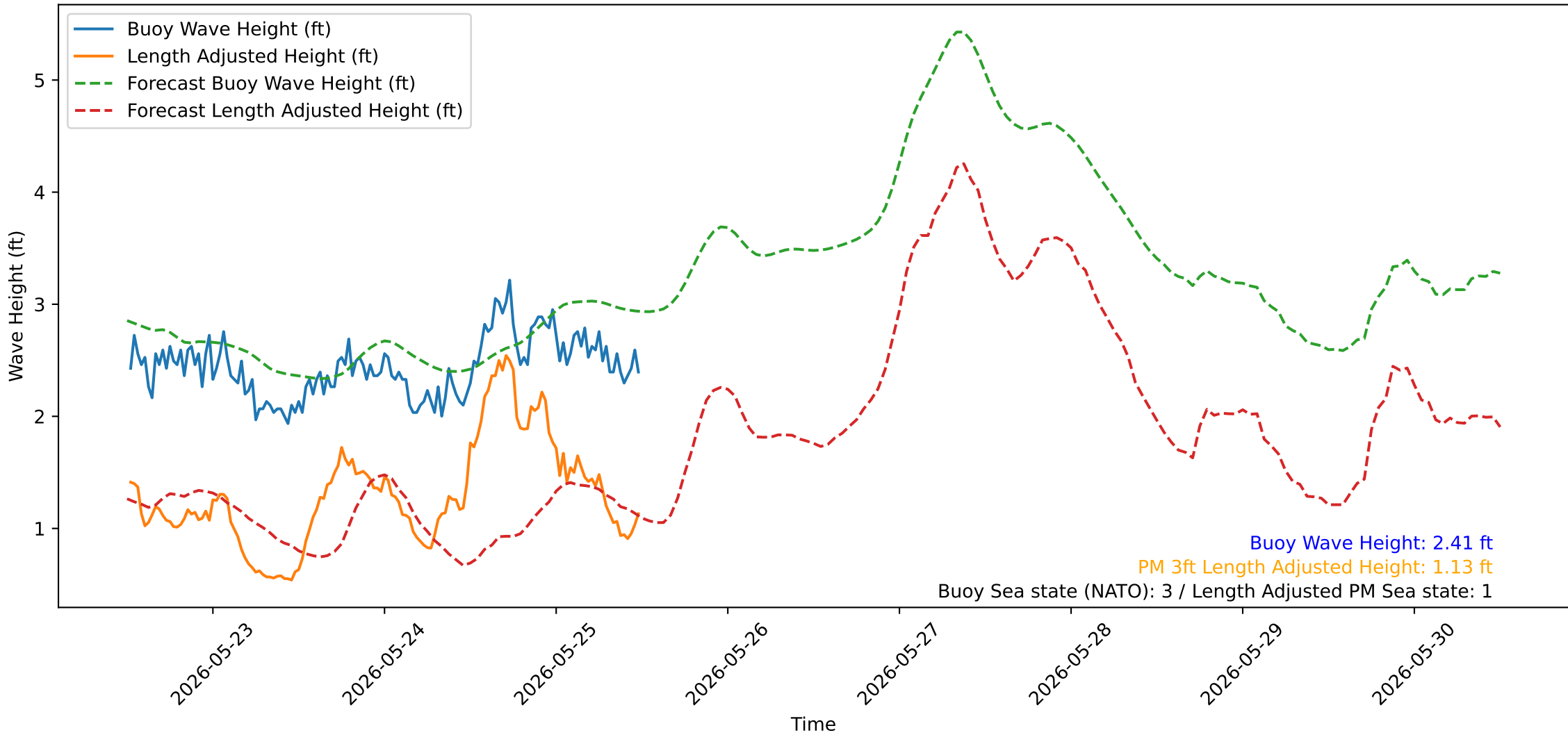
Wave Heights over Time for Red Beach at 2026-05-25 12:10:50
