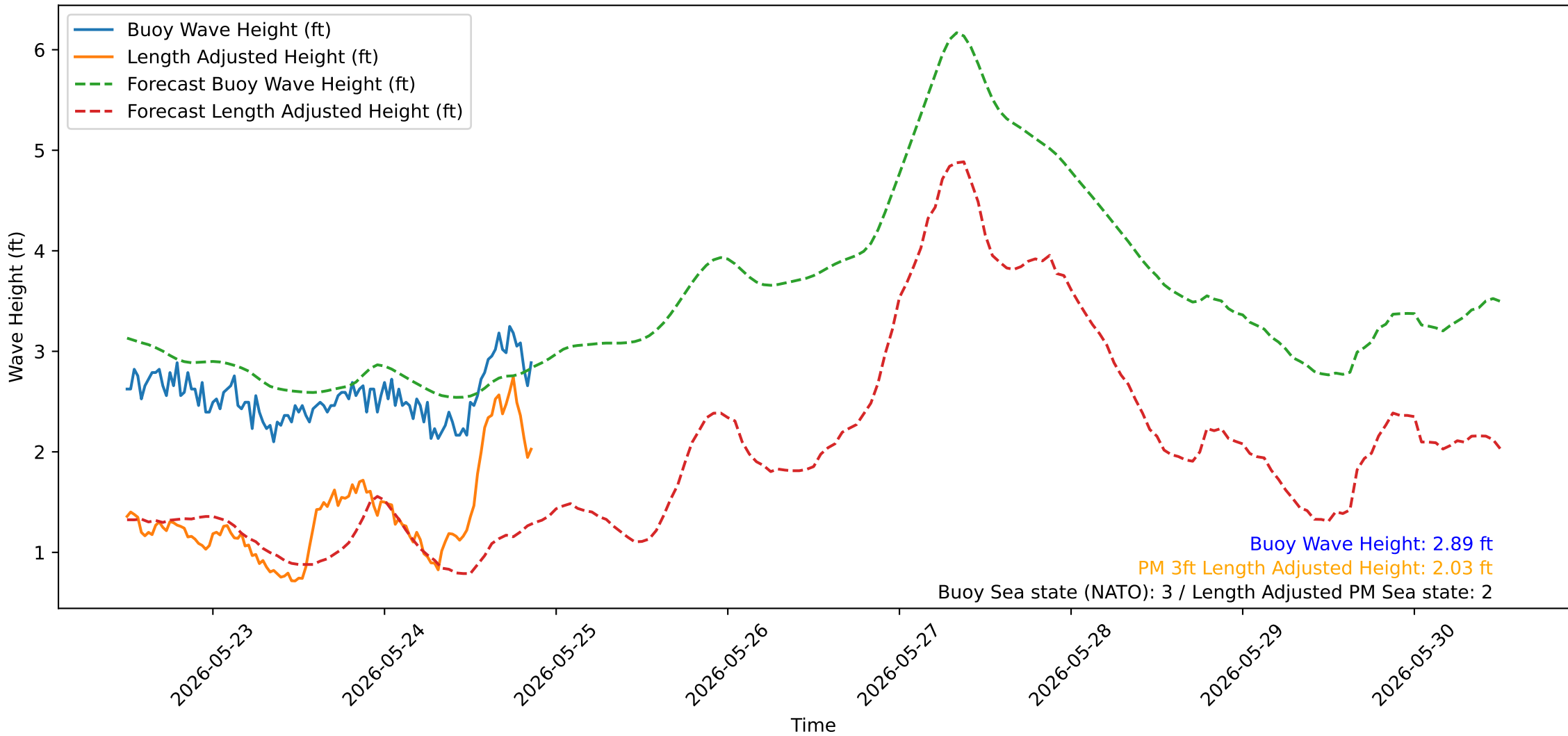
Wave Heights over Time for Oceanside Harbor at 2026-05-25 12:10:31
