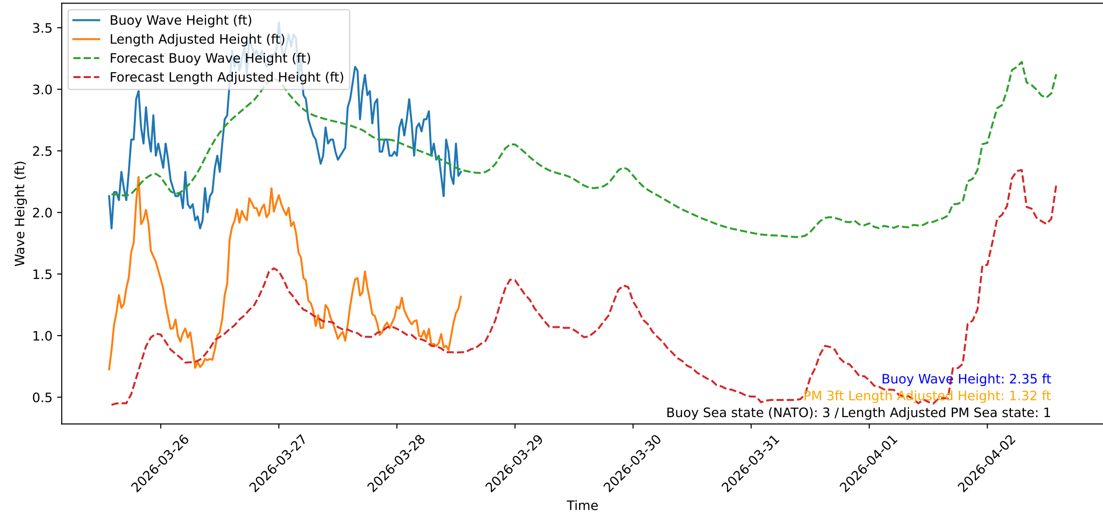
Wave Heights over Time for Green Beach at 2026-03-28 13:41:09
