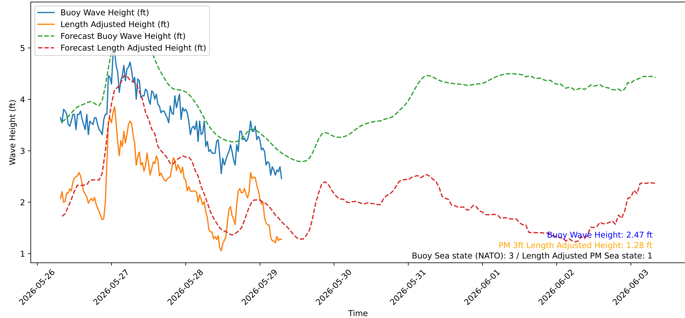
Wave Heights over Time for Green Beach at 2026-05-29 07:41:06
