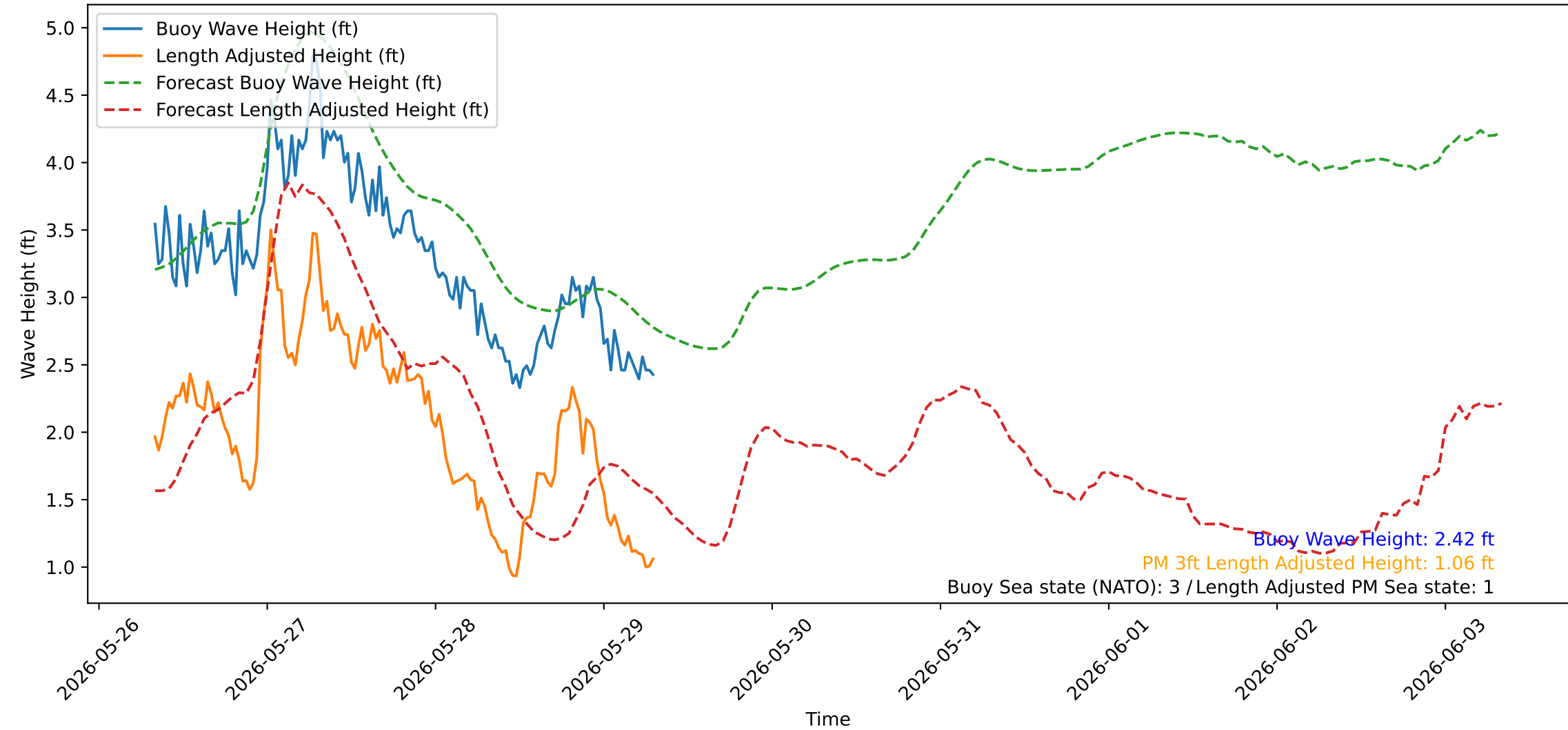
Wave Heights over Time for Red Beach at 2026-05-29 07:40:43
