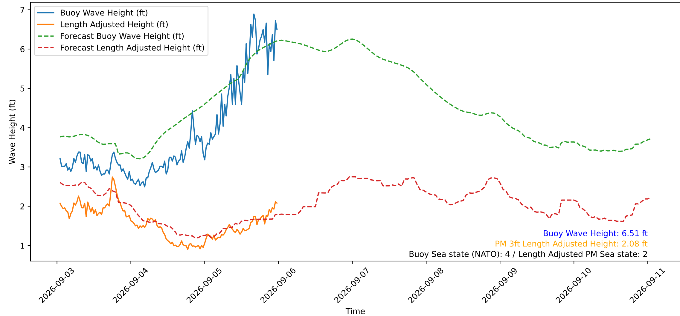
Wave Heights over Time for Green Beach at 2026-09-06 00:31:12
