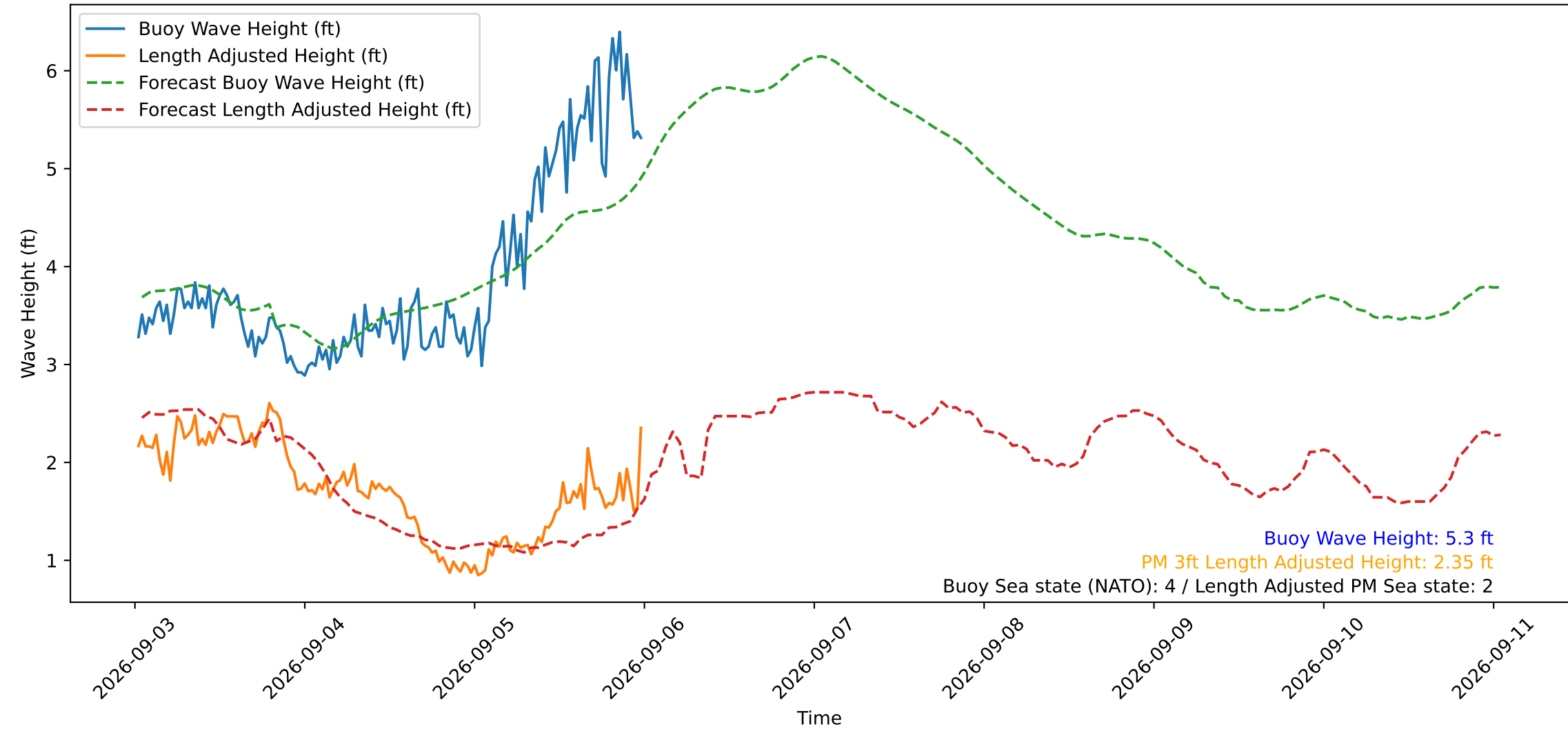
Wave Heights over Time for Oceanside Harbor at 2026-09-06 00:30:30
