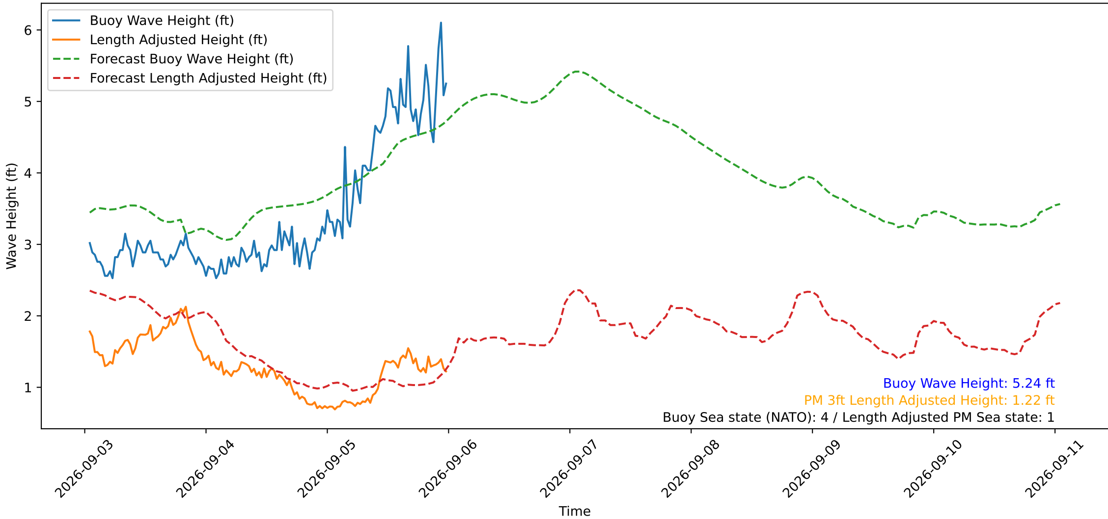
Wave Heights over Time for Red Beach at 2026-09-06 00:30:49
