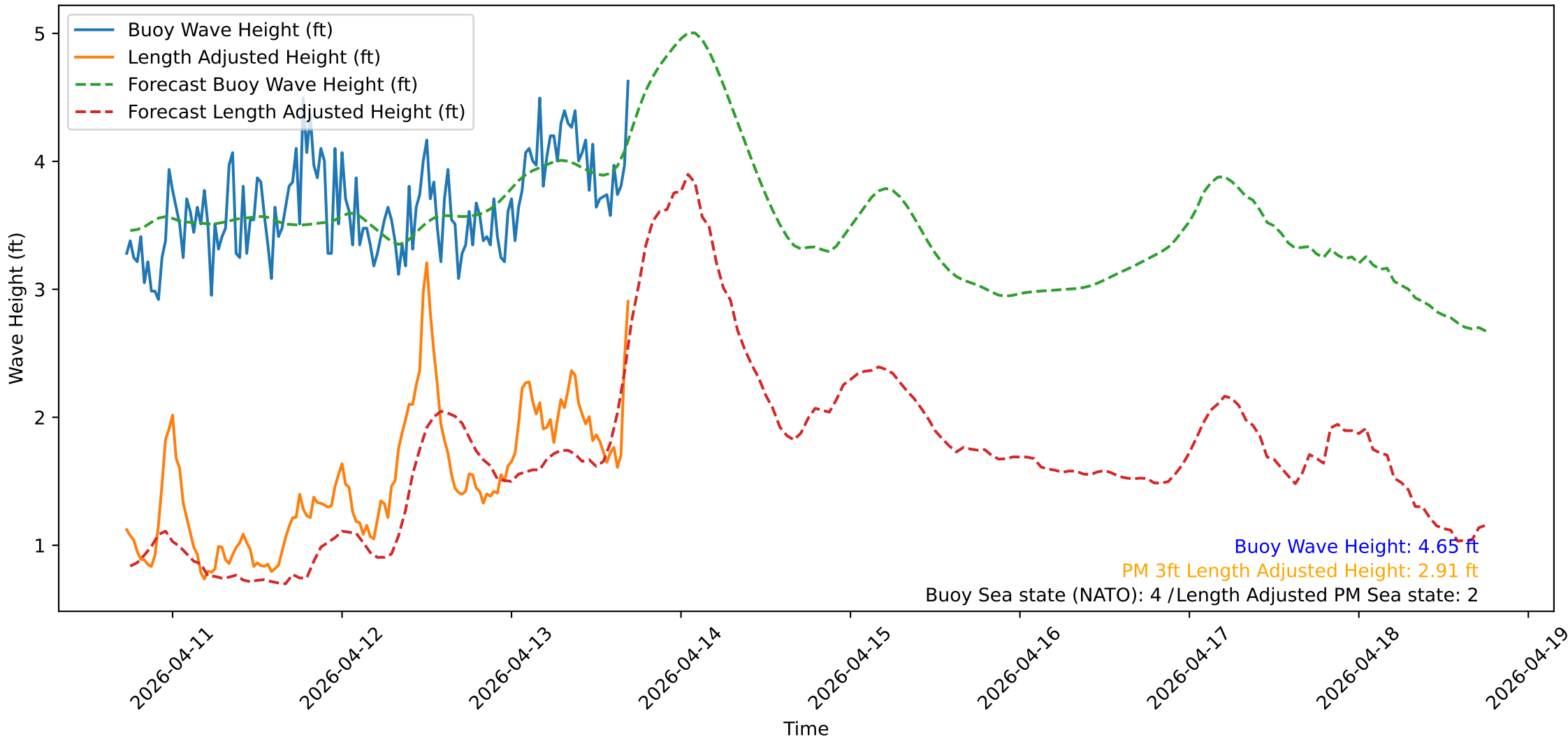
Wave Heights over Time for Green Beach at 2026-04-13 17:31:13
