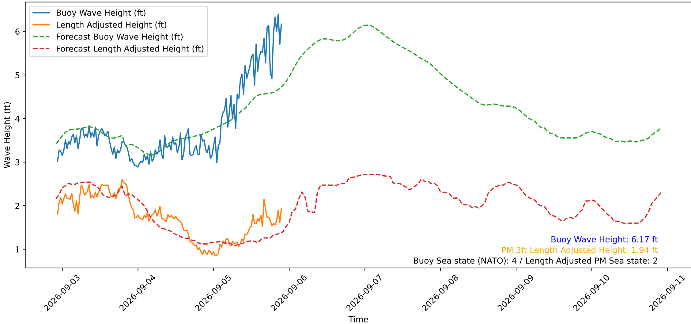
Wave Heights over Time for Oceanside Harbor at 2026-09-05 22:20:30
