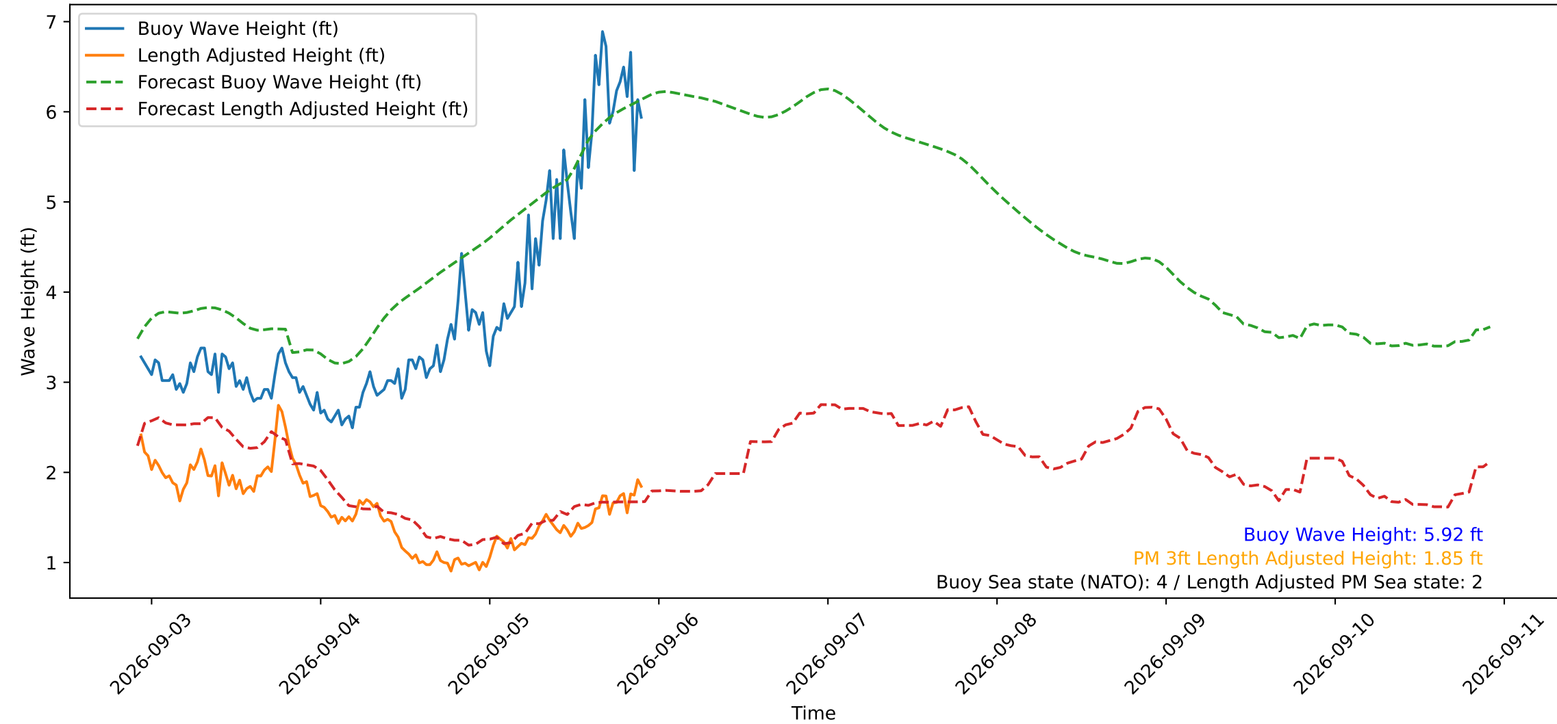
Wave Heights over Time for Green Beach at 2026-09-05 22:21:16
