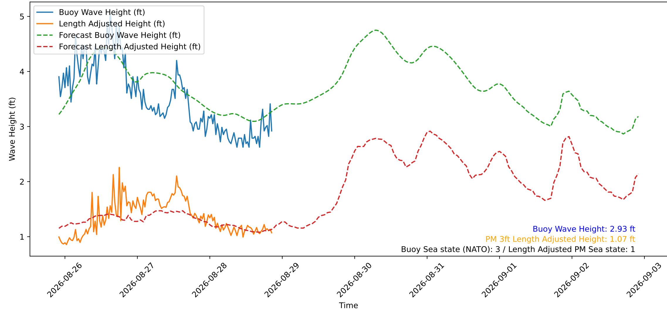
Wave Heights over Time for Red Beach at 2026-08-28 21:30:49
