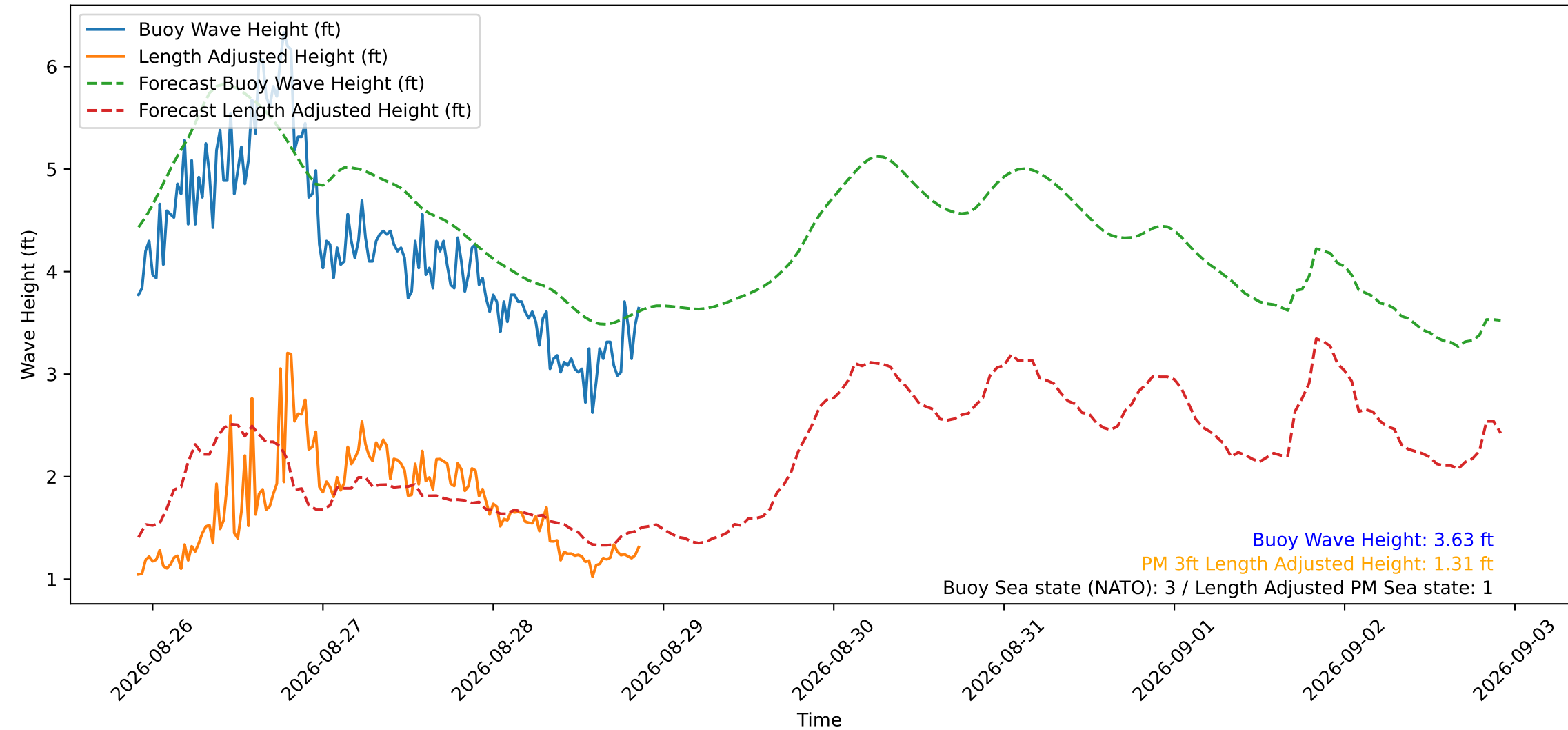
Wave Heights over Time for Green Beach at 2026-08-28 21:31:12
