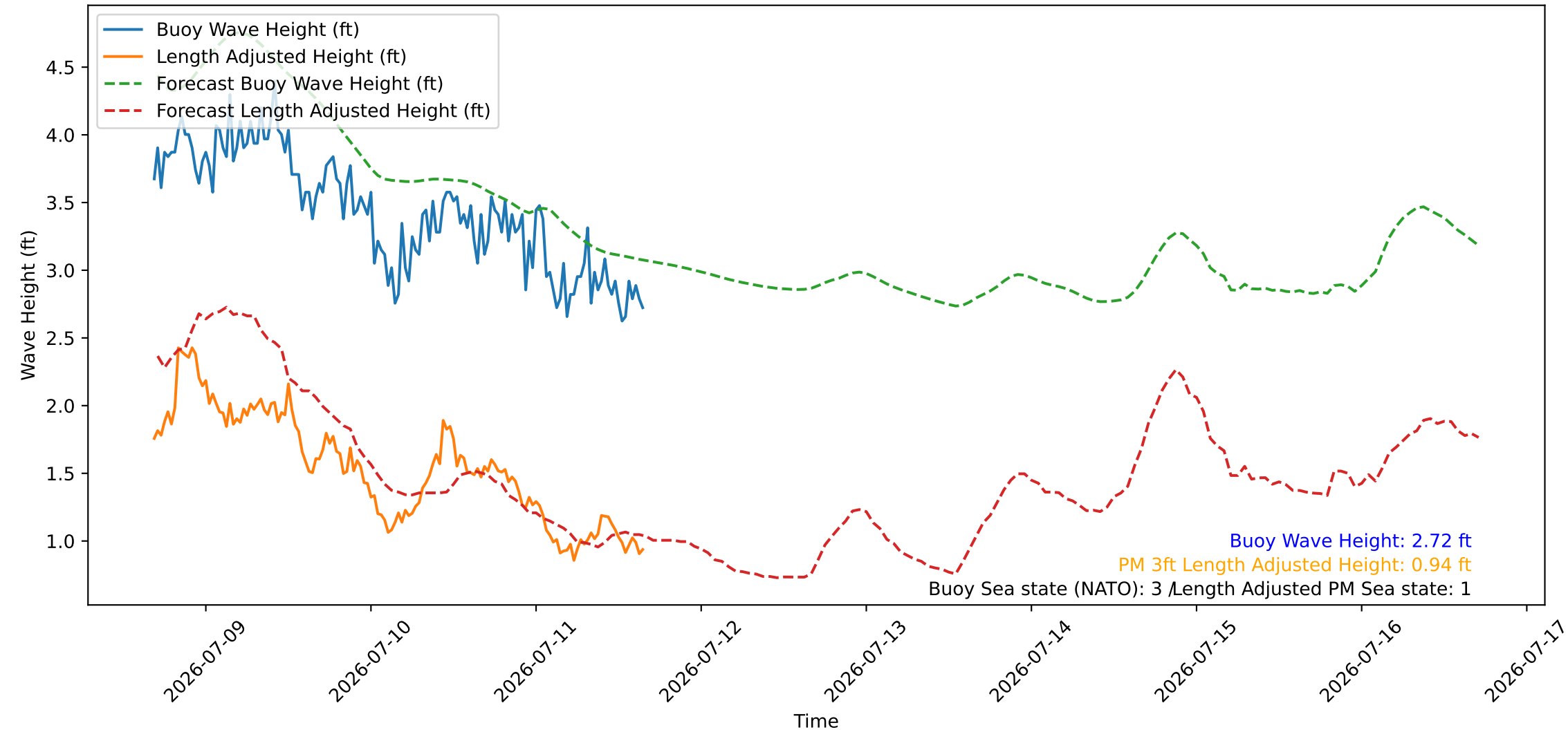
Wave Heights over Time for Green Beach at 2026-07-11 16:31:08
