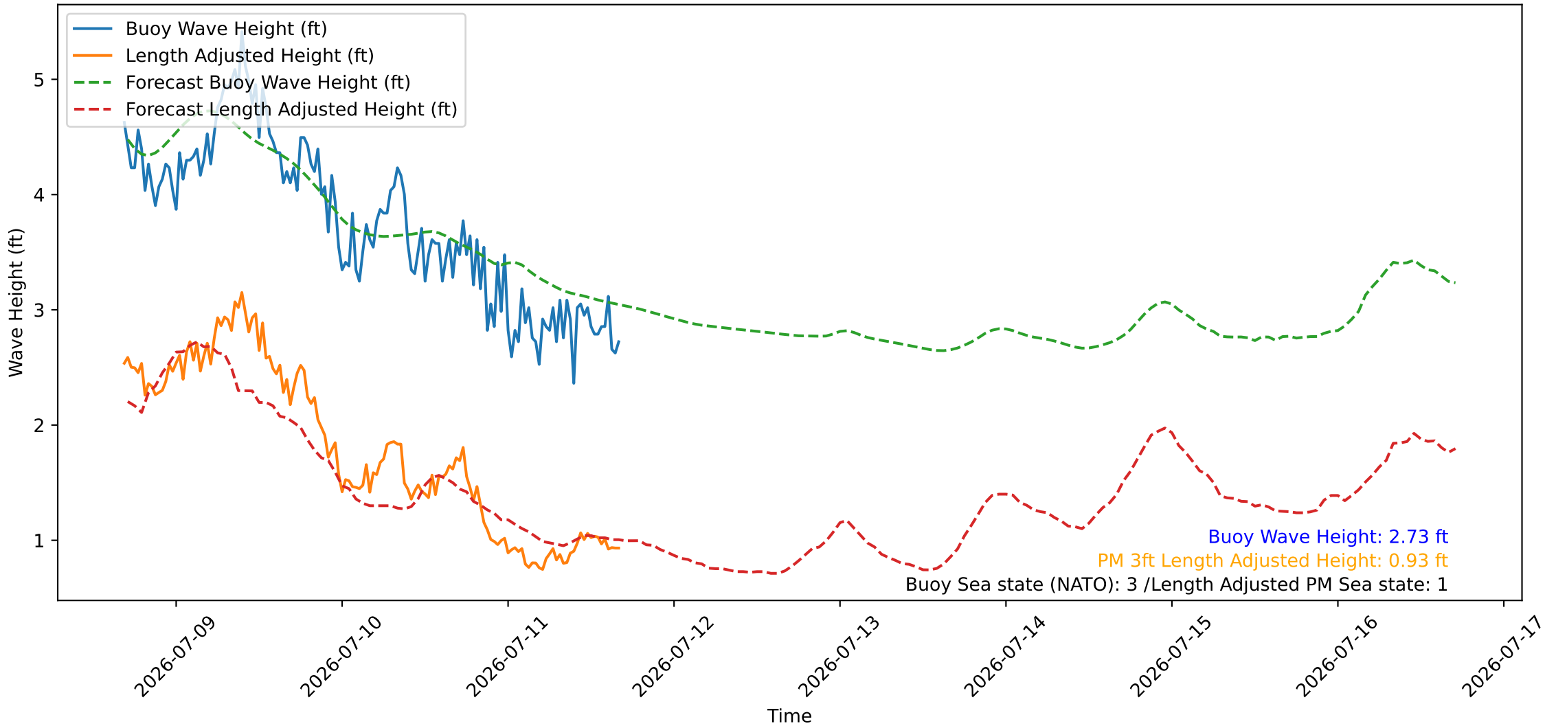
Wave Heights over Time for Oceanside Harbor at 2026-07-11 16:30:26
