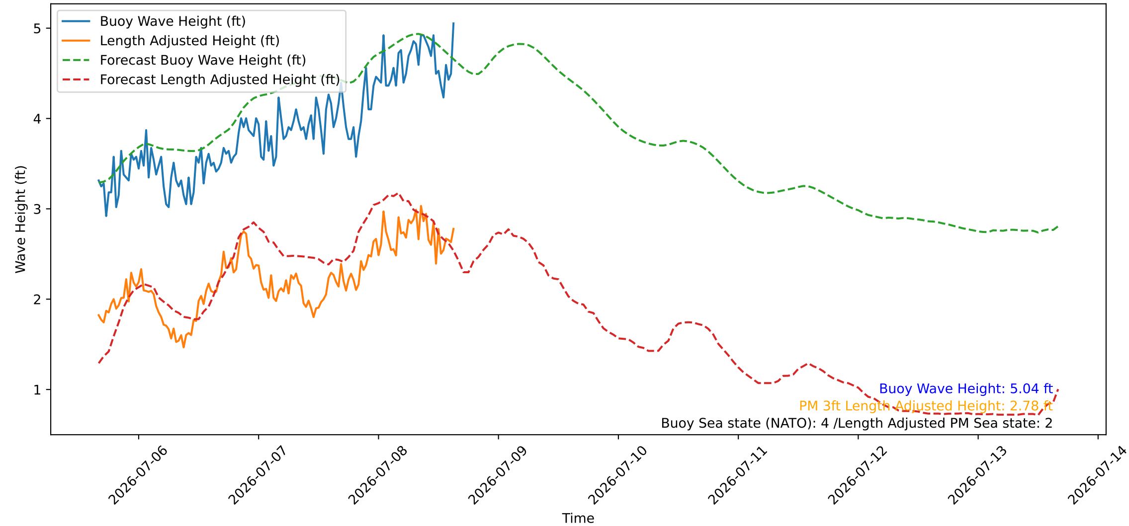
Wave Heights over Time for Oceanside Harbor at 2026-07-08 16:00:26
