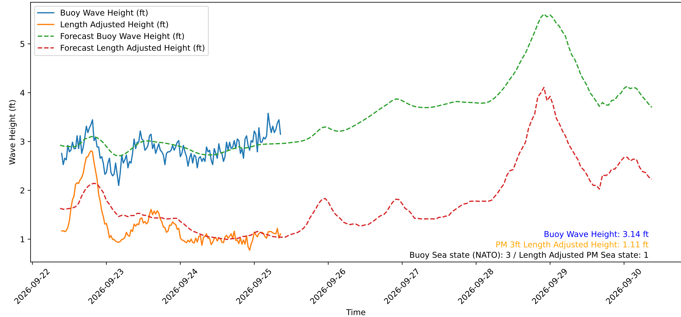
Wave Heights over Time for Green Beach at 2026-09-25 09:11:12
