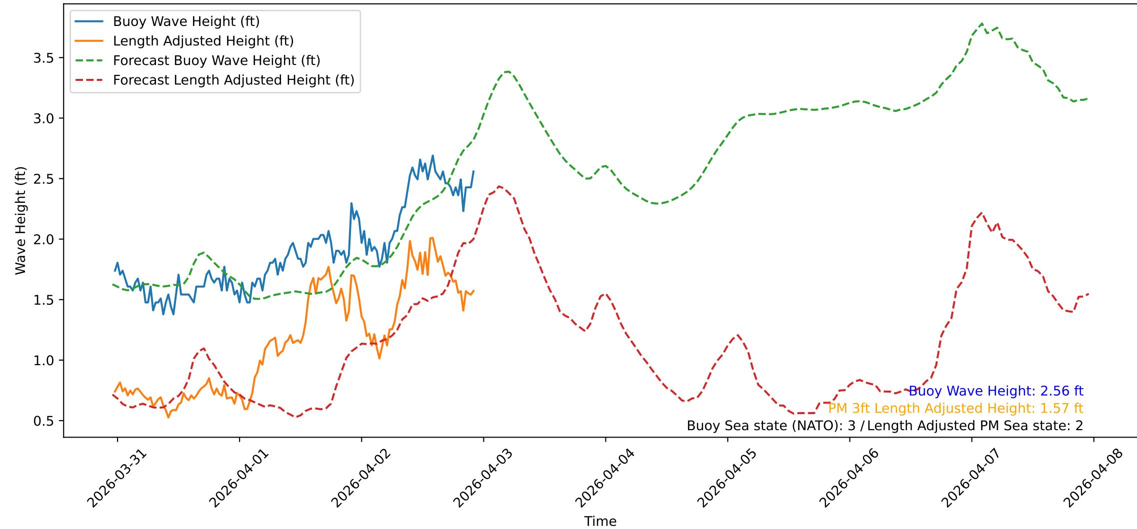
Wave Heights over Time for Red Beach at 2026-04-02 23:00:47
