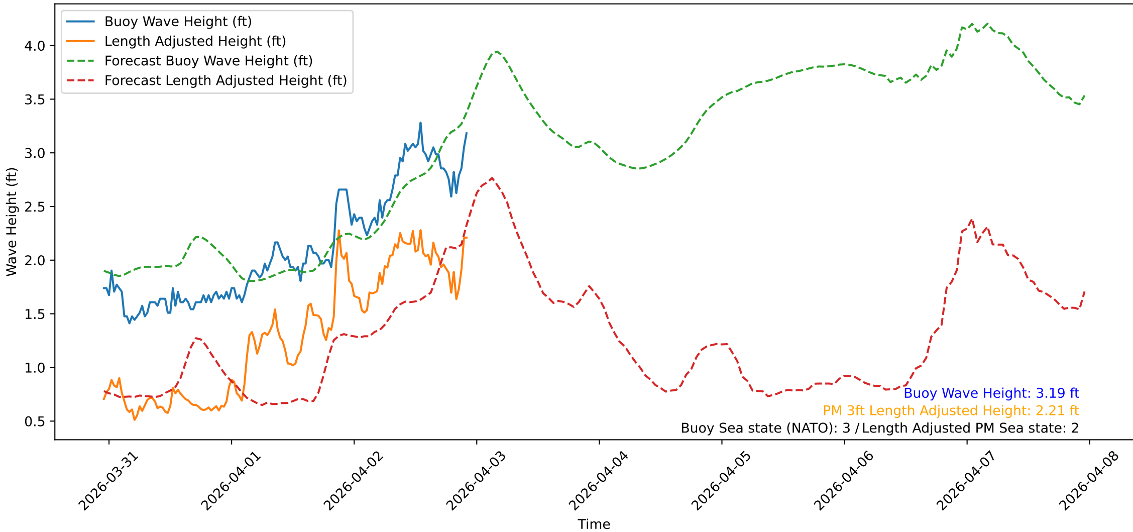
Wave Heights over Time for Green Beach at 2026-04-02 23:01:09
