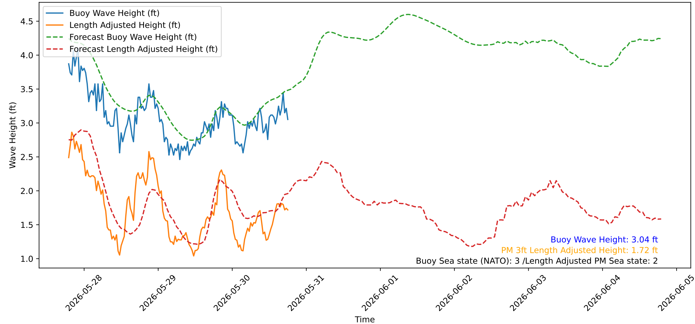
Wave Heights over Time for Green Beach at 2026-05-30 18:51:07
