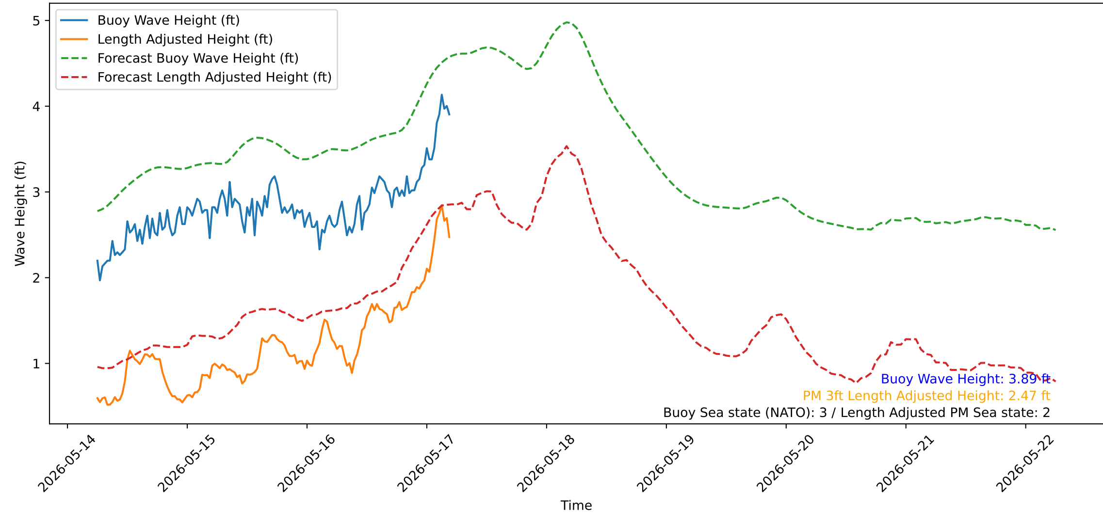
Wave Heights over Time for Red Beach at 2026-05-17 05:30:52
