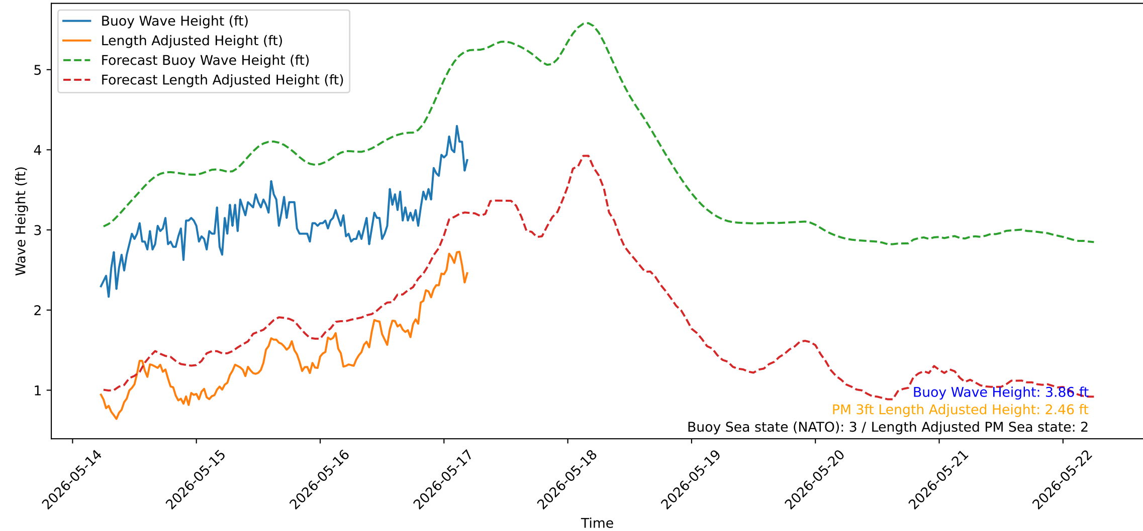
Wave Heights over Time for Oceanside Harbor at 2026-05-17 05:30:32
