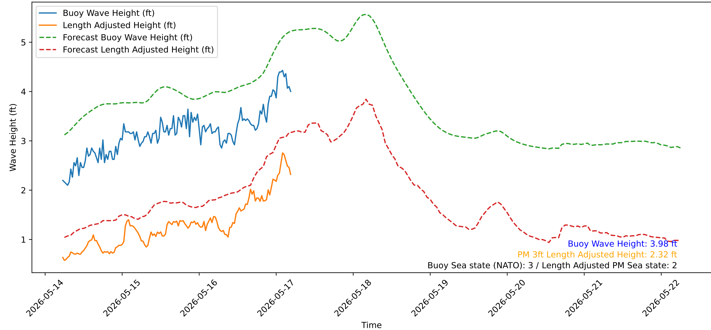
Wave Heights over Time for Green Beach at 2026-05-17 05:31:14
