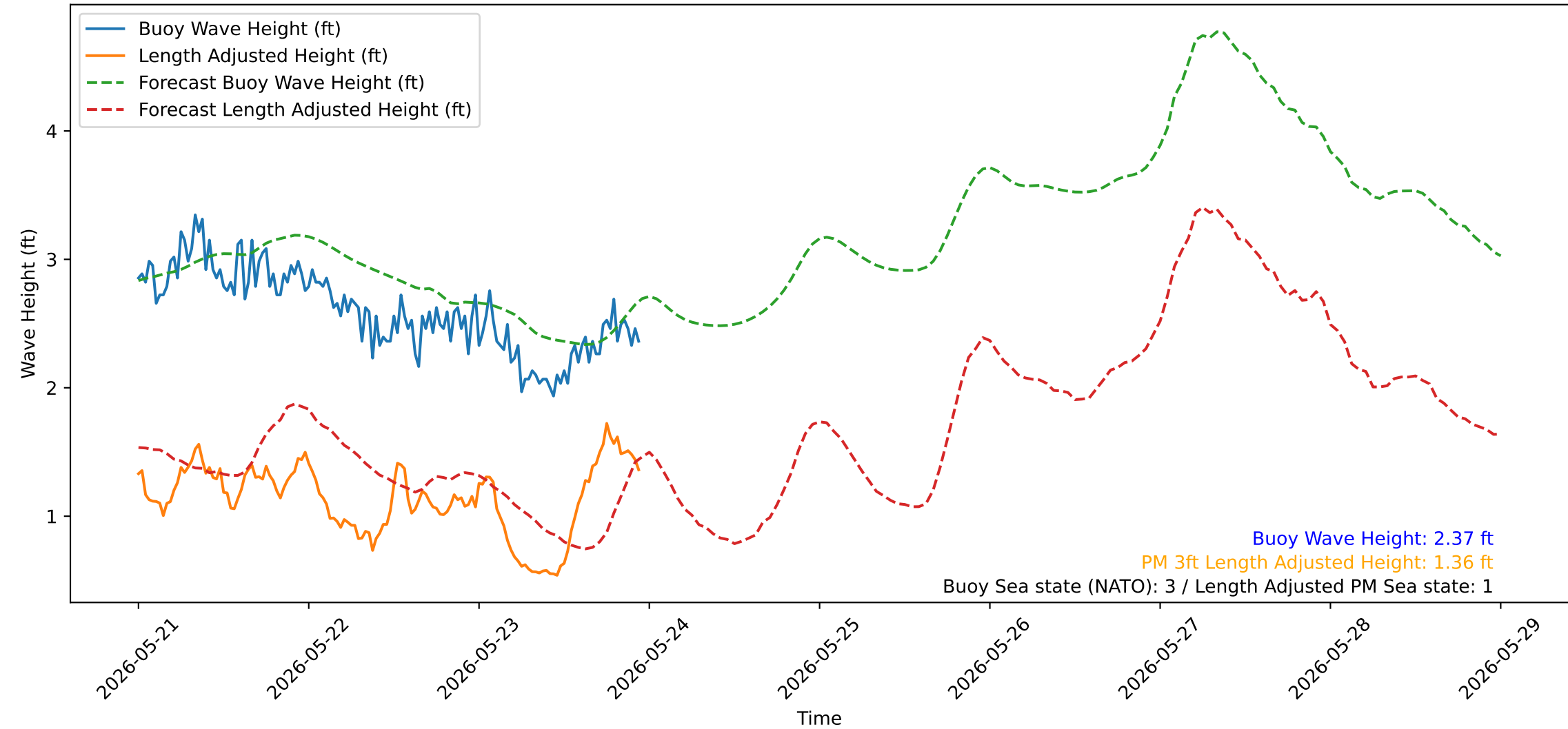
Wave Heights over Time for Red Beach at 2026-05-23 23:30:50
