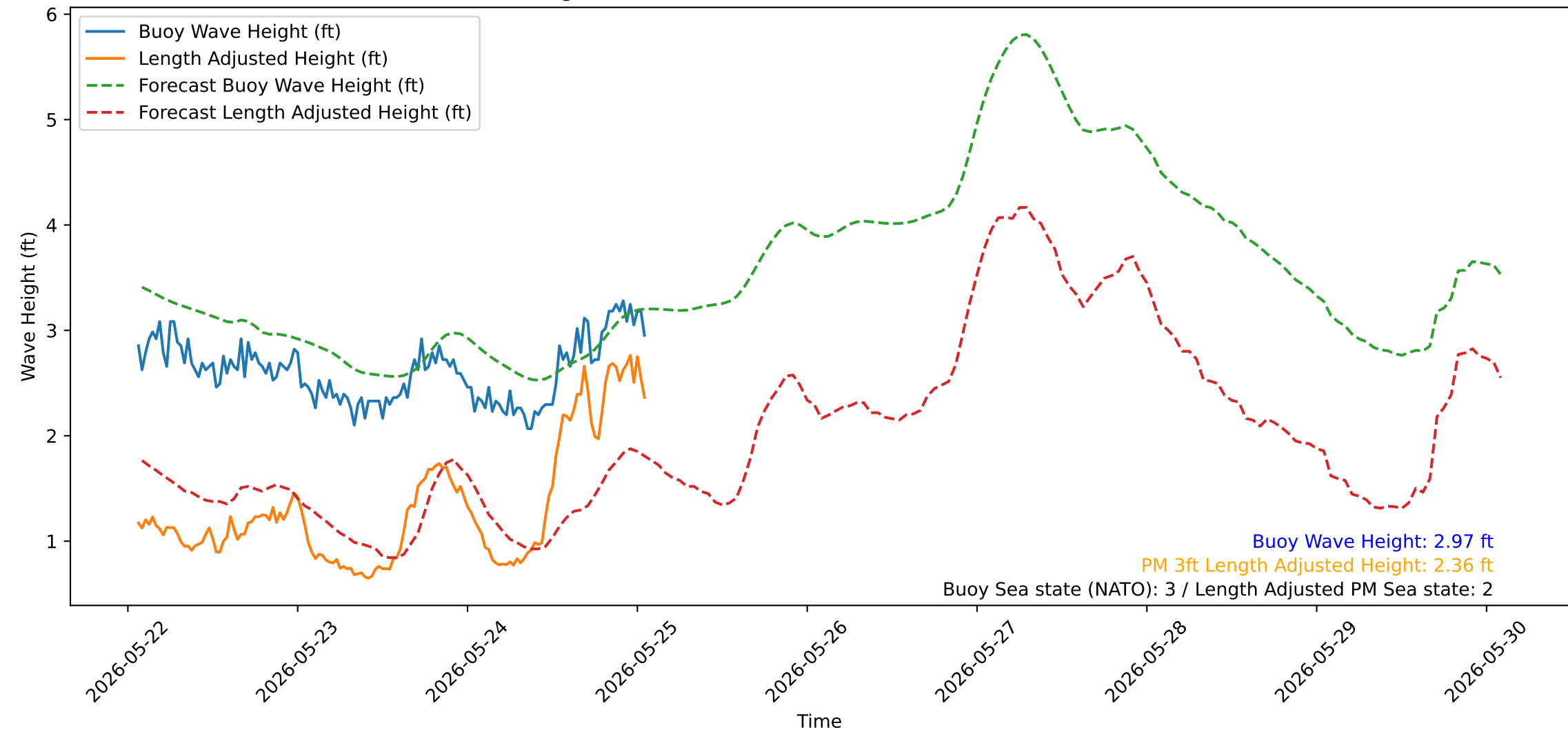
Wave Heights over Time for Green Beach at 2026-05-25 01:41:13
