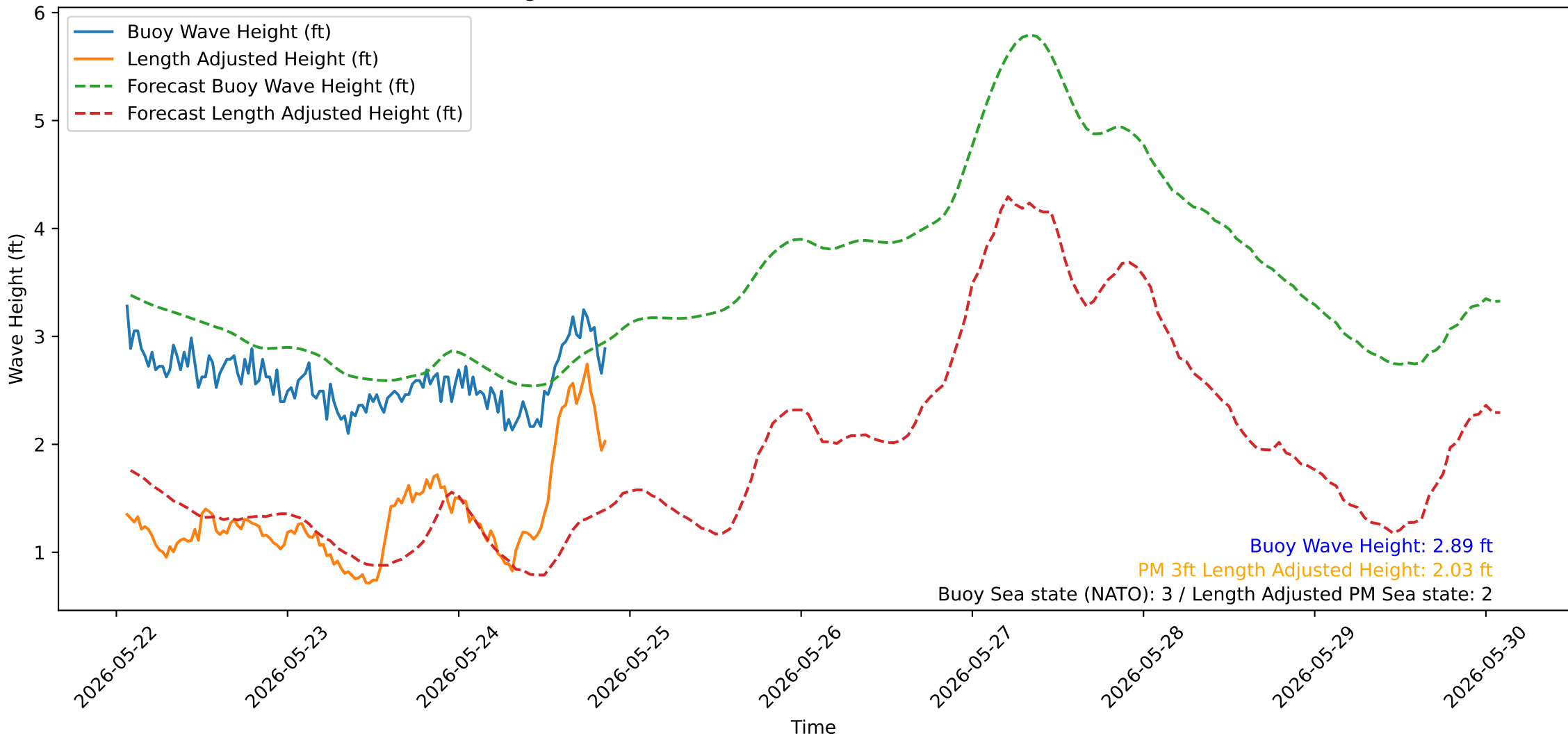
Wave Heights over Time for Oceanside Harbor at 2026-05-25 01:40:31
