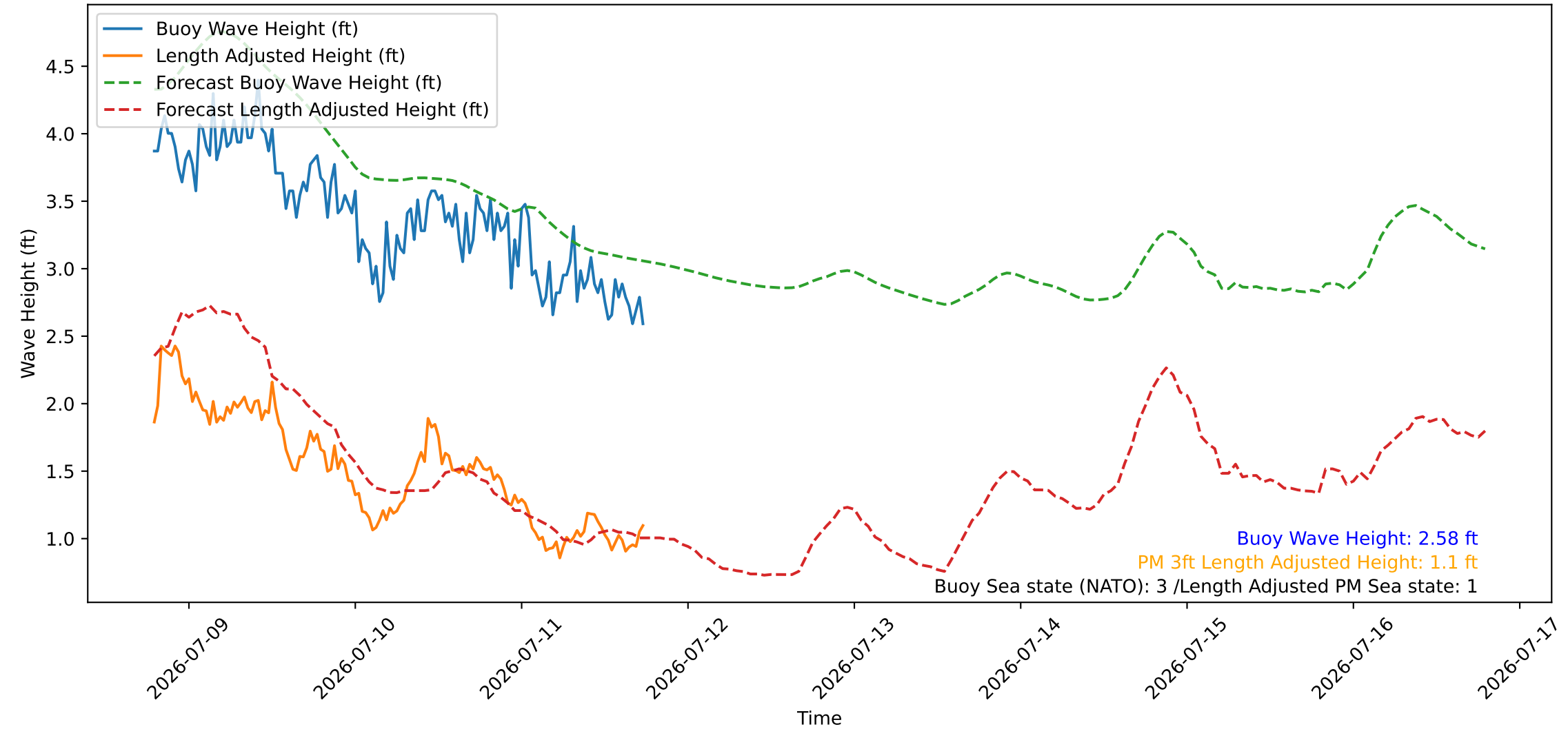
Wave Heights over Time for Green Beach at 2026-07-11 18:51:10
