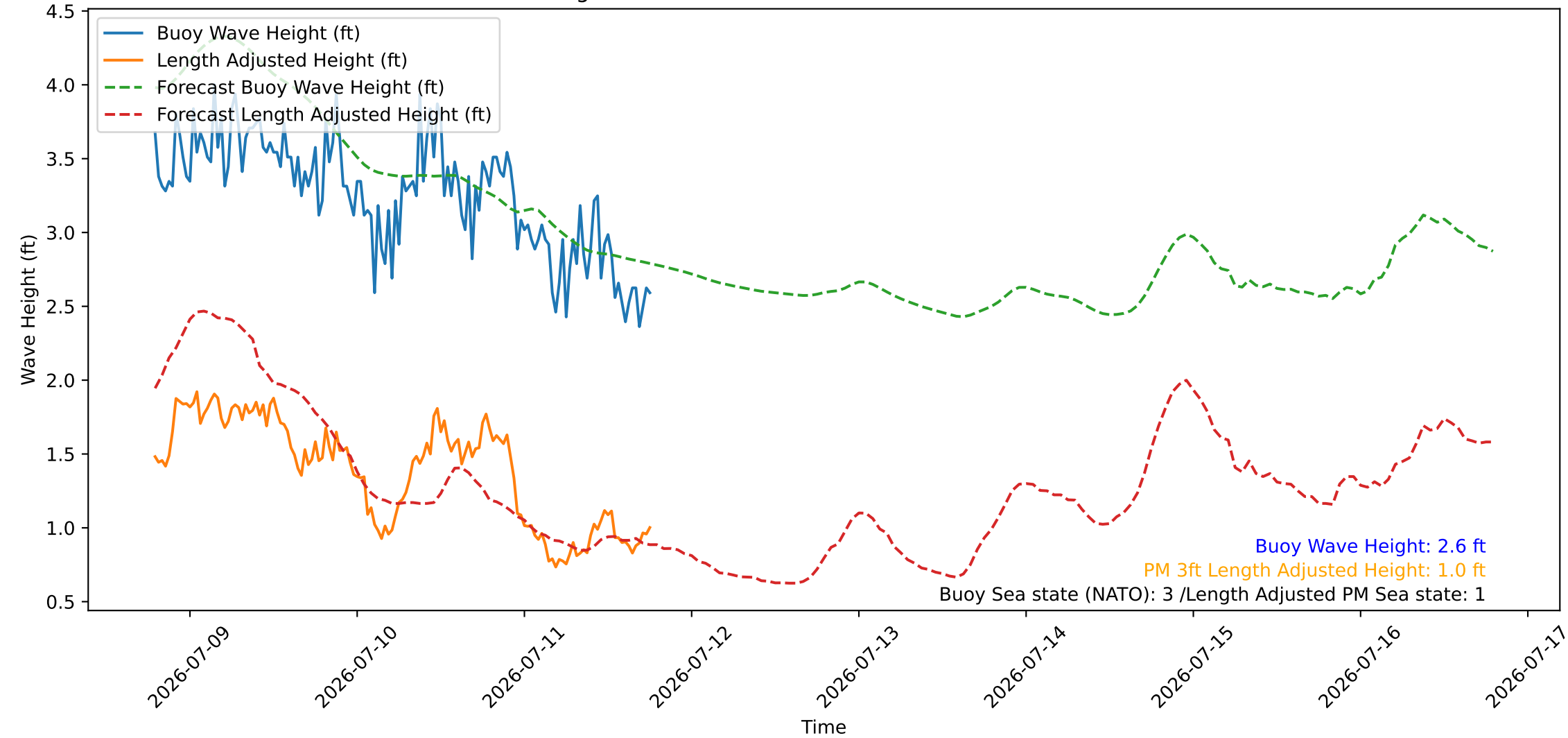
Wave Heights over Time for Red Beach at 2026-07-11 18:50:47
