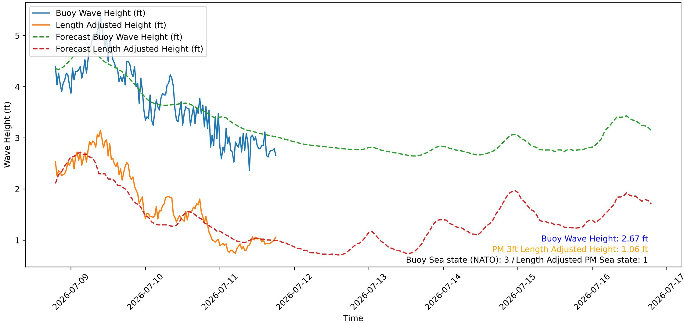
Wave Heights over Time for Oceanside Harbor at 2026-07-11 18:50:26
