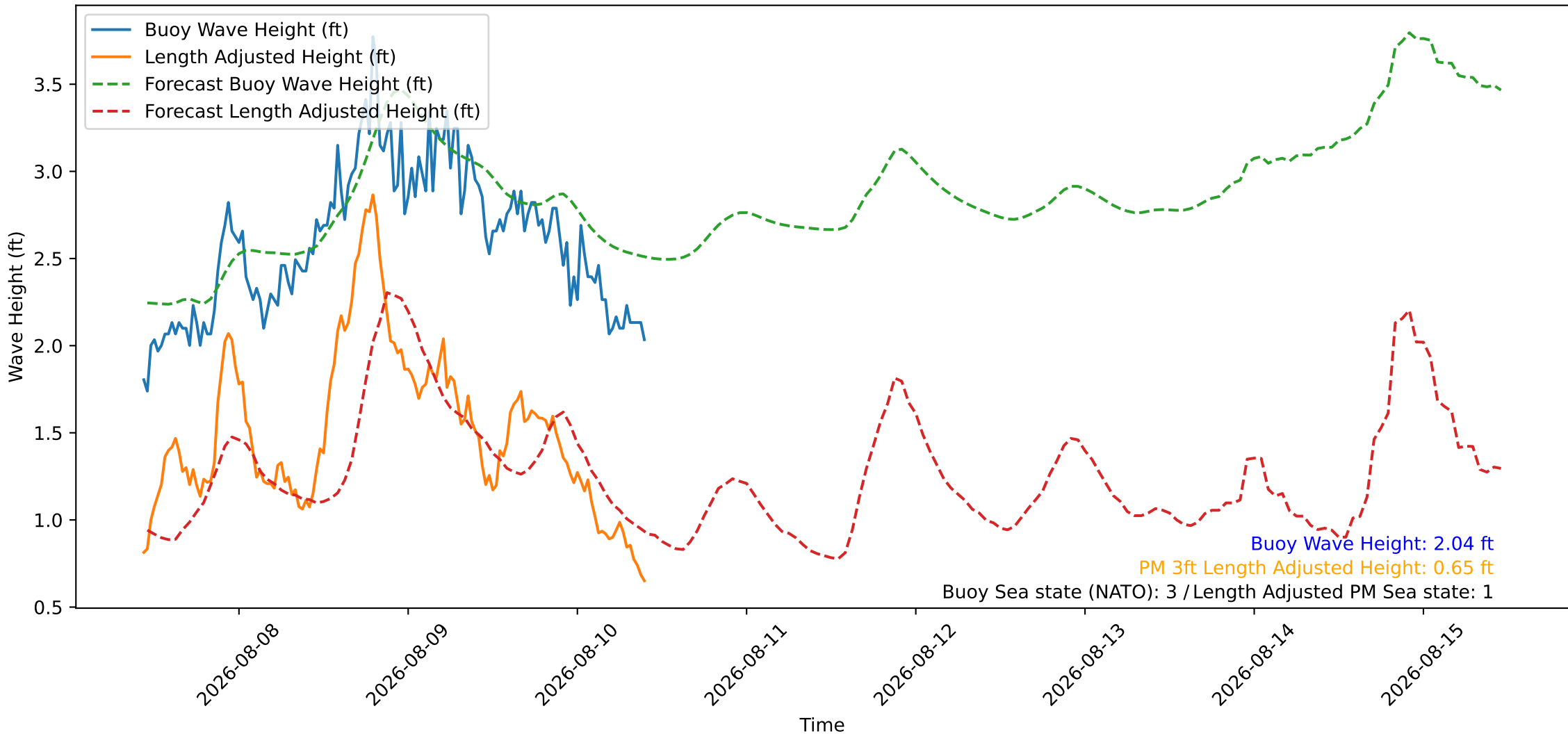
Wave Heights over Time for Green Beach at 2026-08-10 10:31:09
