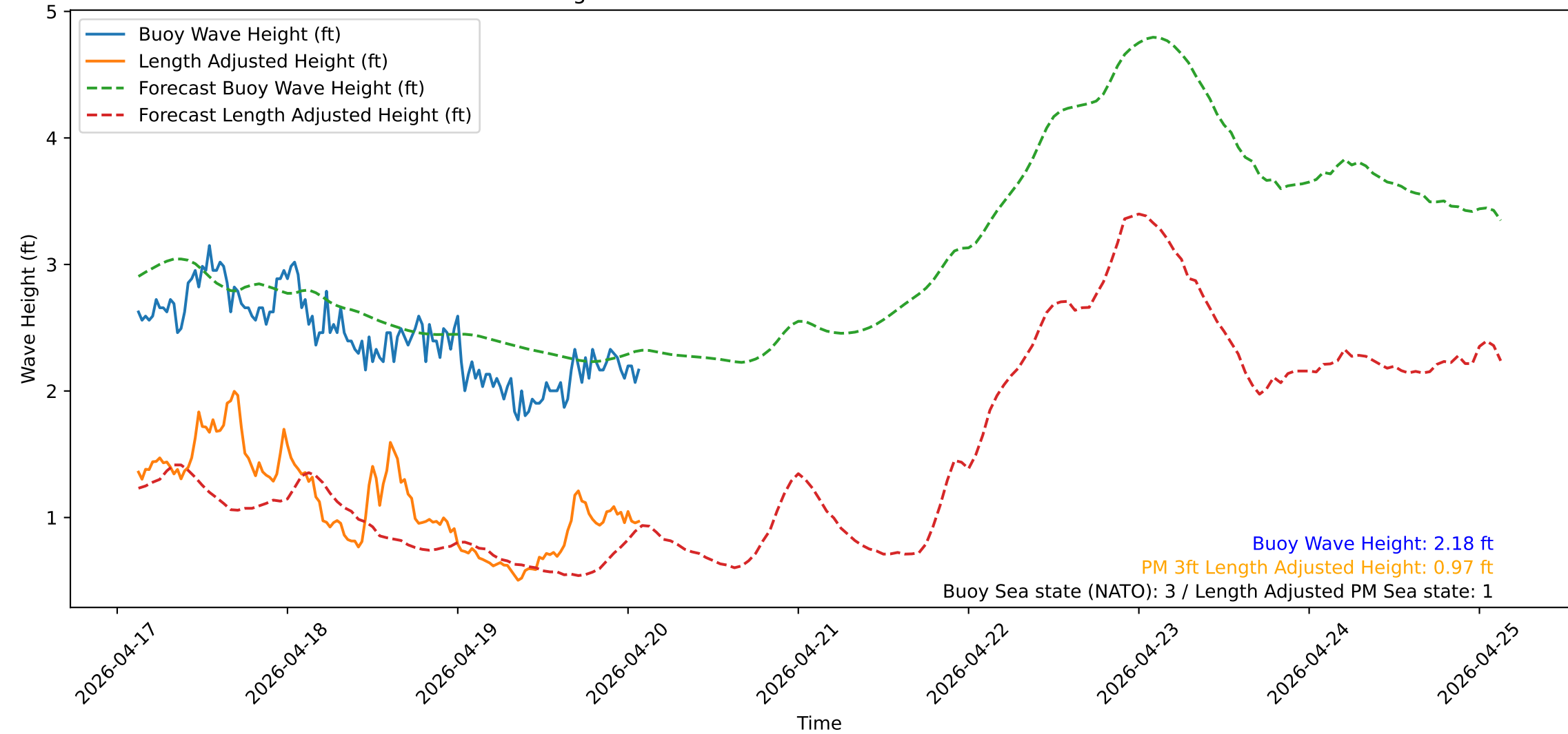
Wave Heights over Time for Red Beach at 2026-04-20 02:30:55
