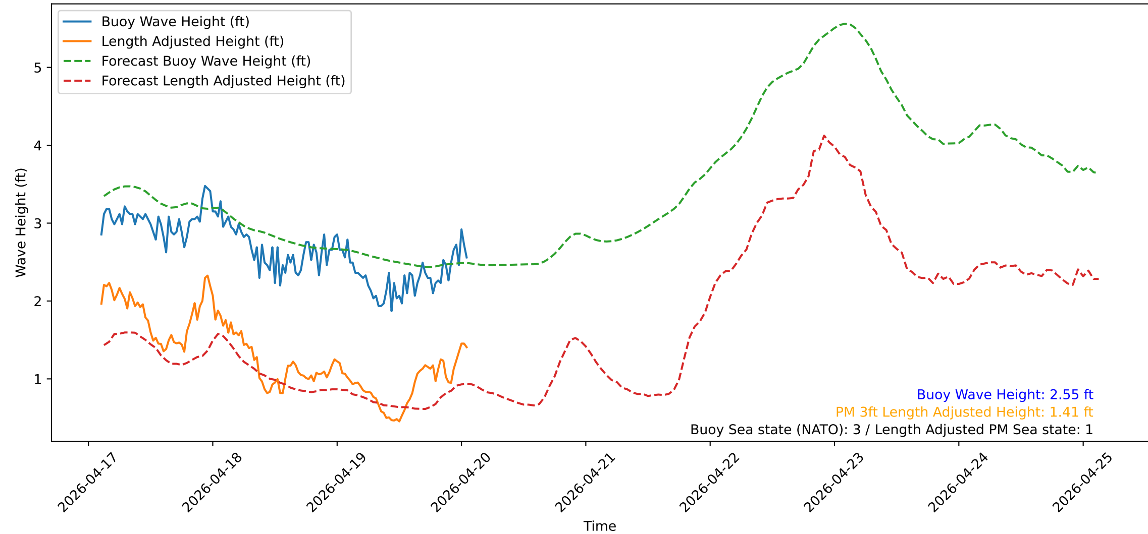
Wave Heights over Time for Green Beach at 2026-04-20 02:31:19
