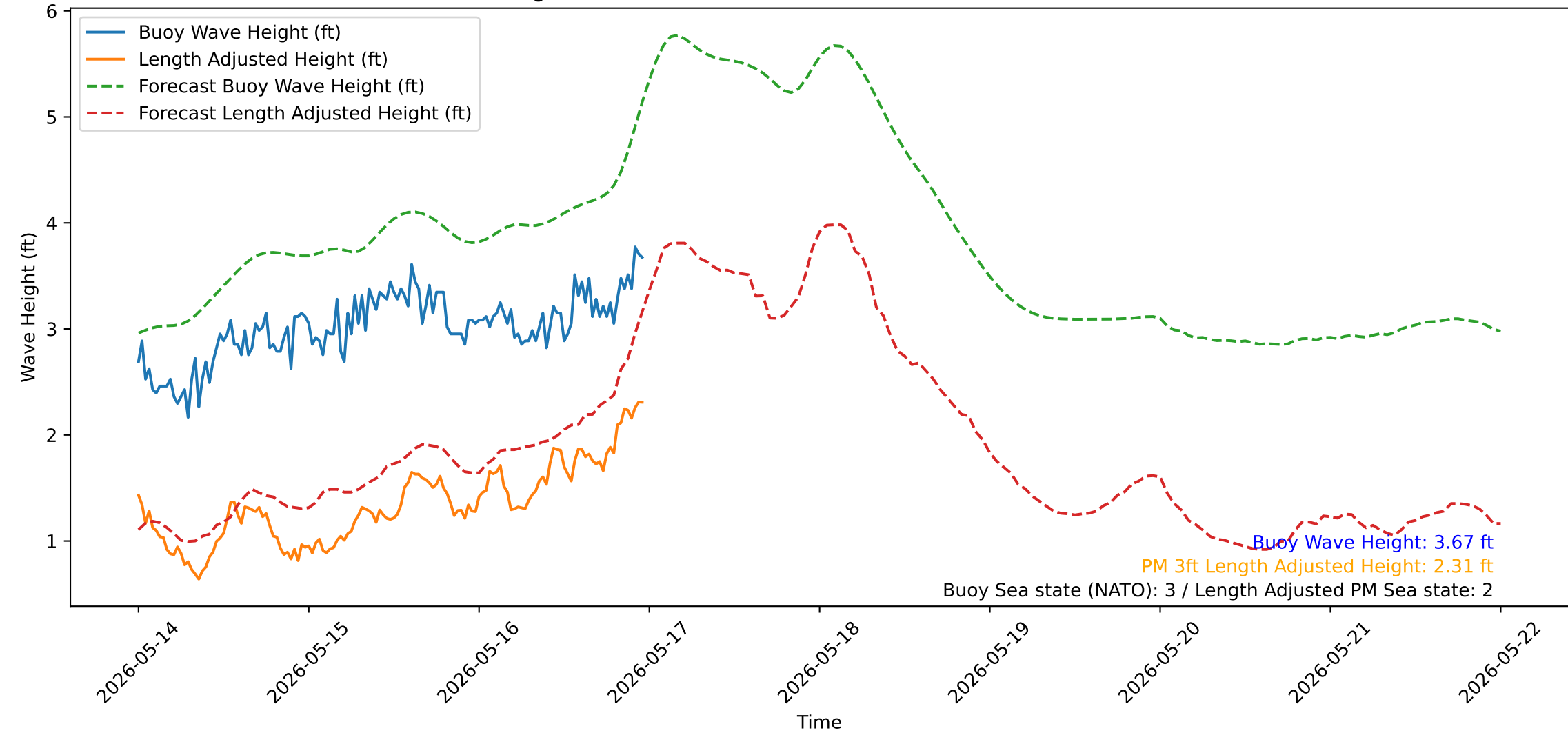
Wave Heights over Time for Oceanside Harbor at 2026-05-16 23:50:31
