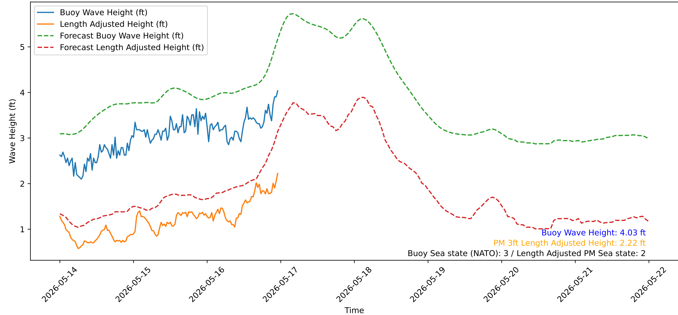
Wave Heights over Time for Green Beach at 2026-05-16 23:51:14
