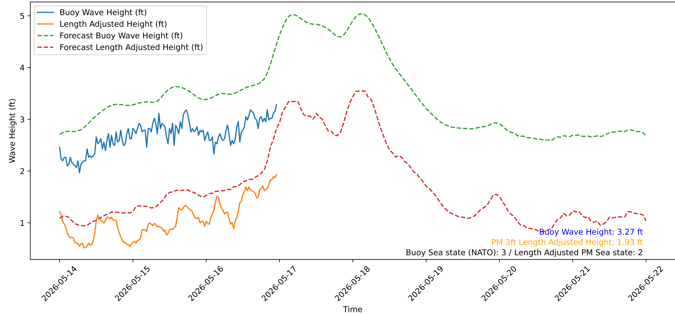
Wave Heights over Time for Red Beach at 2026-05-16 23:50:52
