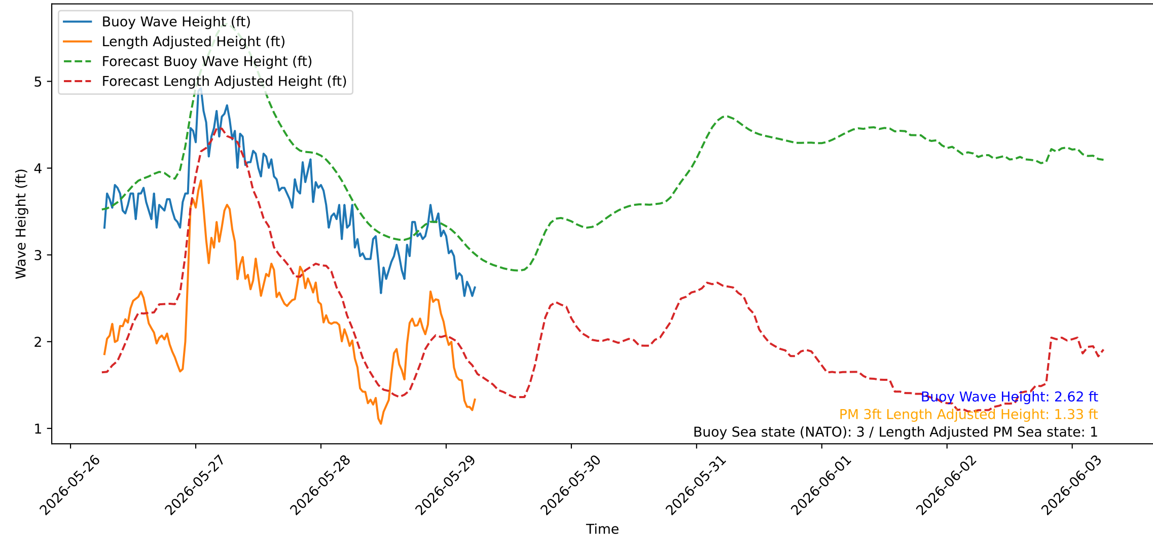
Wave Heights over Time for Green Beach at 2026-05-29 06:21:04
