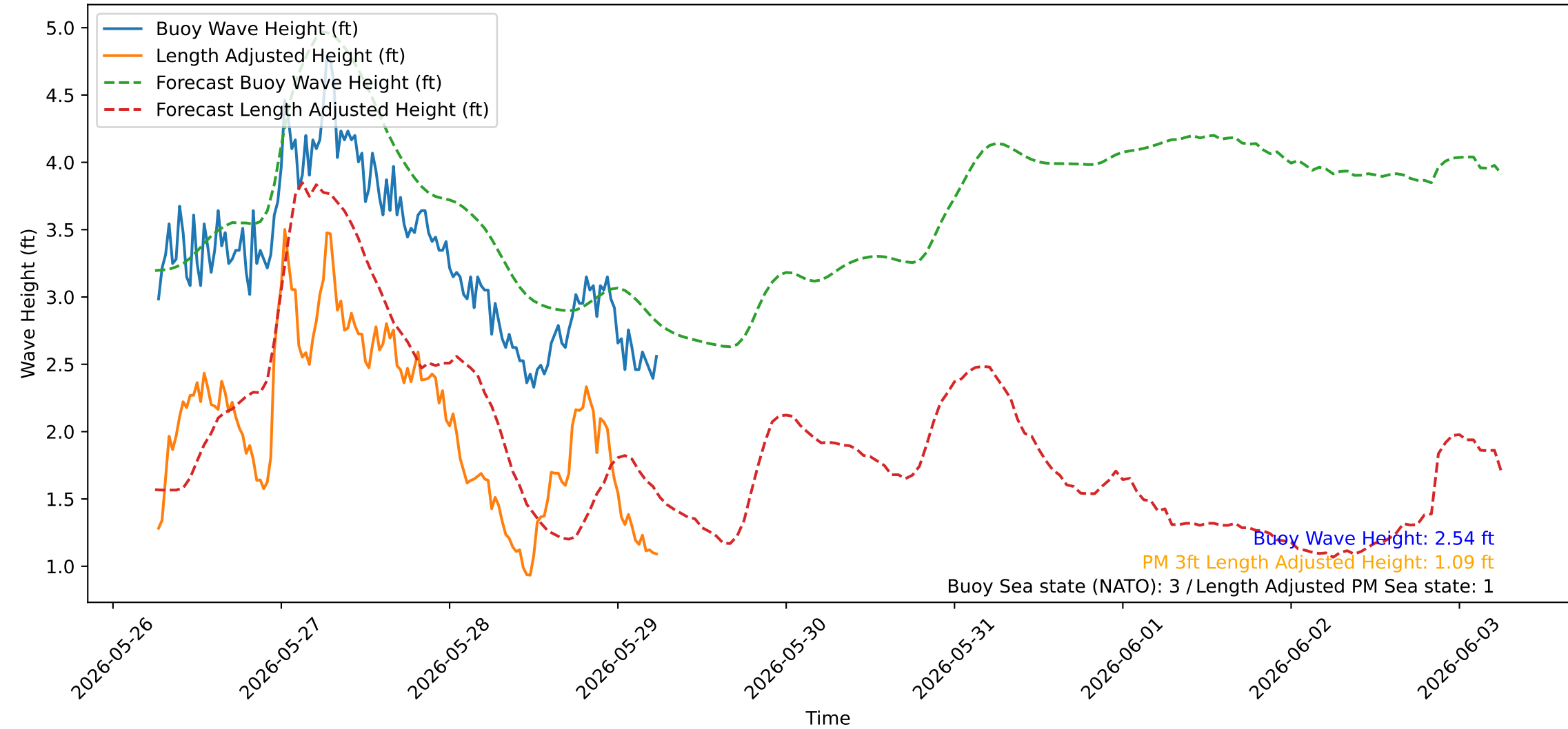
Wave Heights over Time for Red Beach at 2026-05-29 06:20:41
