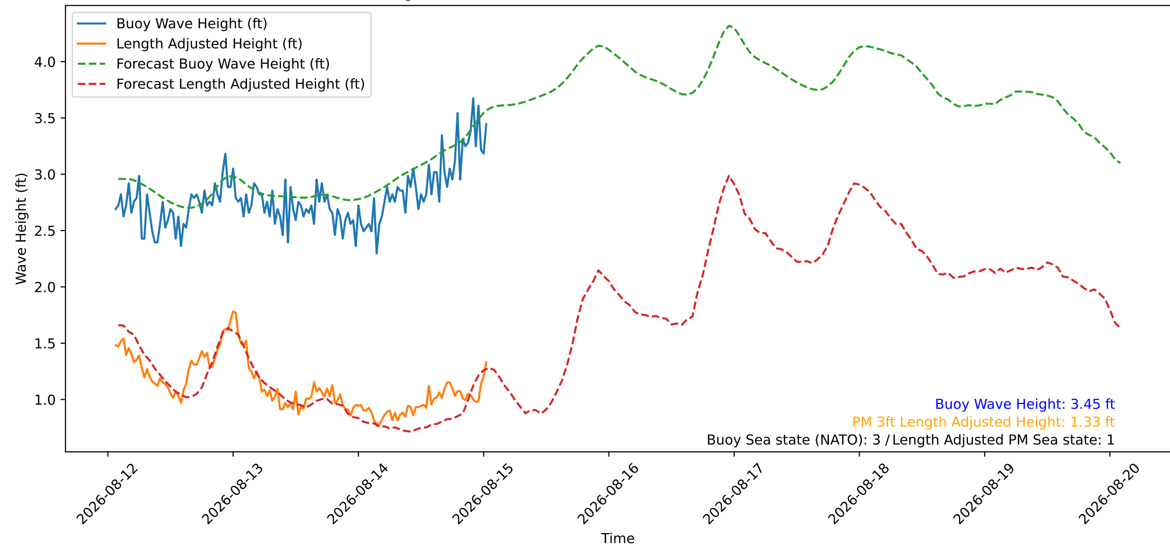
Wave Heights over Time for Oceanside Harbor at 2026-08-15 01:30:26
