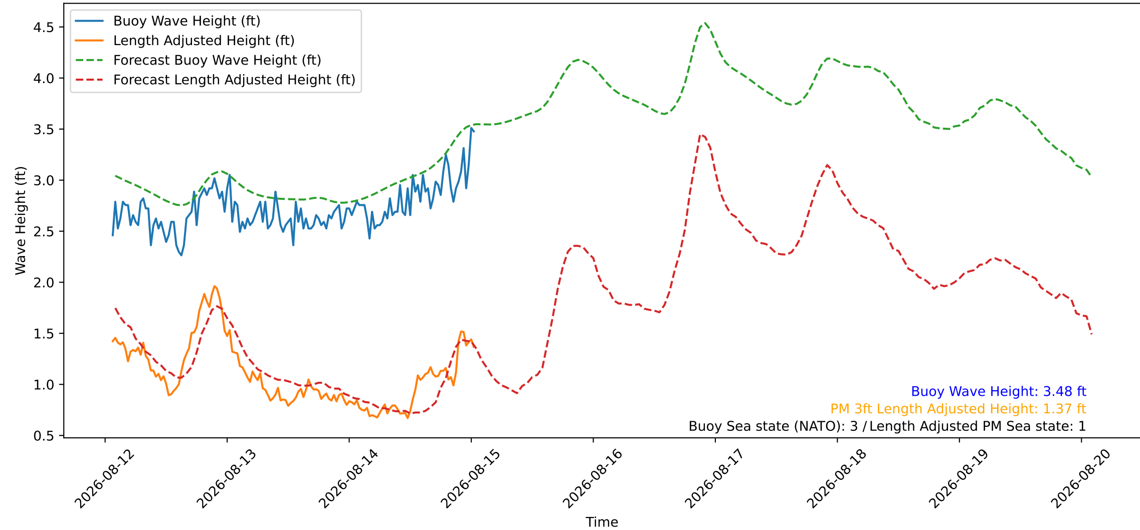
Wave Heights over Time for Green Beach at 2026-08-15 01:31:08
