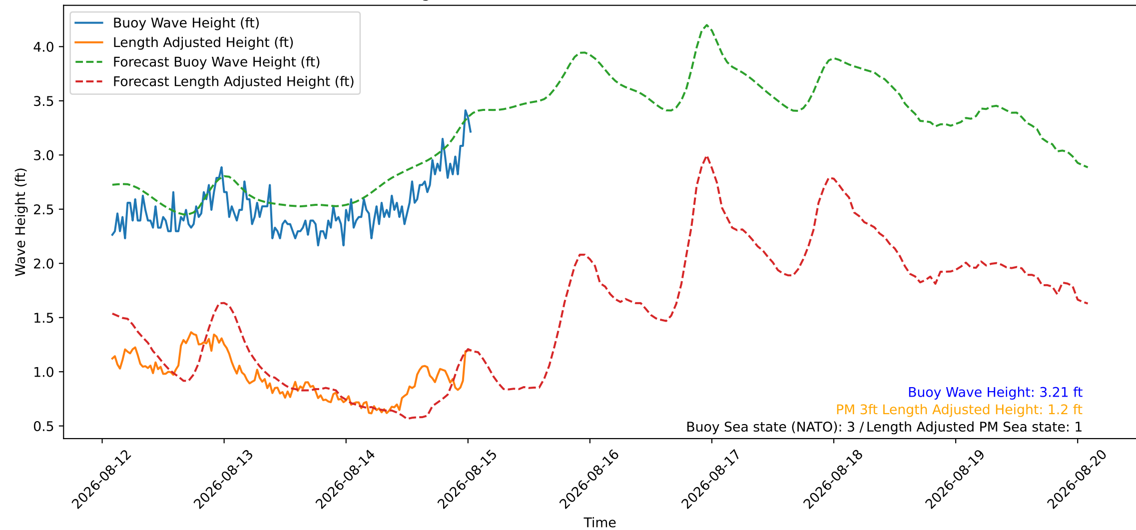
Wave Heights over Time for Red Beach at 2026-08-15 01:30:46
