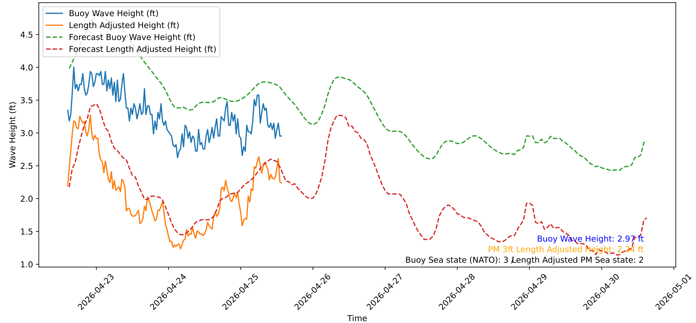
Wave Heights over Time for Green Beach at 2026-04-25 14:31:13
