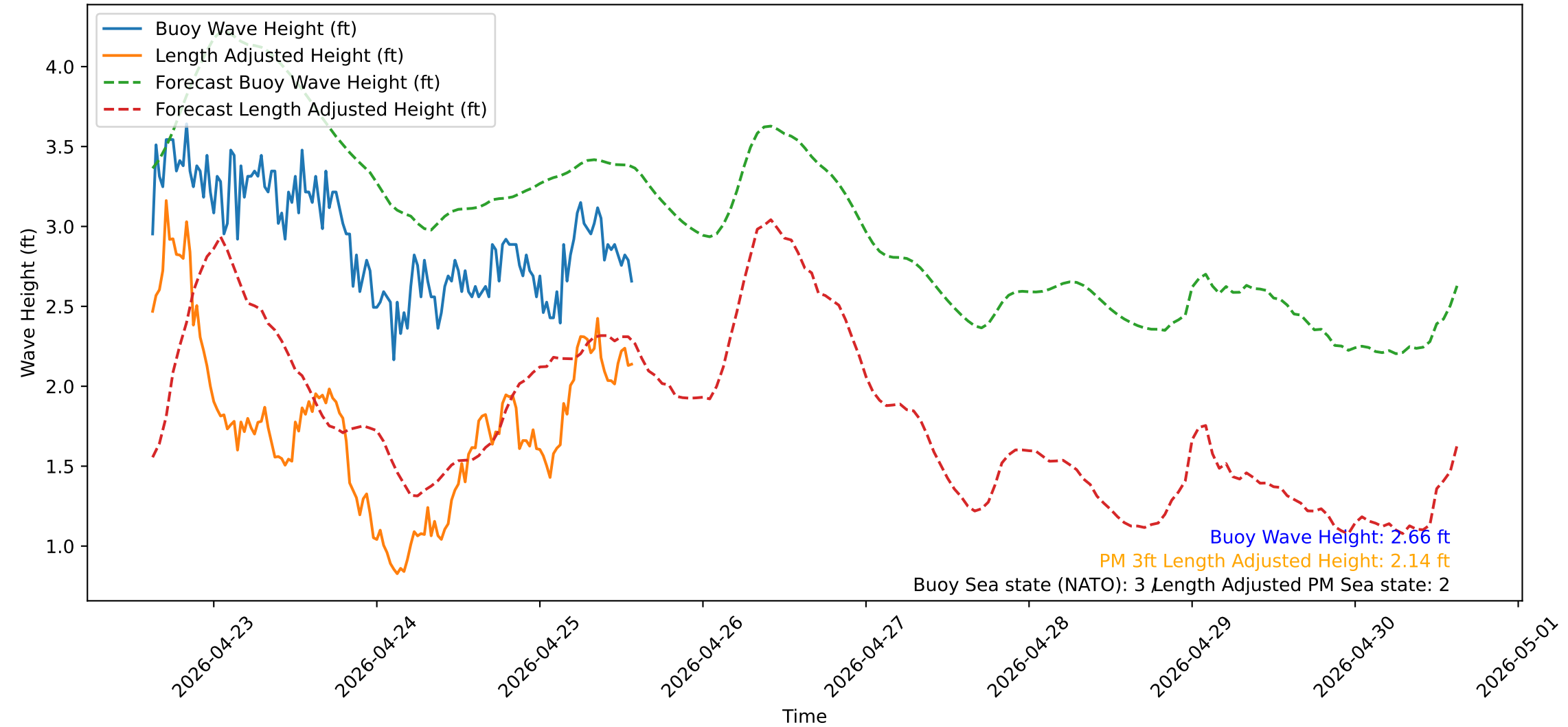
Wave Heights over Time for Red Beach at 2026-04-25 14:30:51
