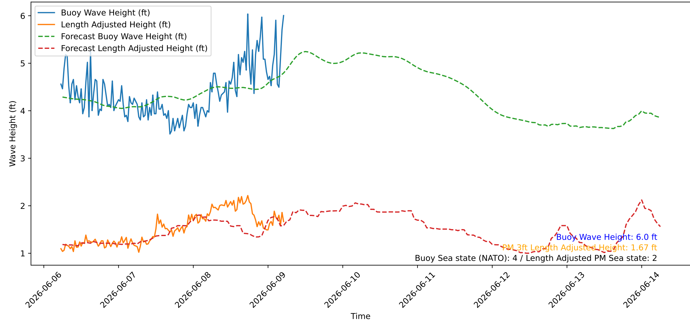
Wave Heights over Time for Oceanside Harbor at 2026-06-09 05:40:26
