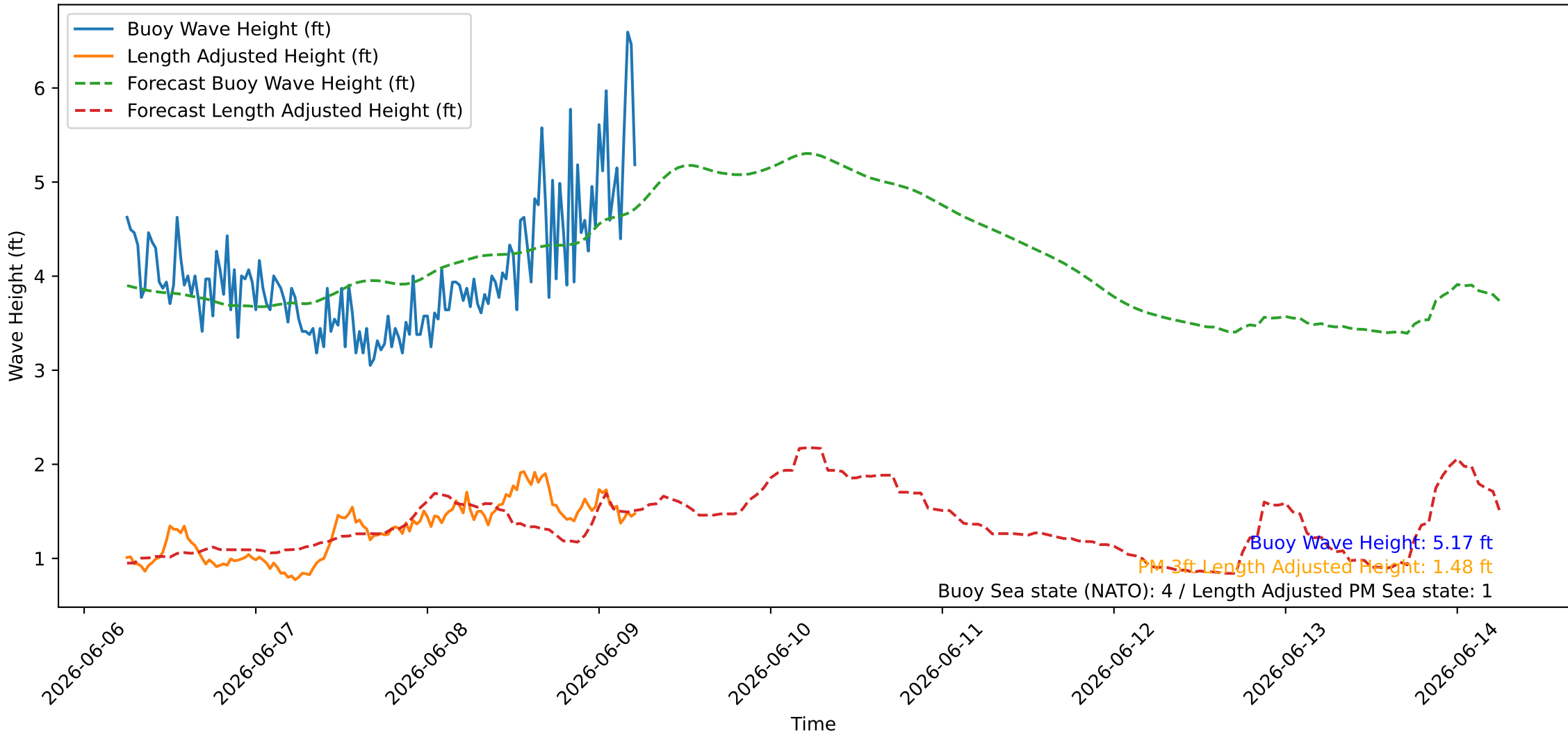
Wave Heights over Time for Red Beach at 2026-06-09 05:40:46
