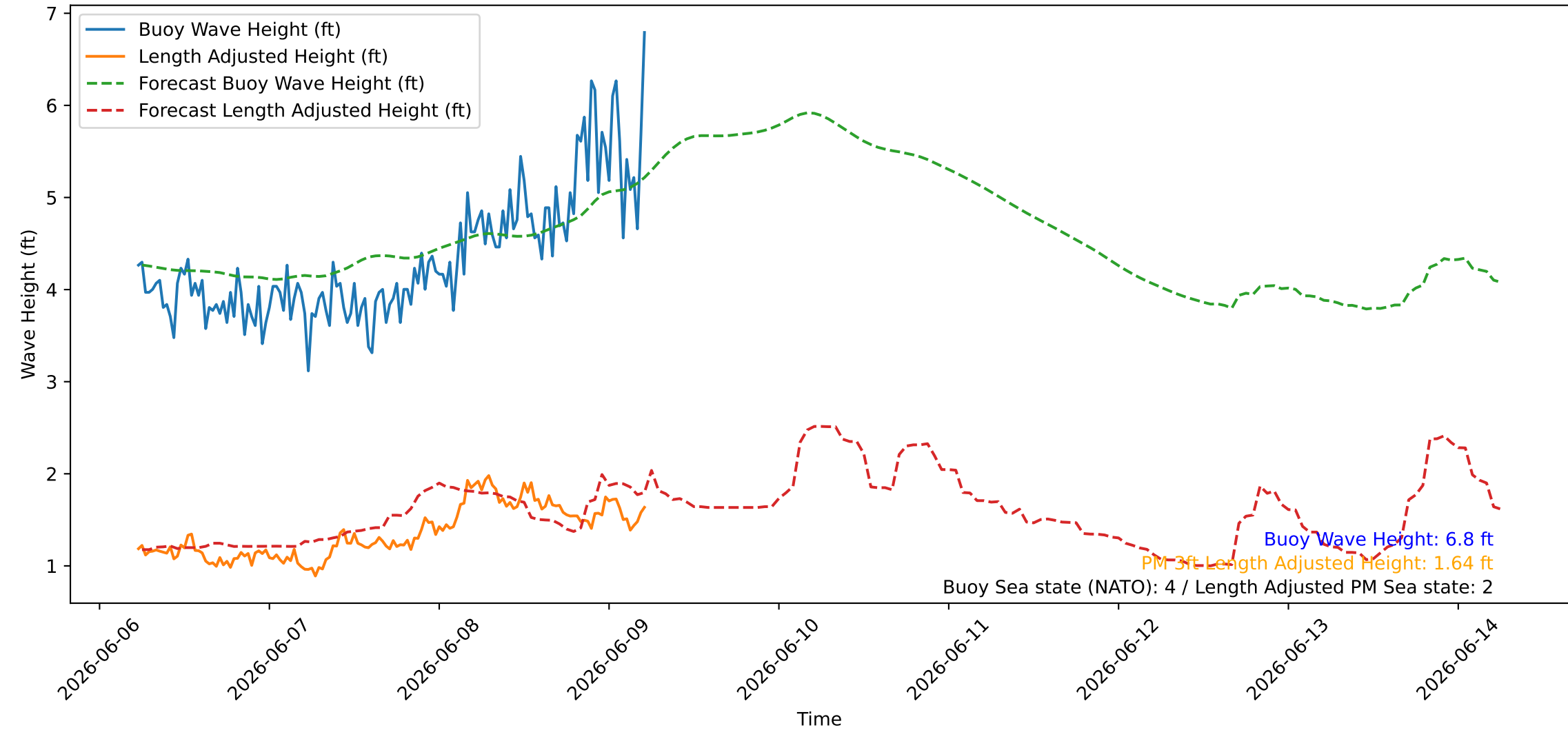
Wave Heights over Time for Green Beach at 2026-06-09 05:41:08
