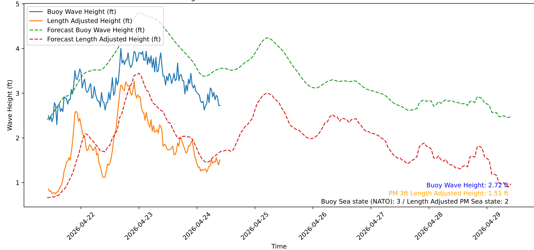
Wave Heights over Time for Green Beach at 2026-04-24 10:21:13
