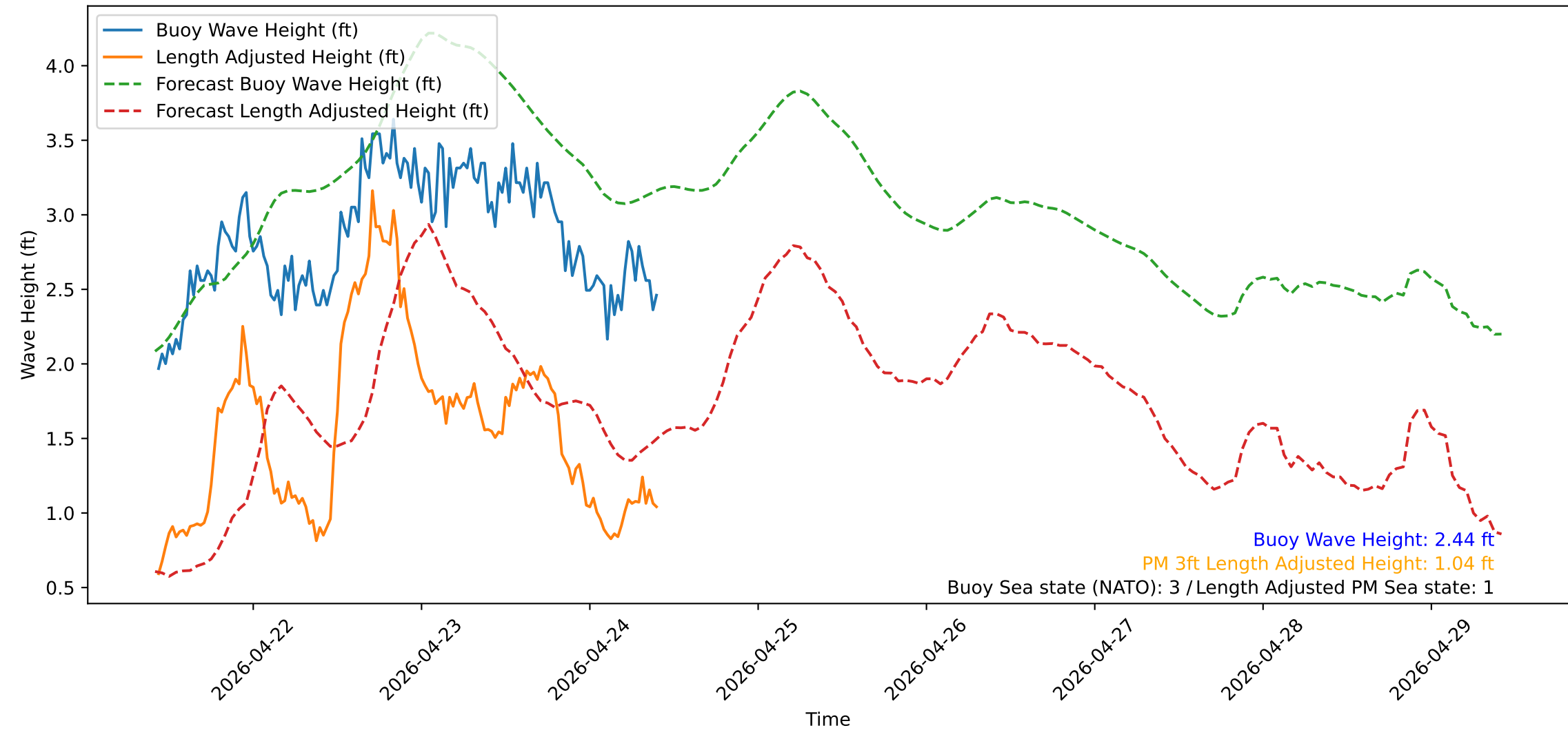
Wave Heights over Time for Red Beach at 2026-04-24 10:20:51
