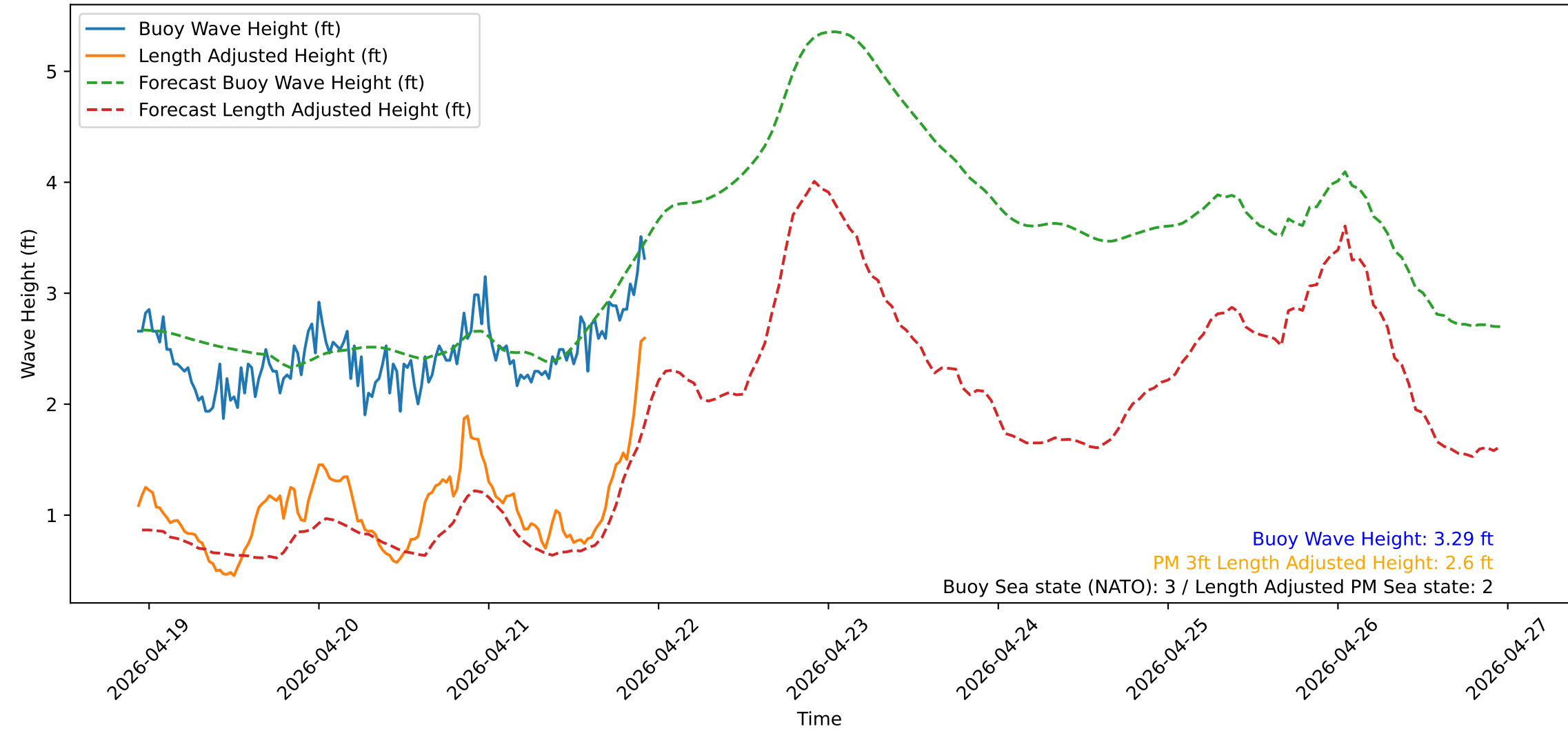
Wave Heights over Time for Green Beach at 2026-04-21 22:41:13
