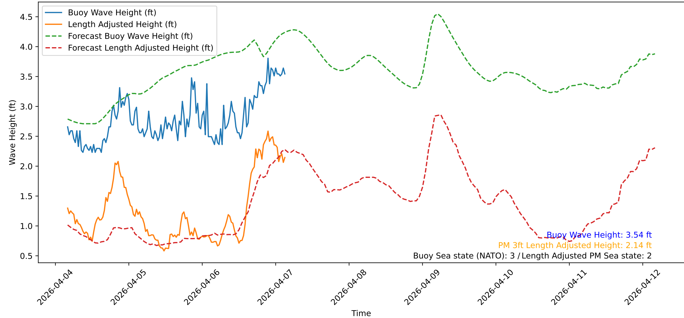
Wave Heights over Time for Green Beach at 2026-04-07 04:01:09
