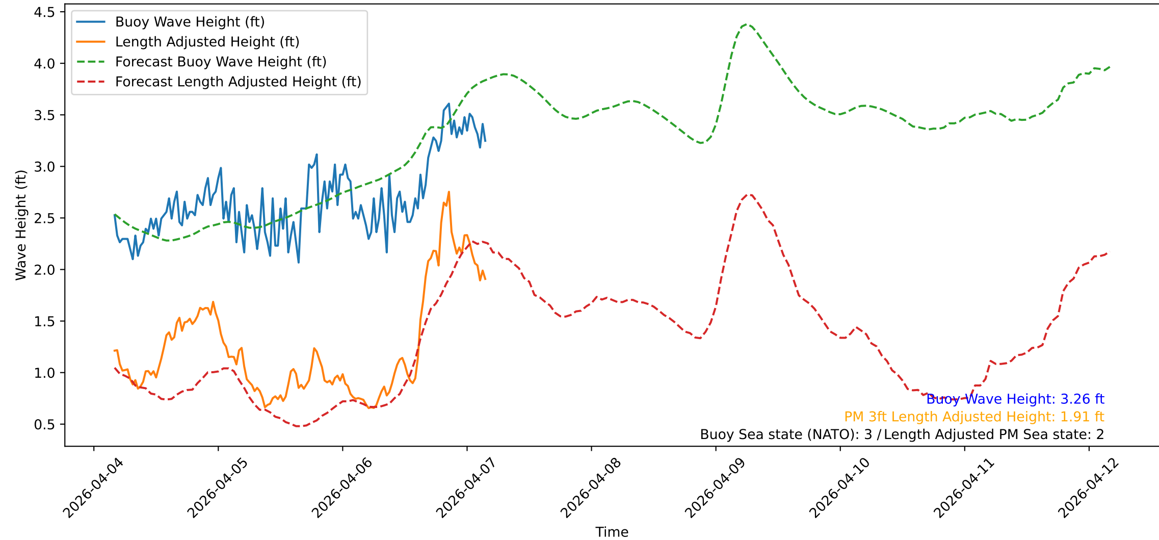
Wave Heights over Time for Oceanside Harbor at 2026-04-07 04:00:31
