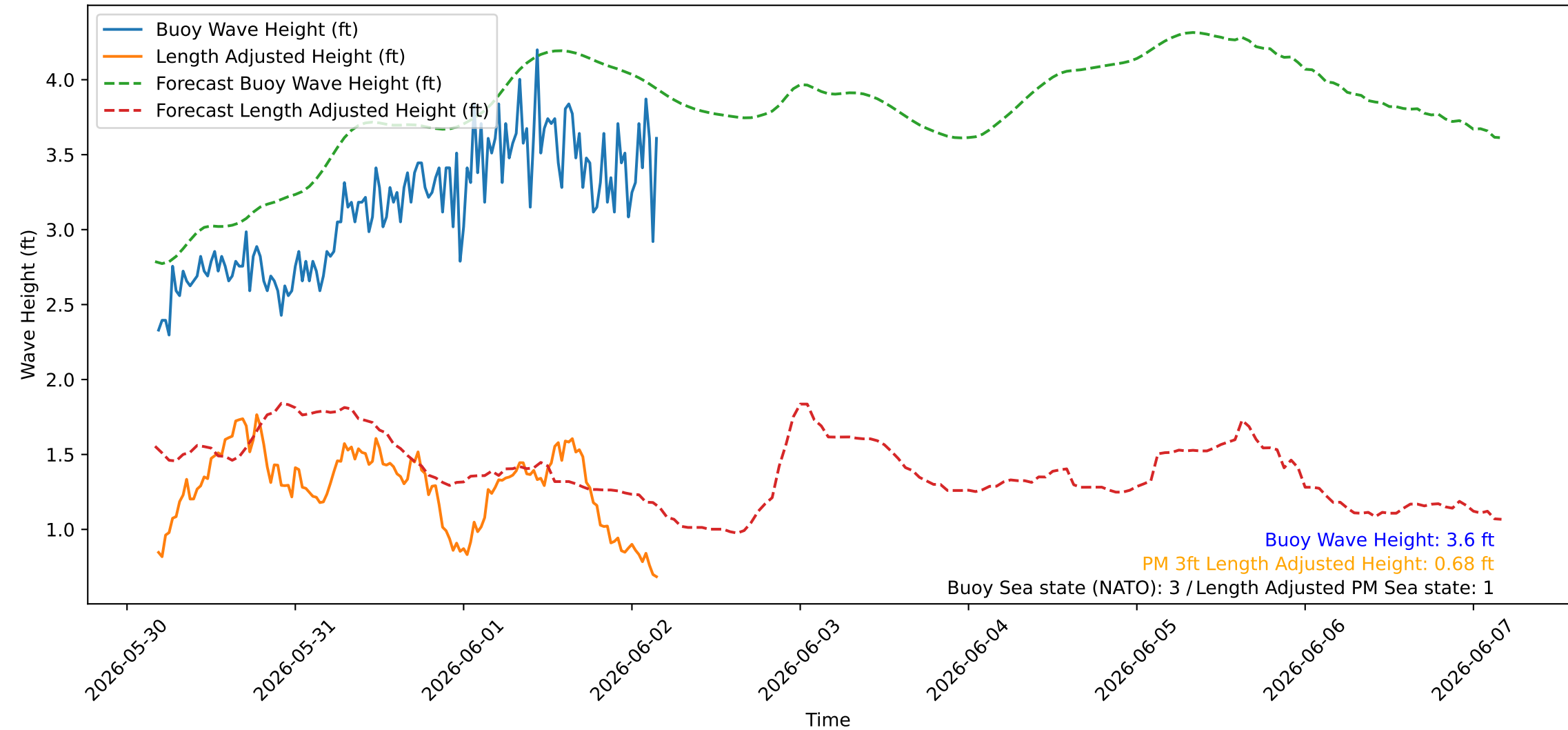
Wave Heights over Time for Red Beach at 2026-06-02 04:20:46
