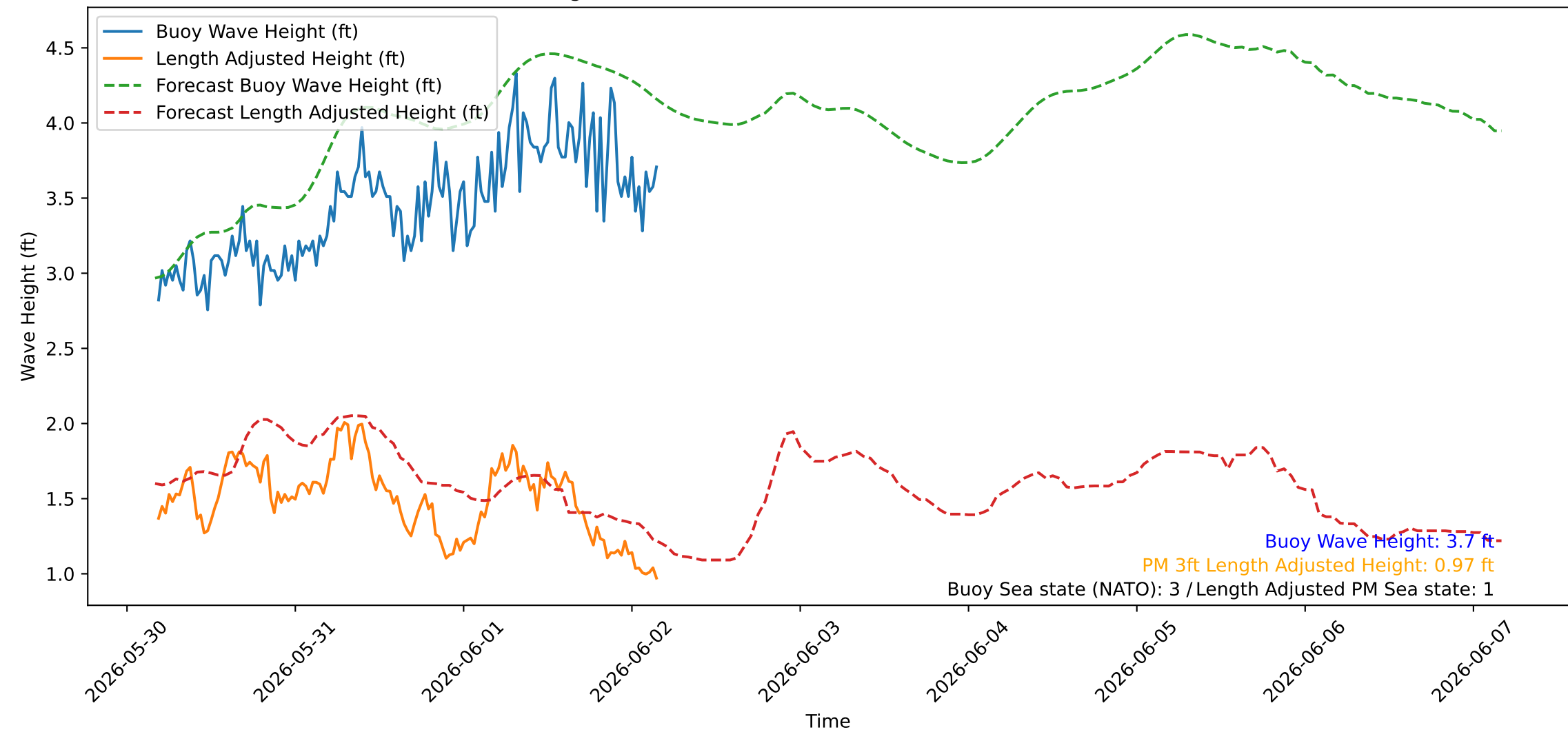
Wave Heights over Time for Green Beach at 2026-06-02 04:21:09
