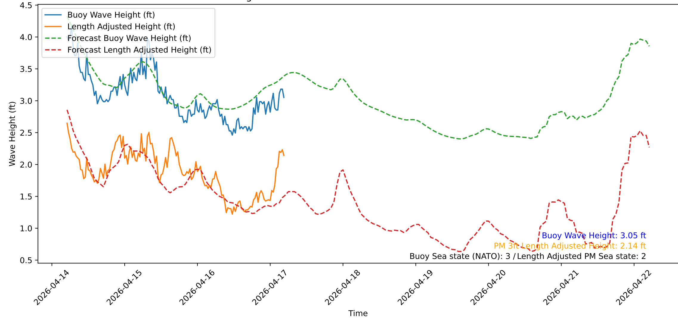
Wave Heights over Time for Green Beach at 2026-04-17 05:11:14
