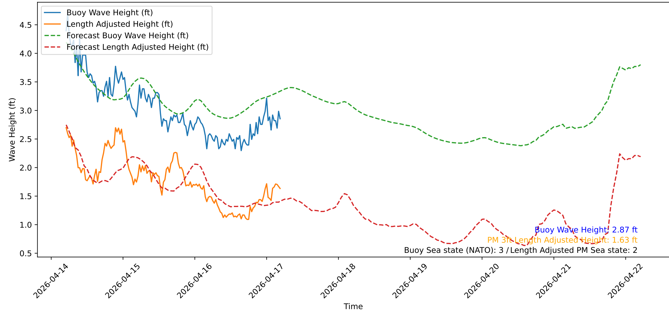
Wave Heights over Time for Oceanside Harbor at 2026-04-17 05:10:32
