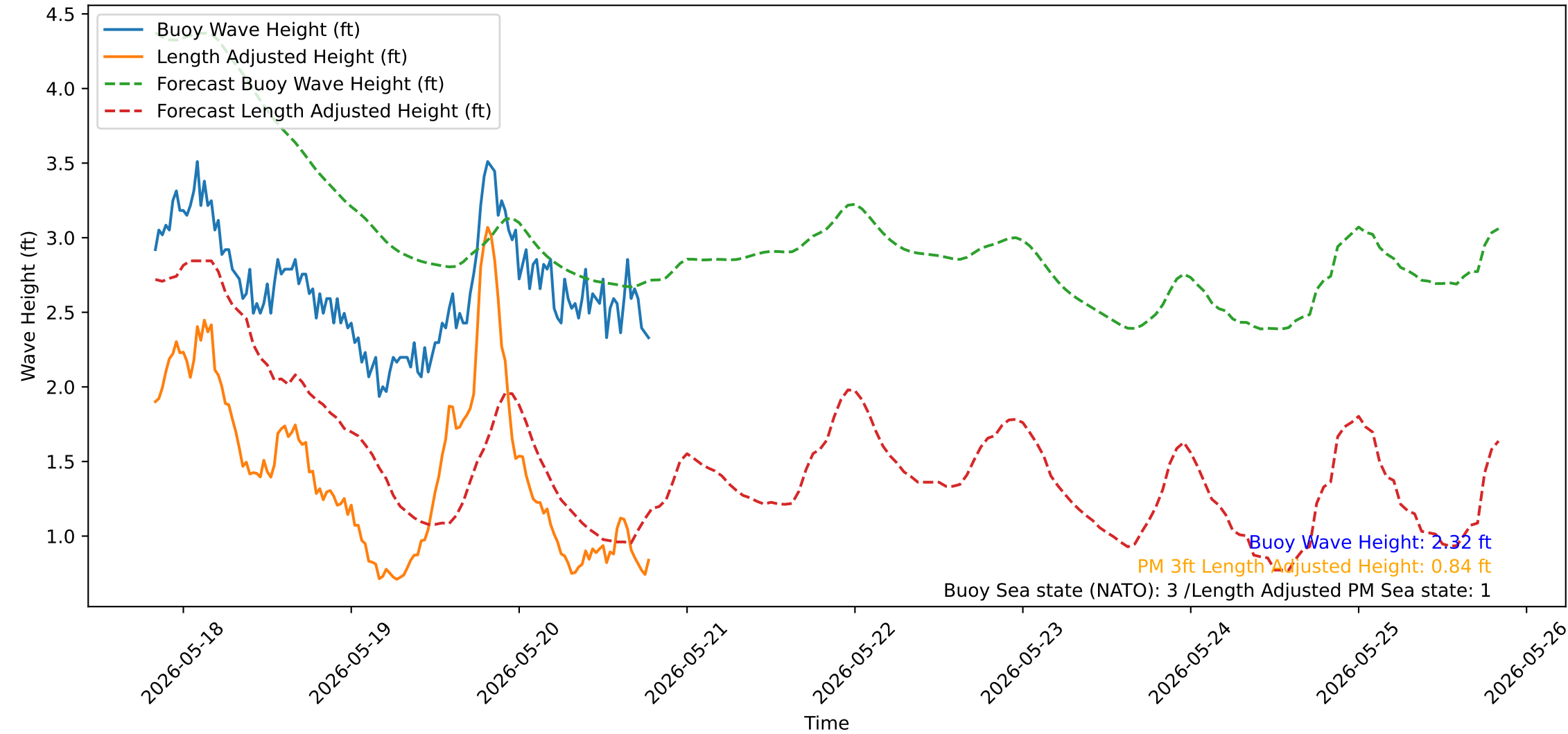
Wave Heights over Time for Red Beach at 2026-05-20 19:30:51
