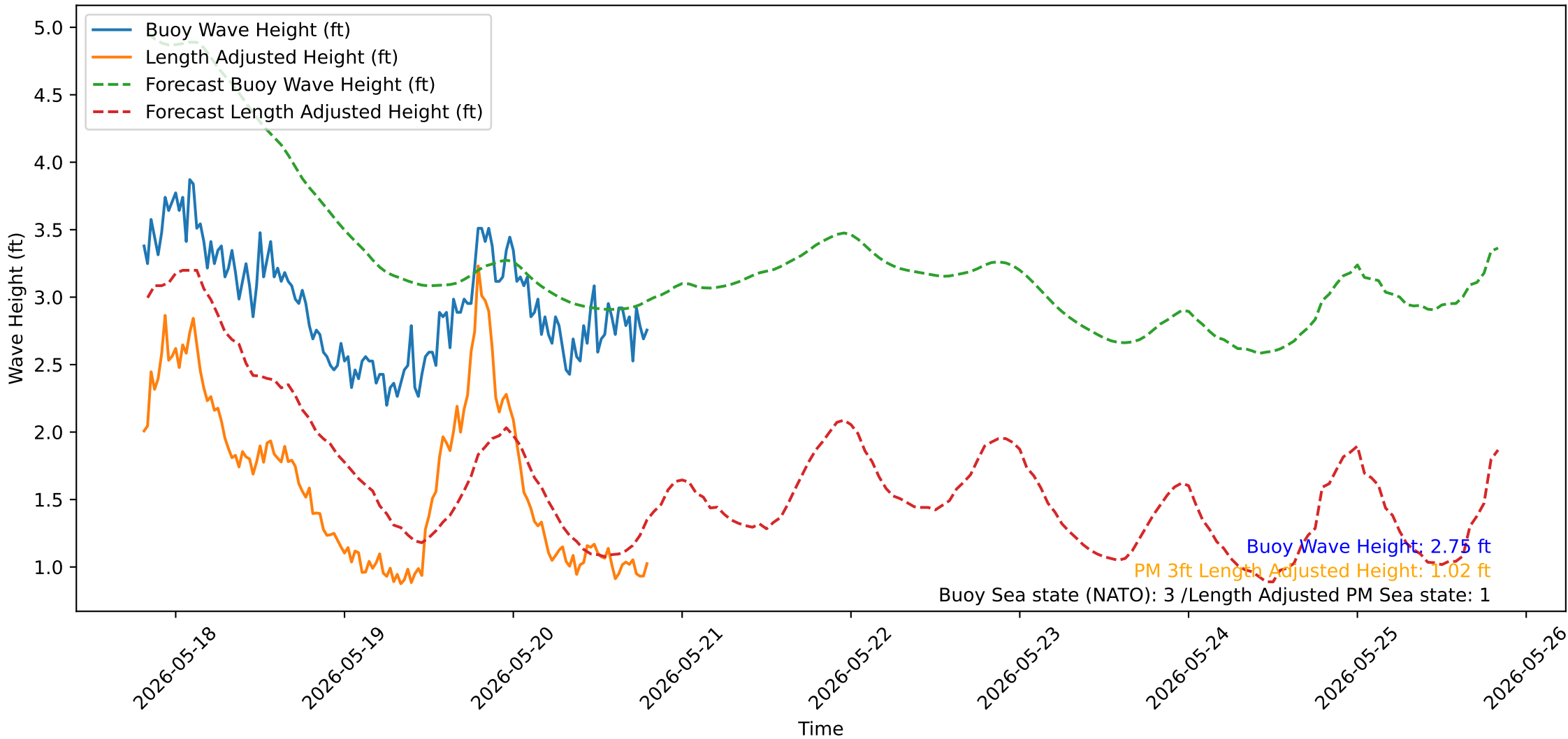
Wave Heights over Time for Oceanside Harbor at 2026-05-20 19:30:31
