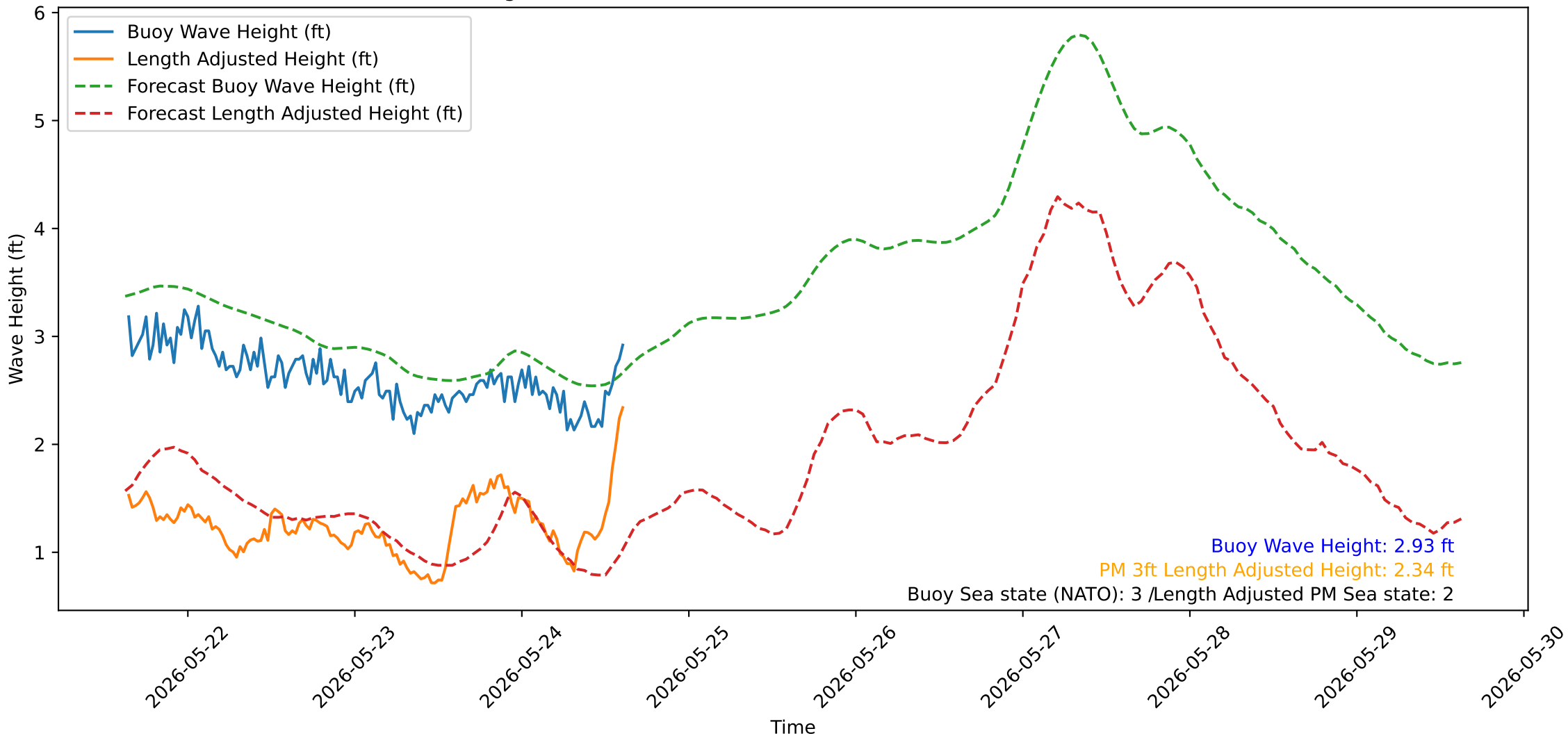
Wave Heights over Time for Oceanside Harbor at 2026-05-24 15:20:31
