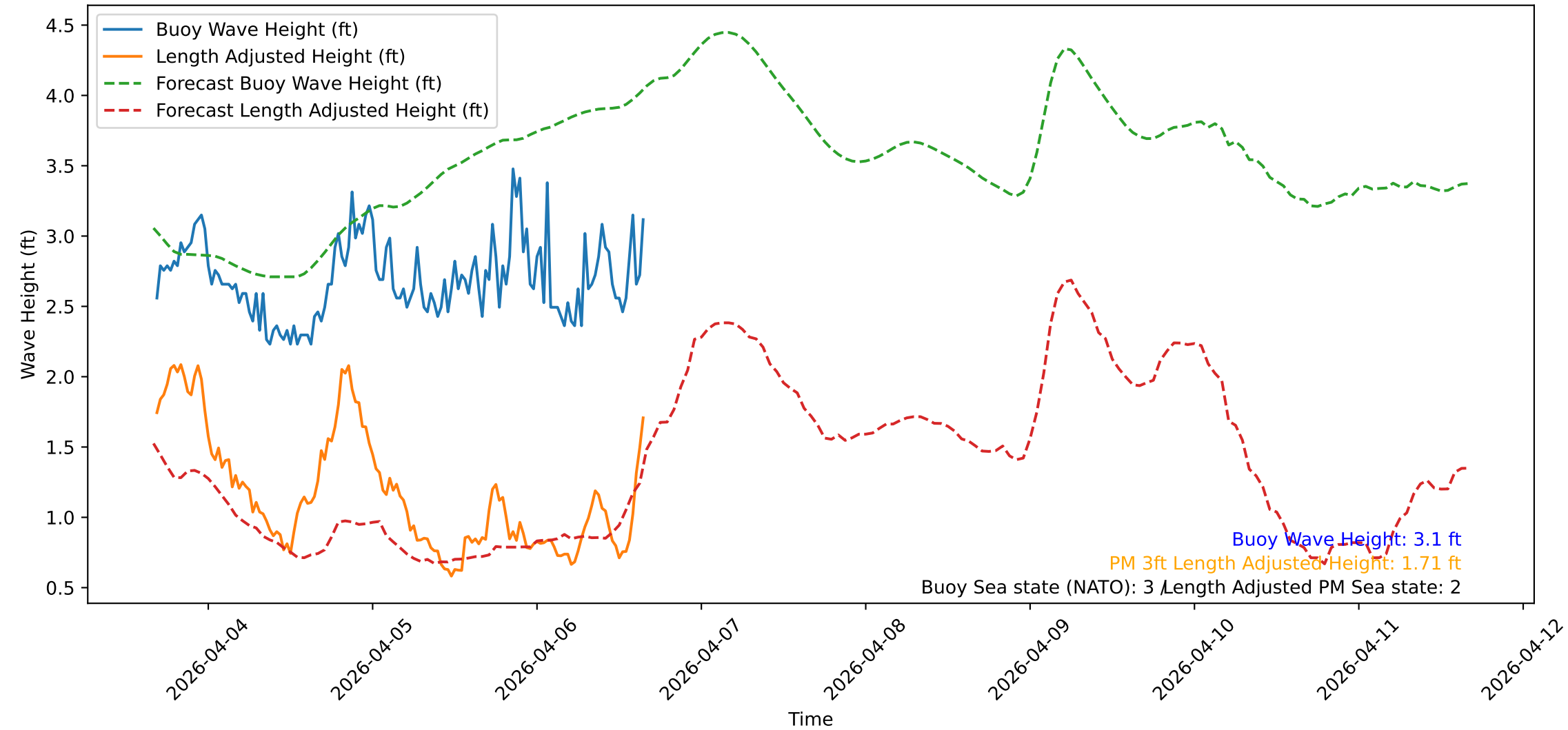
Wave Heights over Time for Green Beach at 2026-04-06 16:21:09
