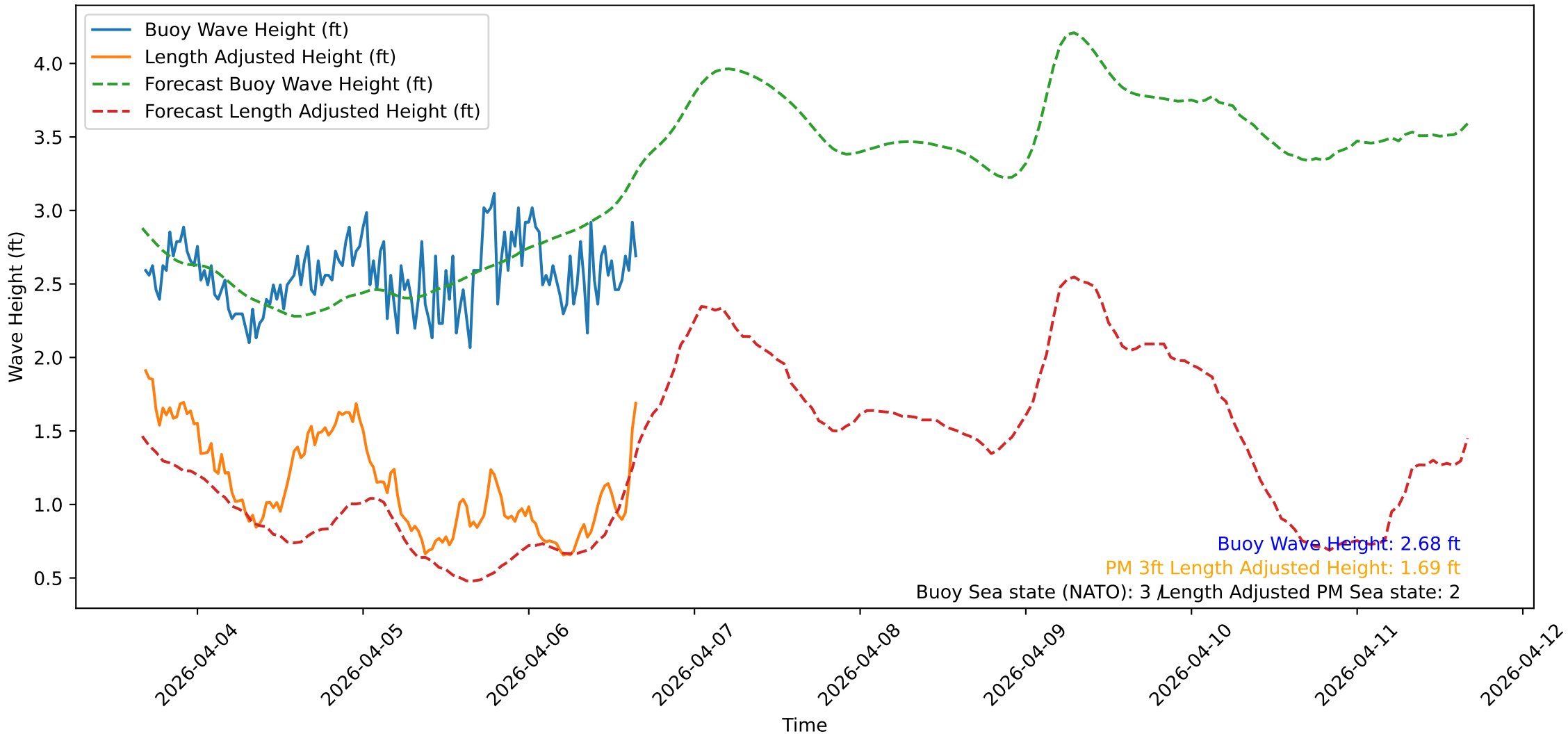
Wave Heights over Time for Oceanside Harbor at 2026-04-06 16:20:31
