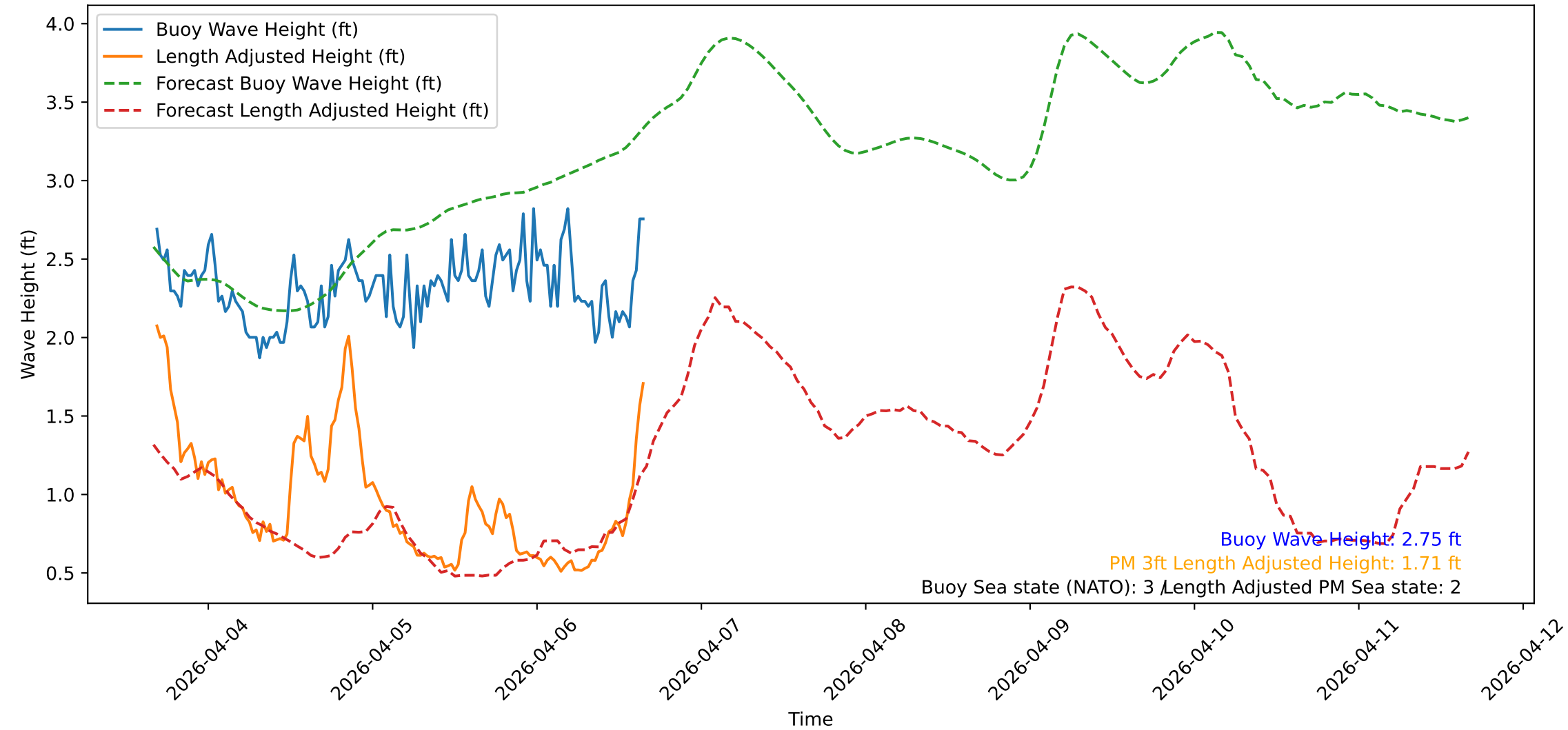
Wave Heights over Time for Red Beach at 2026-04-06 16:20:47
