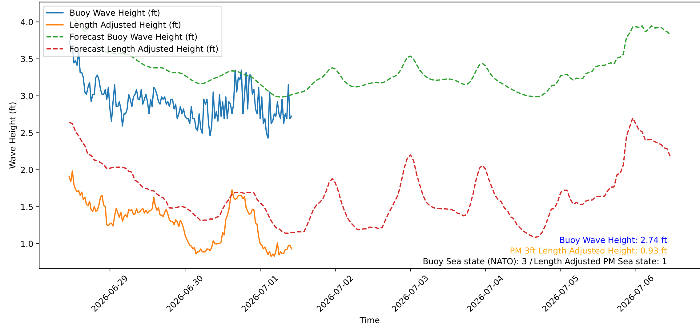
Wave Heights over Time for Red Beach at 2026-07-01 10:50:47
