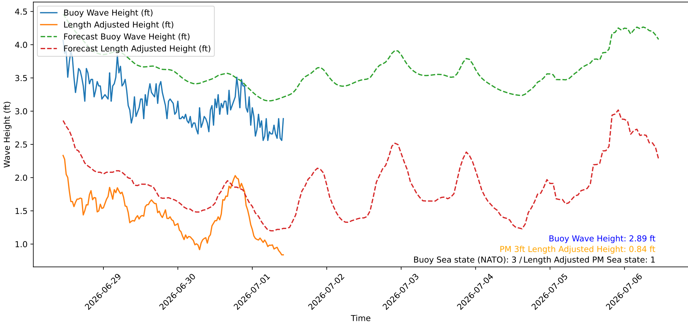
Wave Heights over Time for Green Beach at 2026-07-01 10:51:09
