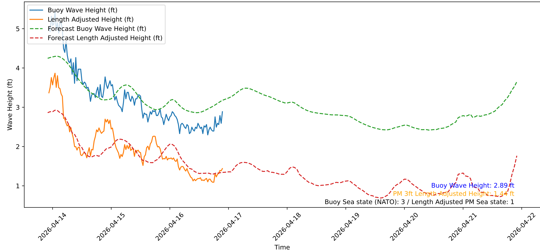
Wave Heights over Time for Oceanside Harbor at 2026-04-16 22:20:34
