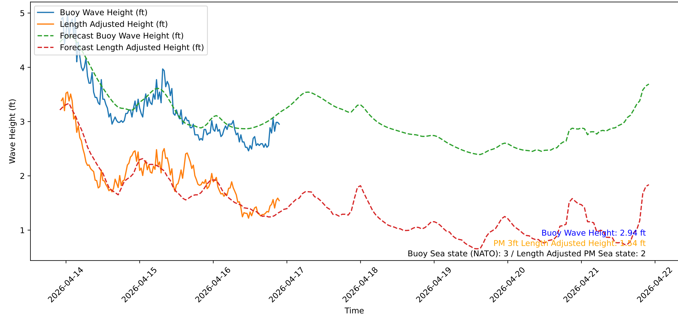
Wave Heights over Time for Green Beach at 2026-04-16 22:21:19
