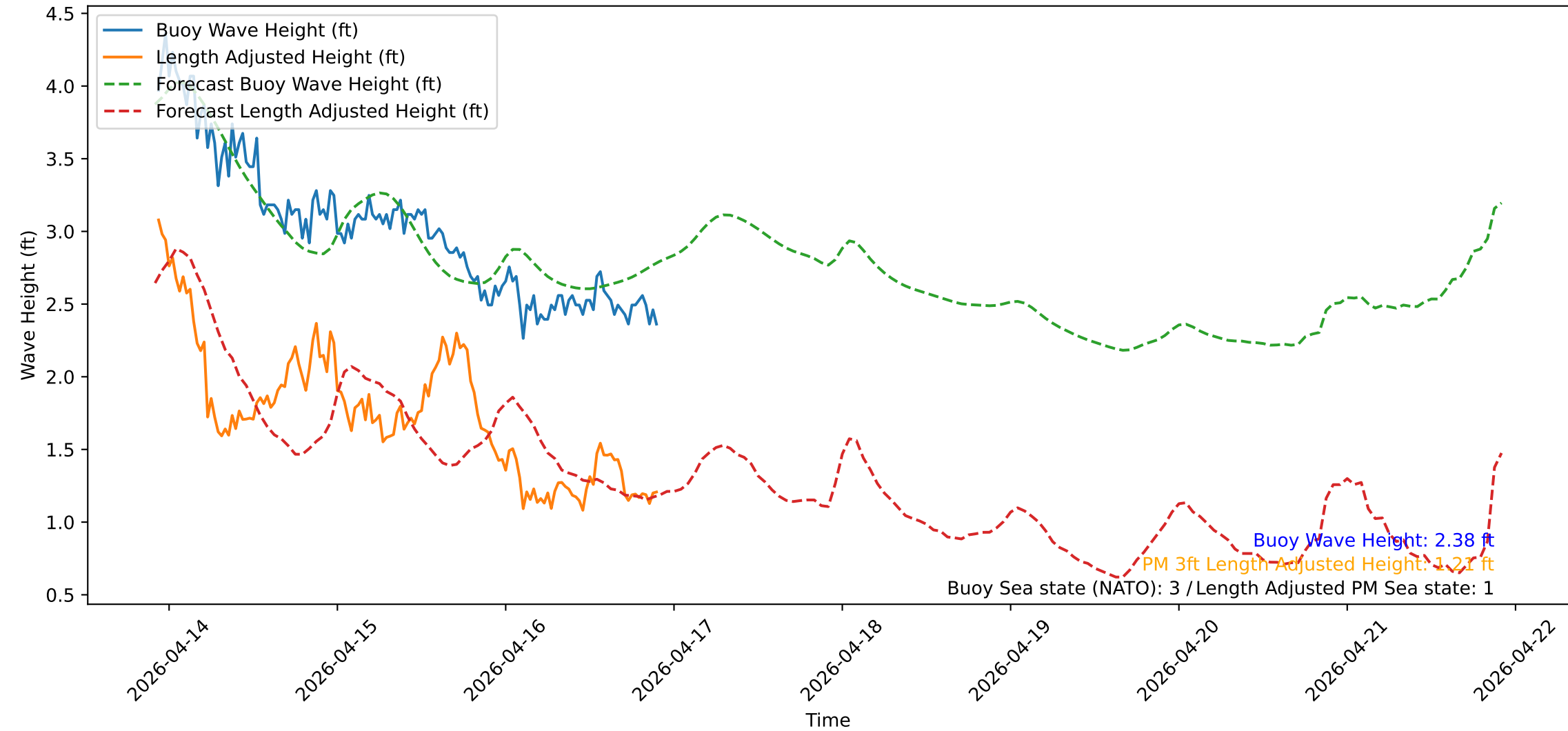
Wave Heights over Time for Red Beach at 2026-04-16 22:20:55
